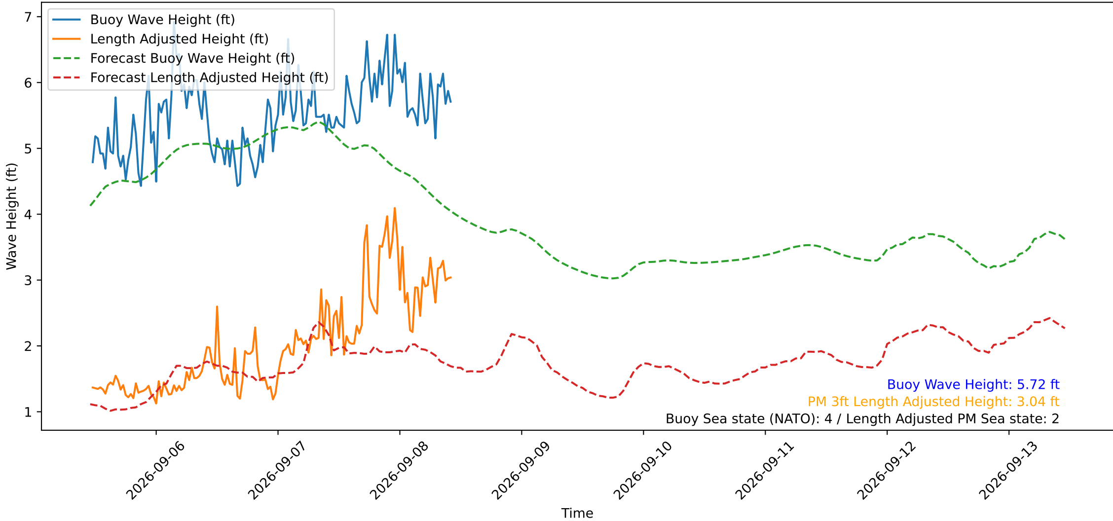
Wave Heights over Time for Red Beach at 2026-09-08 11:00:49
