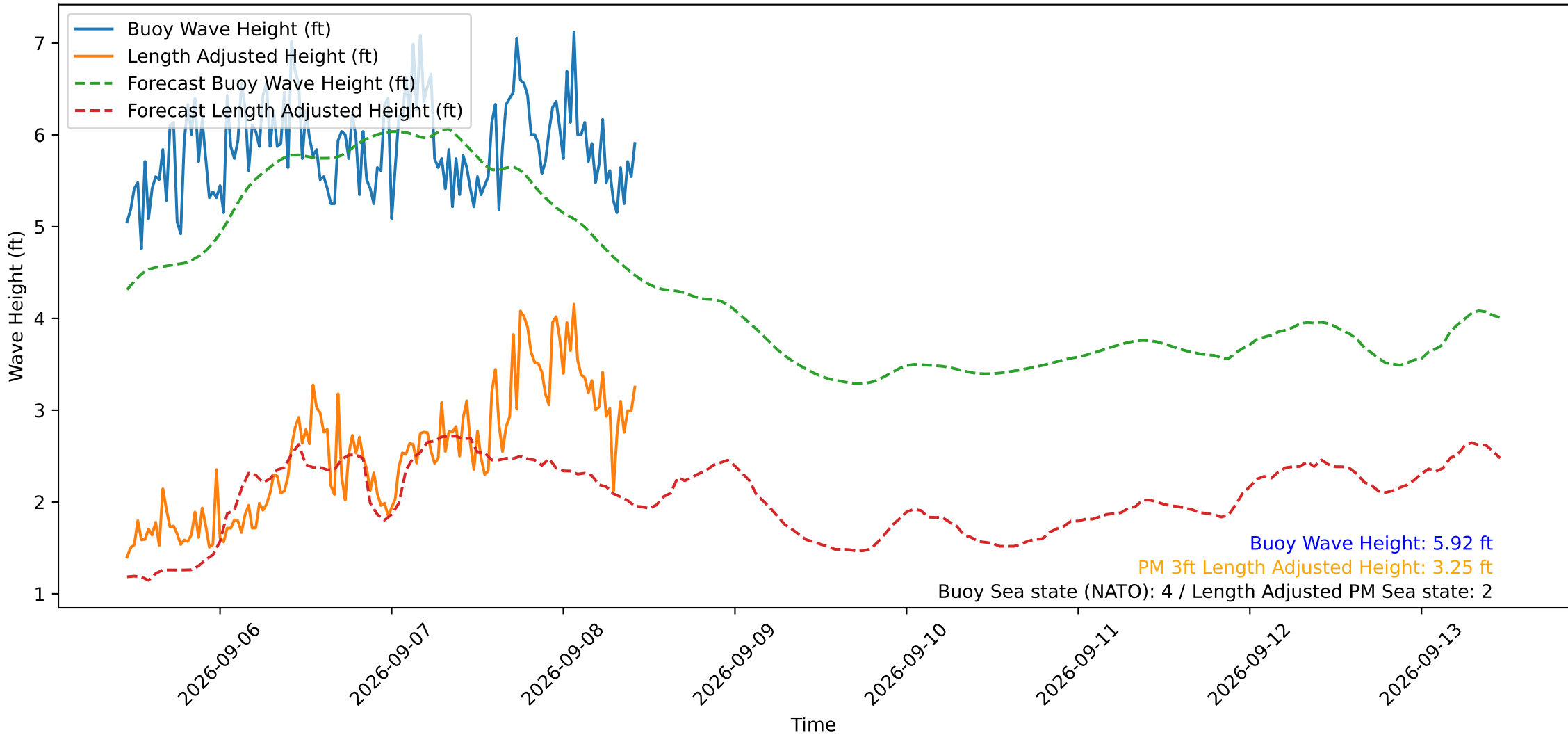
Wave Heights over Time for Oceanside Harbor at 2026-09-08 11:00:30
