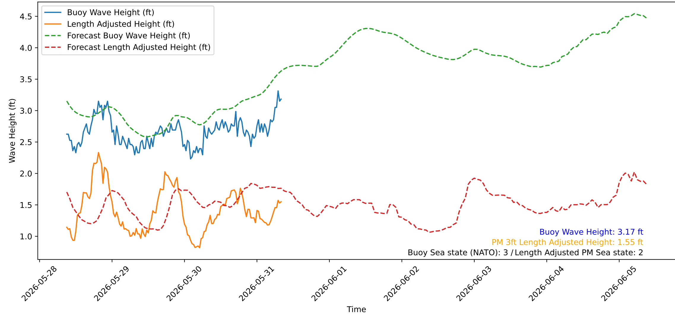
Wave Heights over Time for Red Beach at 2026-05-31 08:50:46
