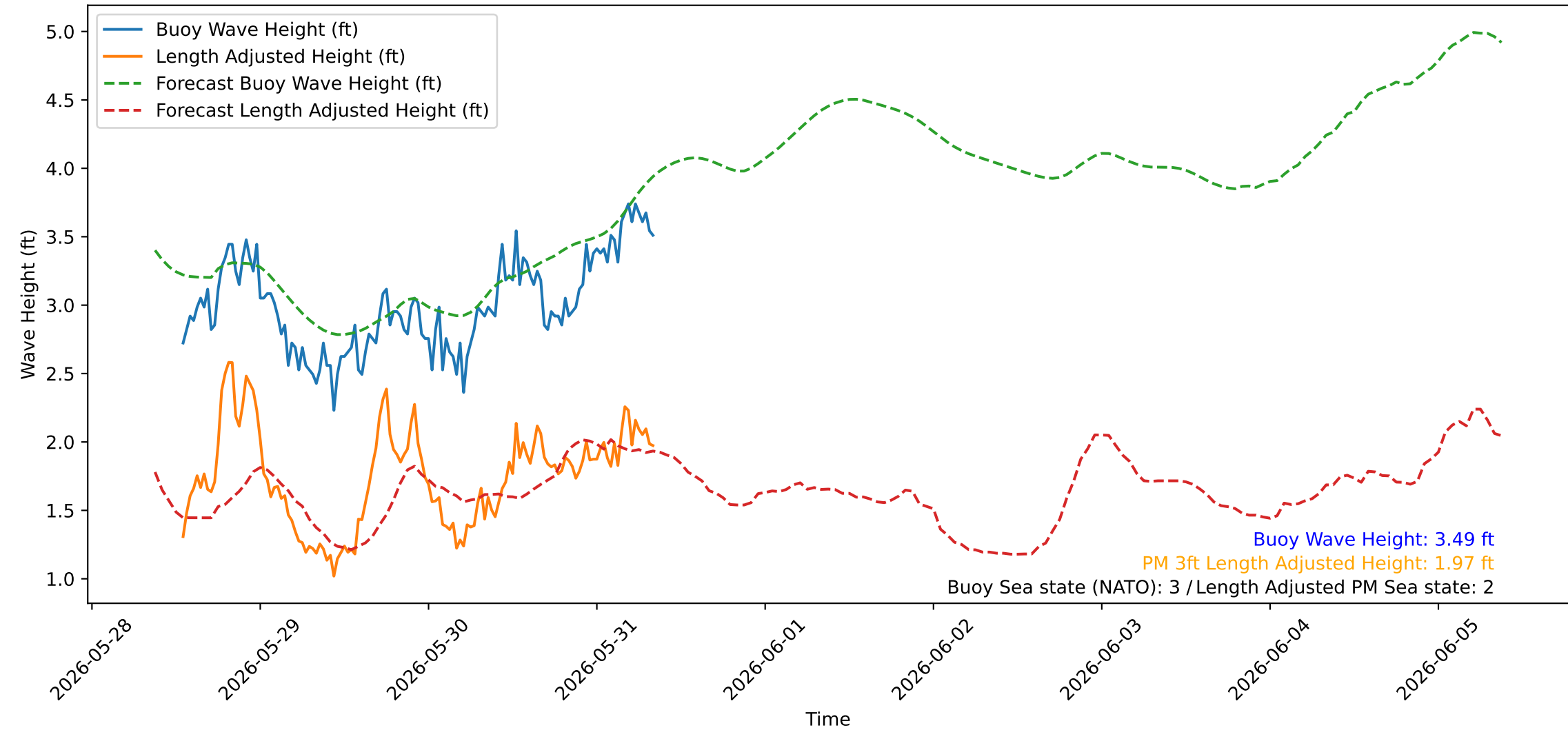
Wave Heights over Time for Oceanside Harbor at 2026-05-31 08:50:25
