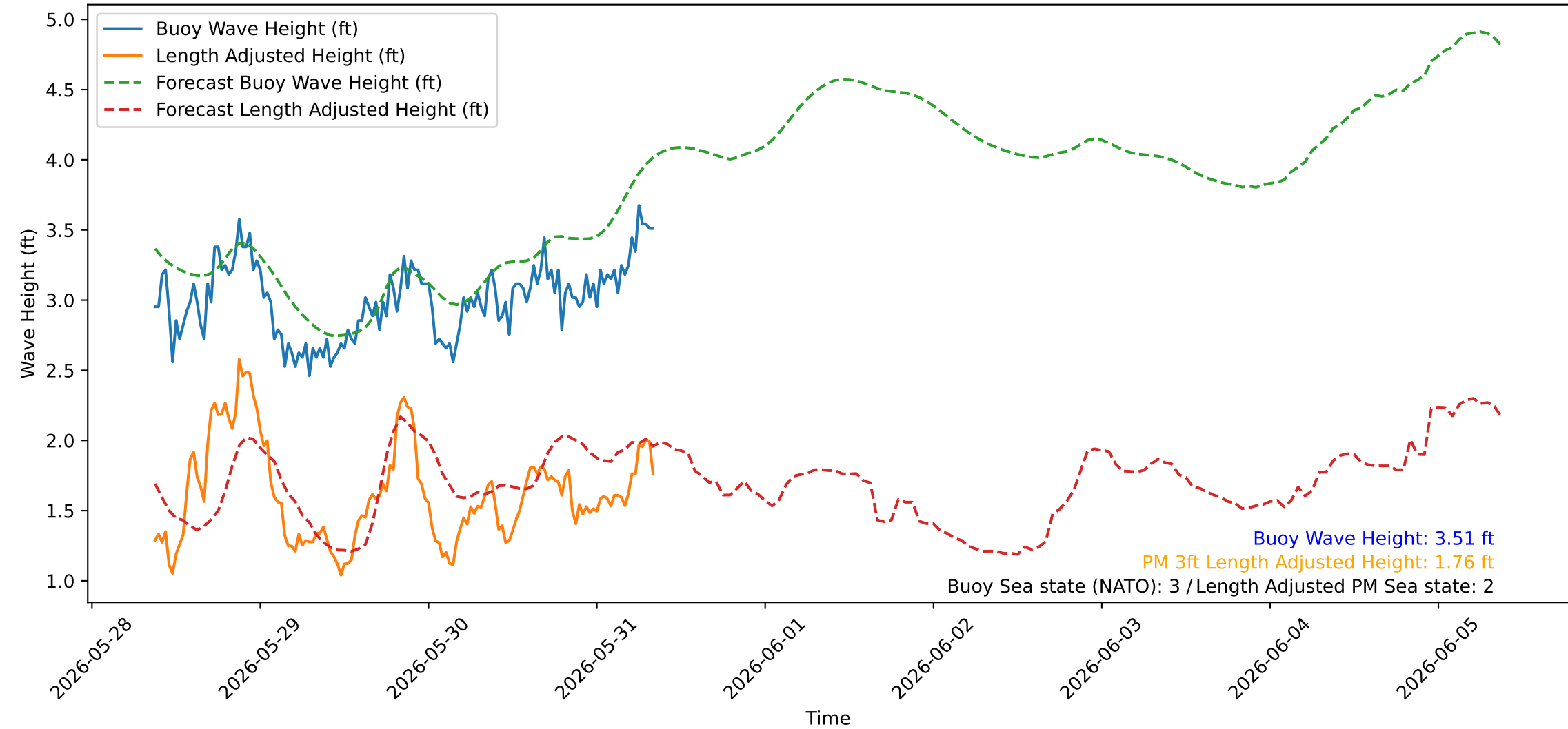
Wave Heights over Time for Green Beach at 2026-05-31 08:51:08
