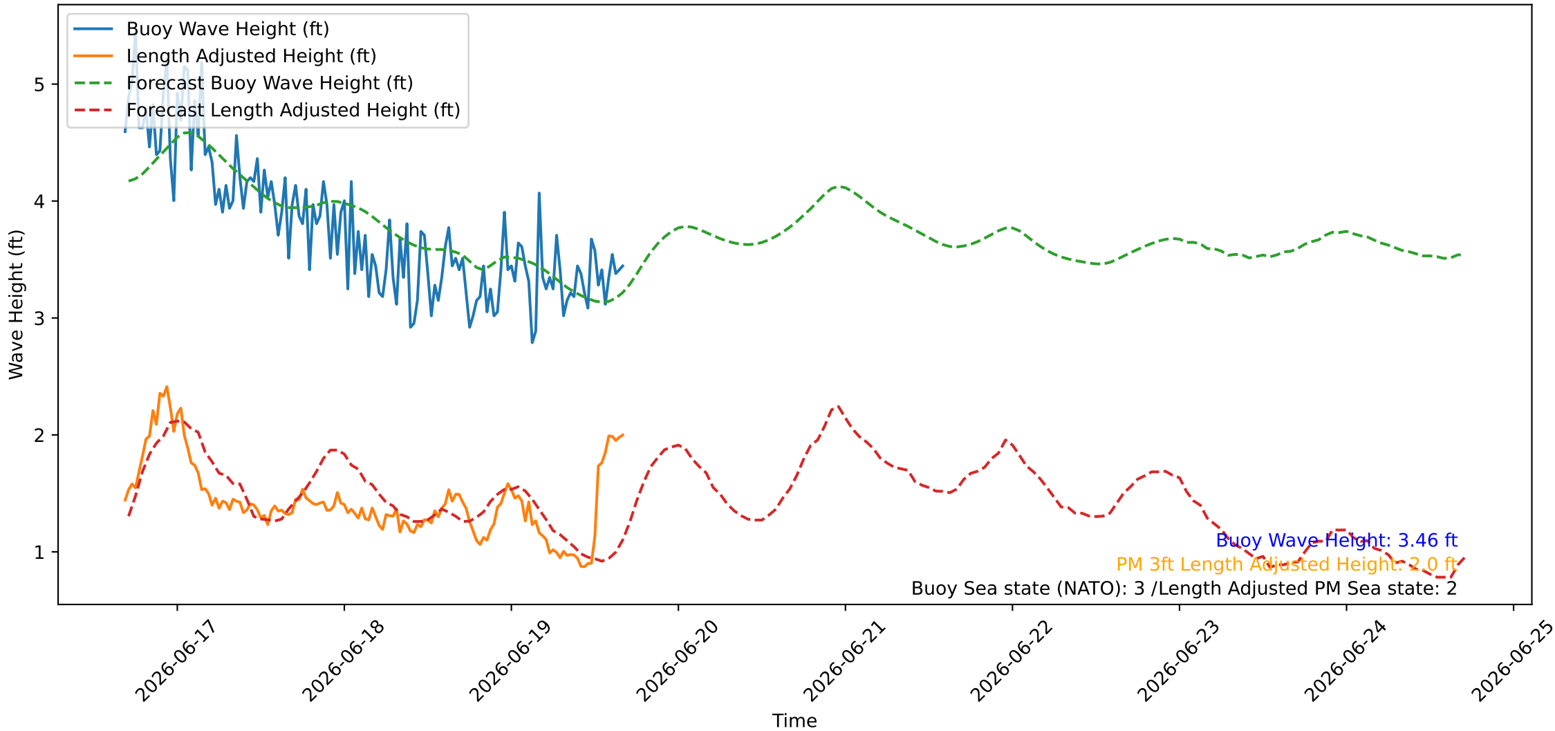
Wave Heights over Time for Oceanside Harbor at 2026-06-19 16:30:27
