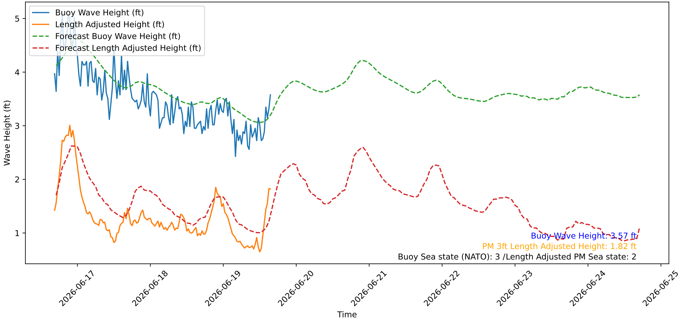
Wave Heights over Time for Green Beach at 2026-06-19 16:31:09
