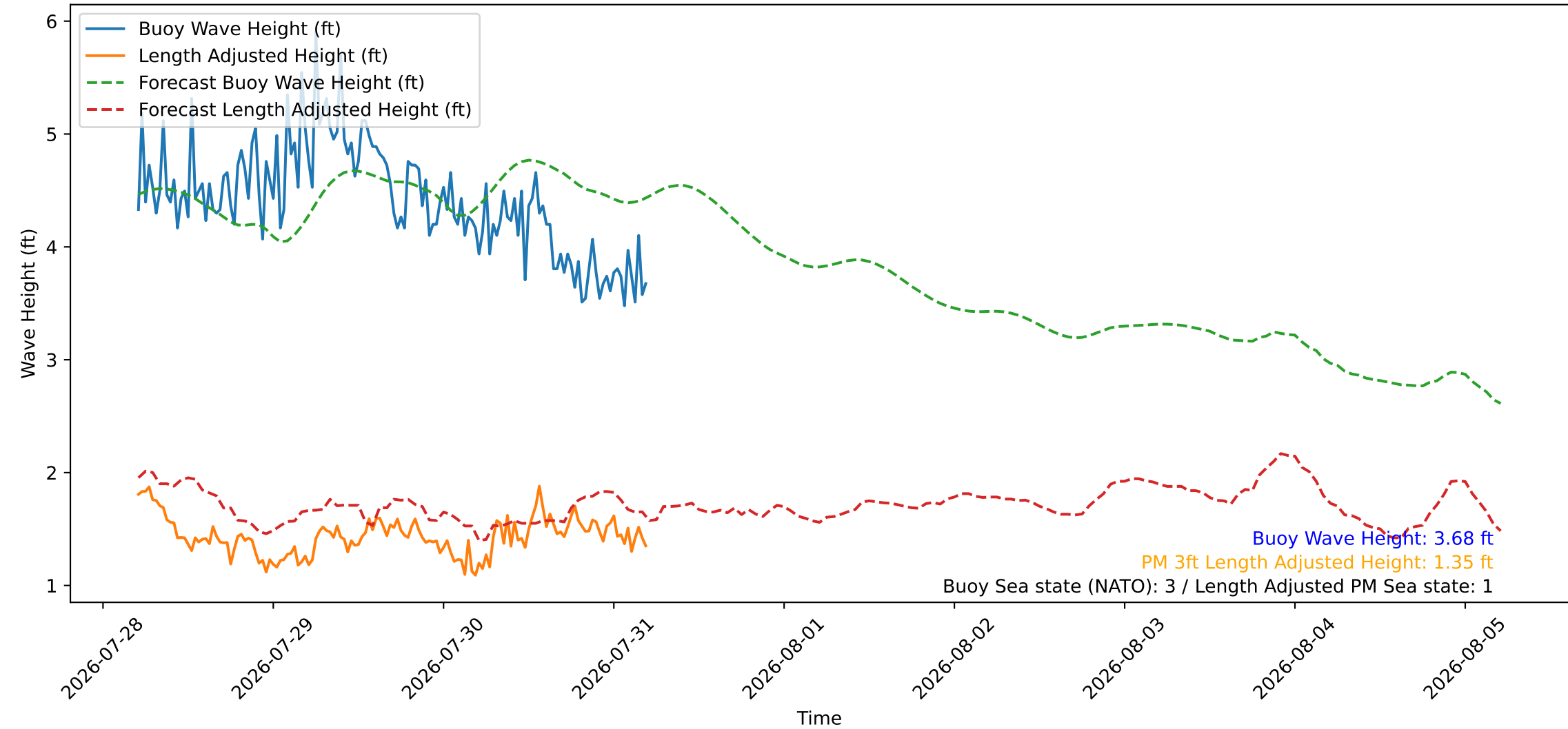
Wave Heights over Time for Oceanside Harbor at 2026-07-31 05:10:26
