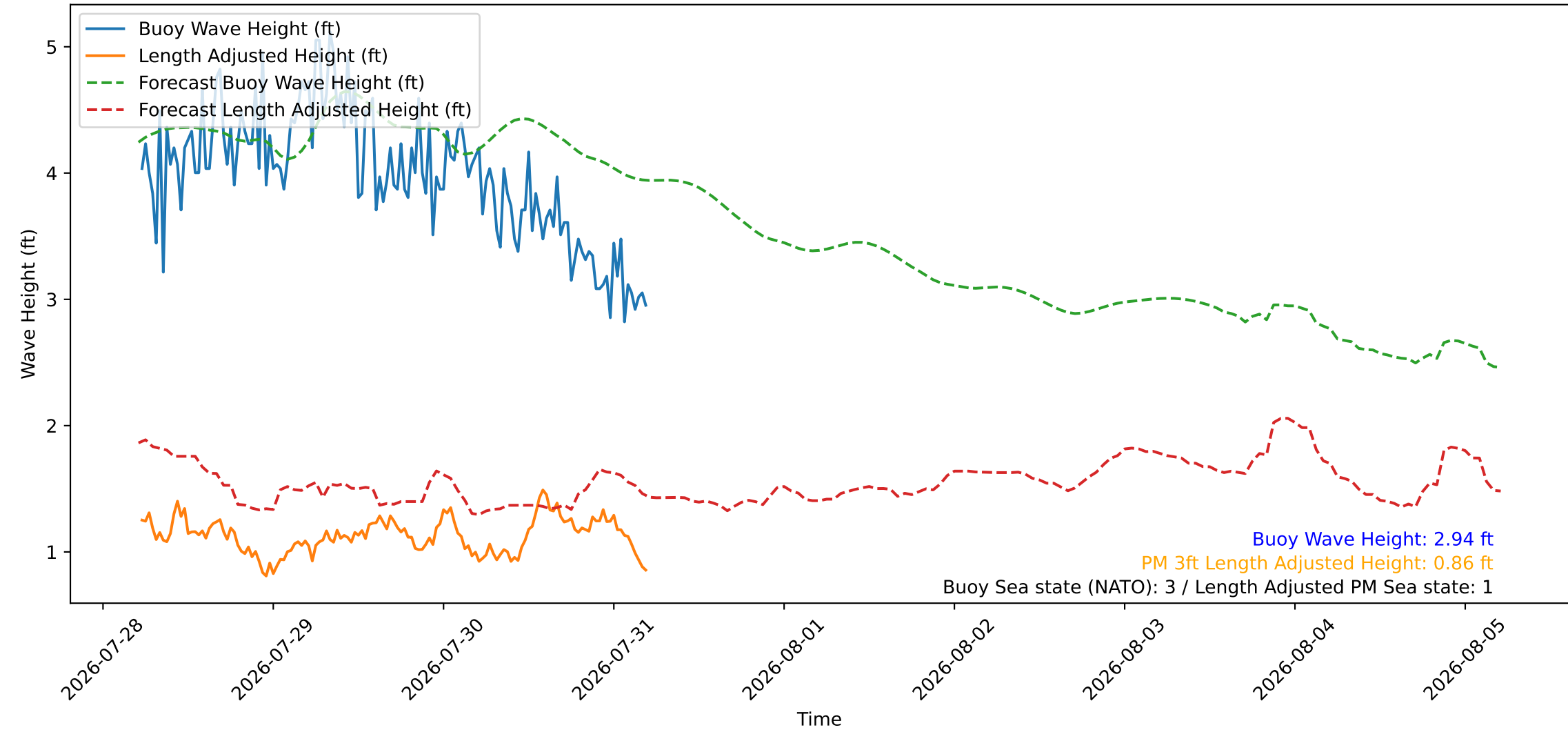
Wave Heights over Time for Red Beach at 2026-07-31 05:10:45
