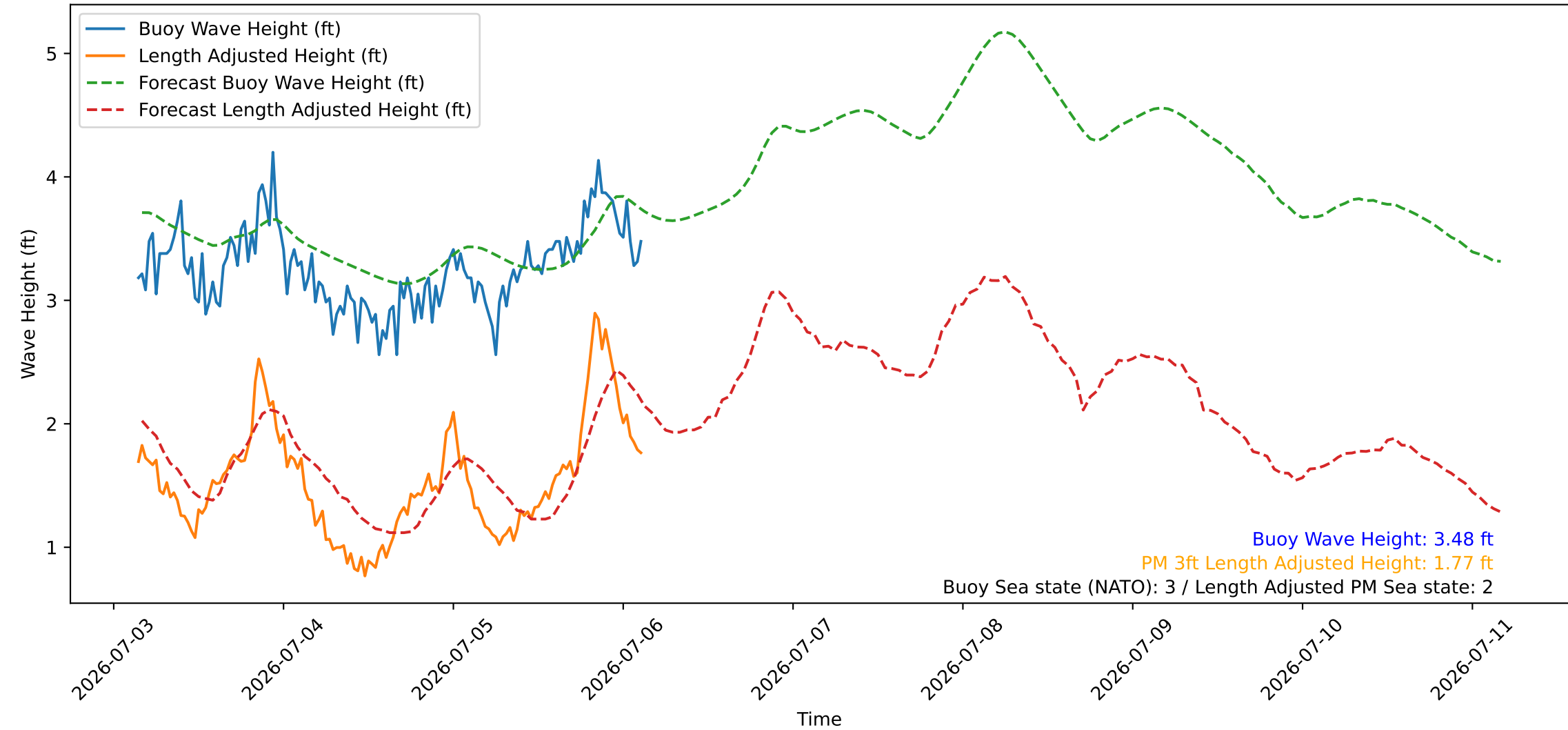
Wave Heights over Time for Green Beach at 2026-07-06 03:31:08
