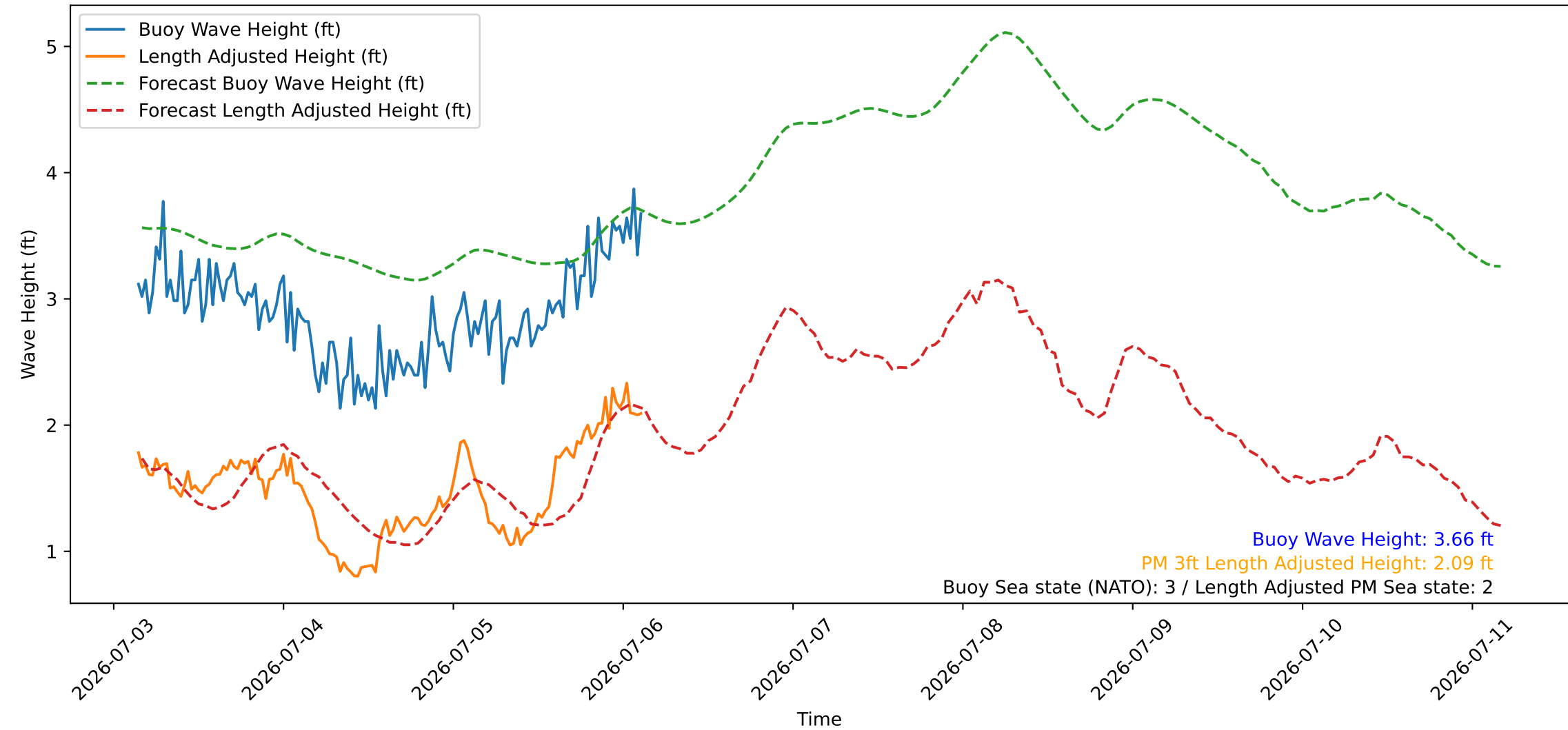
Wave Heights over Time for Oceanside Harbor at 2026-07-06 03:30:27
