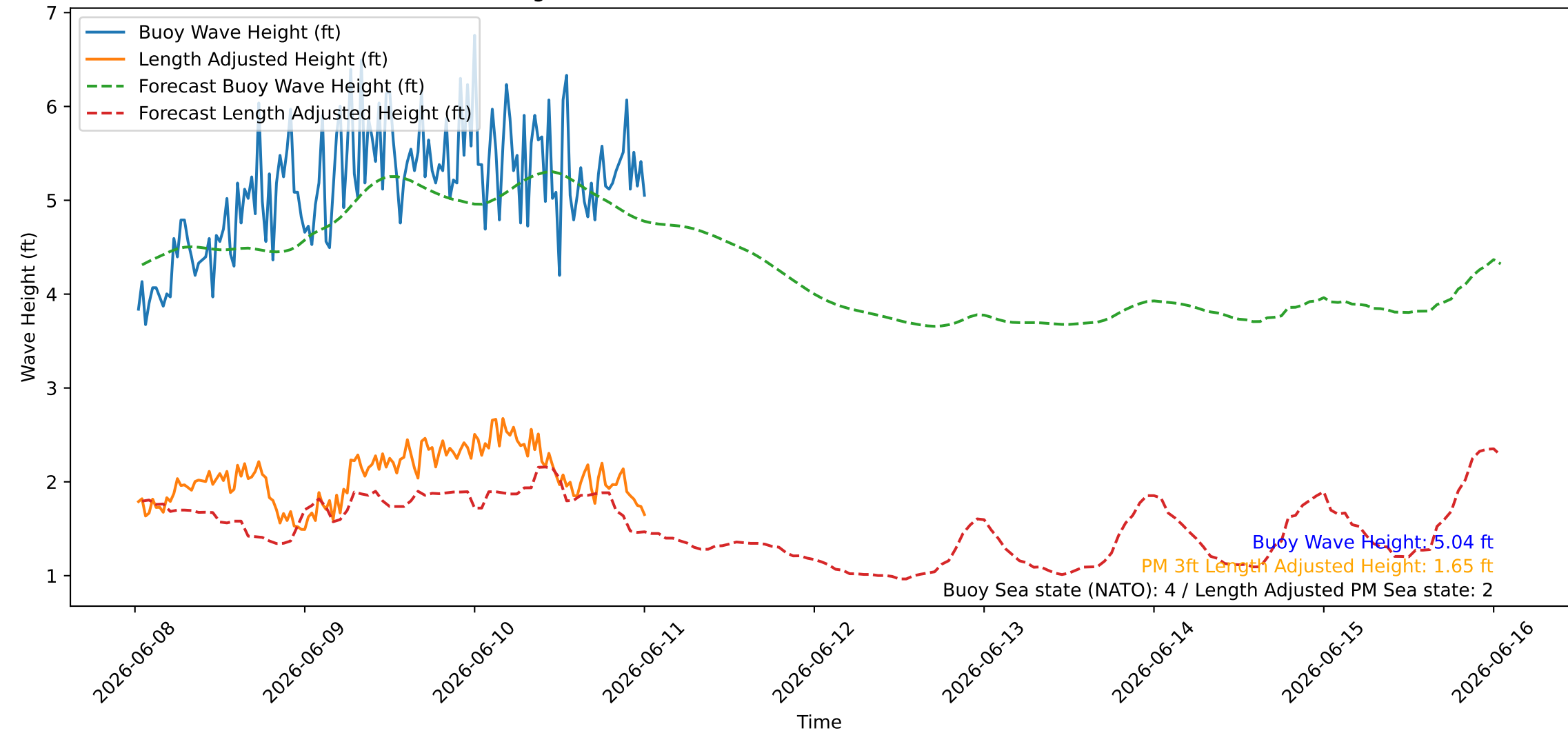
Wave Heights over Time for Oceanside Harbor at 2026-06-11 00:40:27
