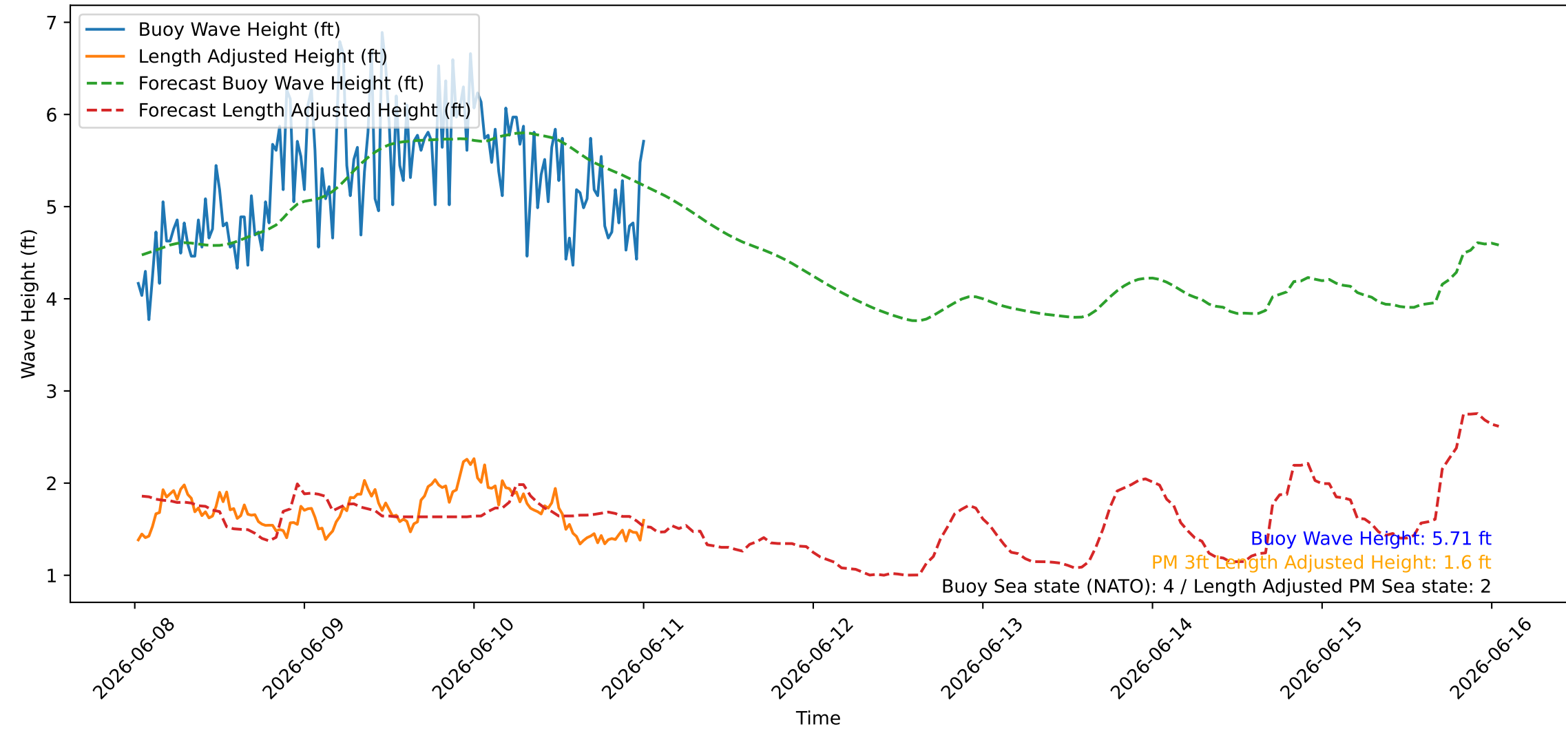
Wave Heights over Time for Green Beach at 2026-06-11 00:41:11
