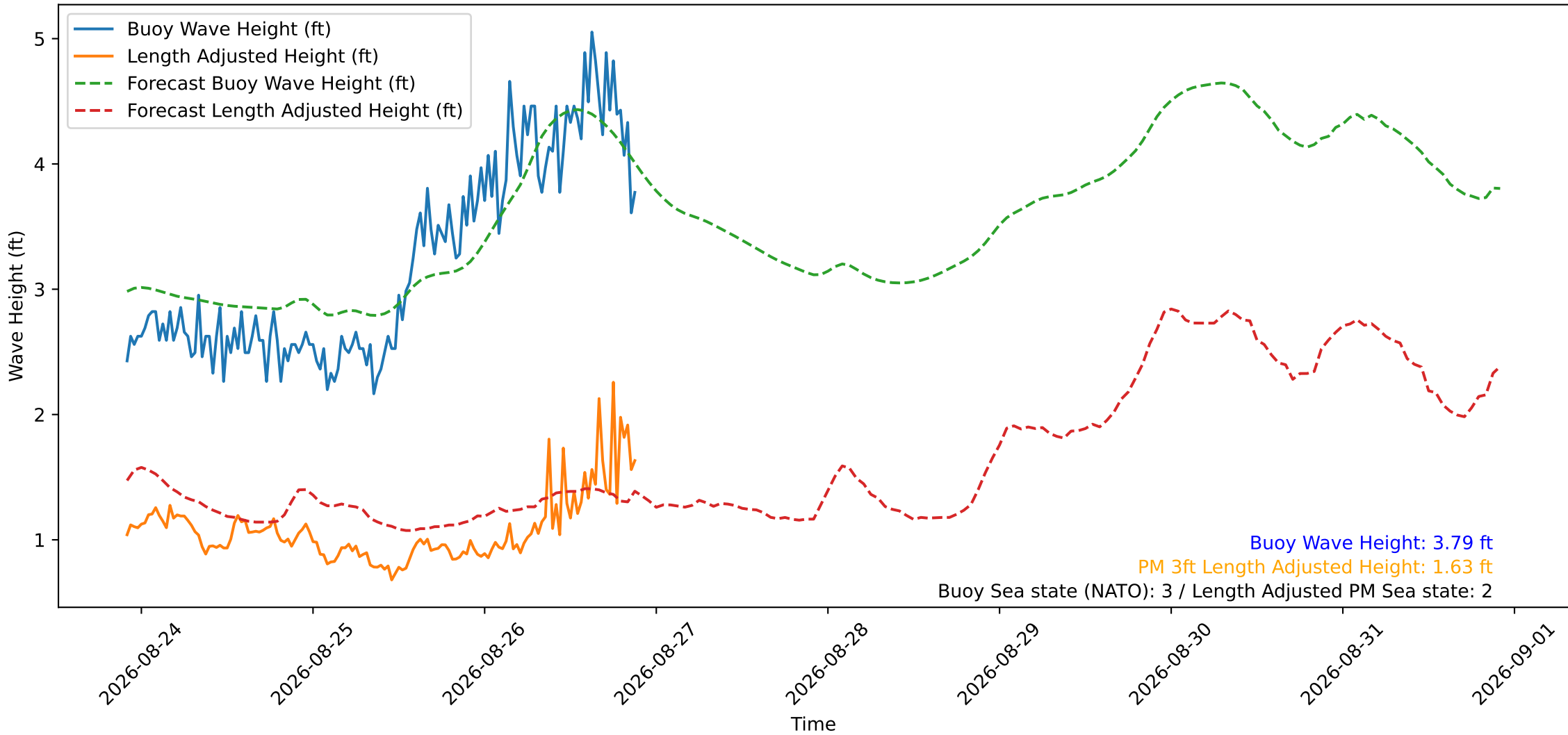
Wave Heights over Time for Red Beach at 2026-08-26 21:40:49
