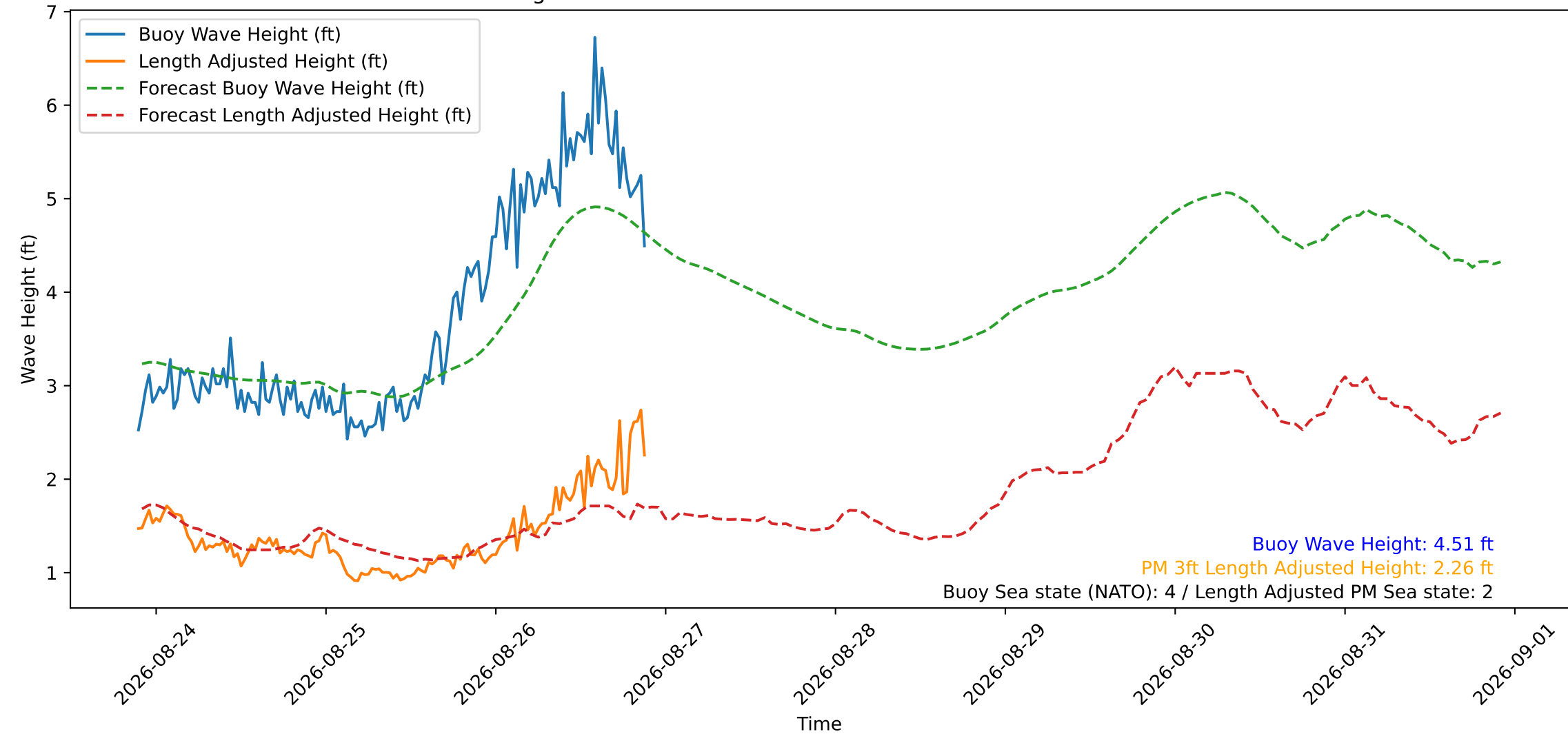
Wave Heights over Time for Oceanside Harbor at 2026-08-26 21:40:29
