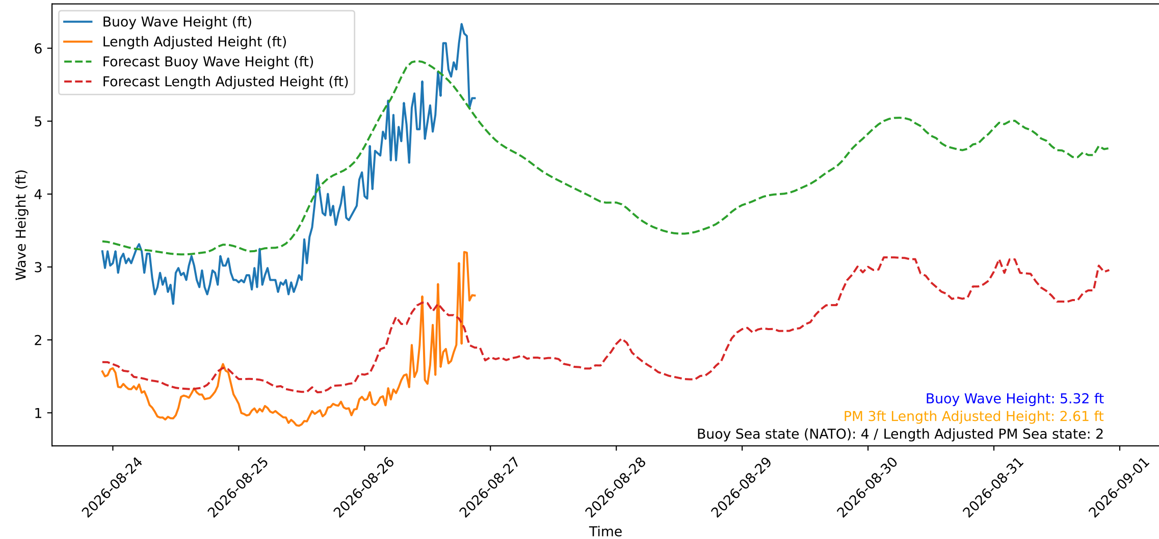
Wave Heights over Time for Green Beach at 2026-08-26 21:41:12
