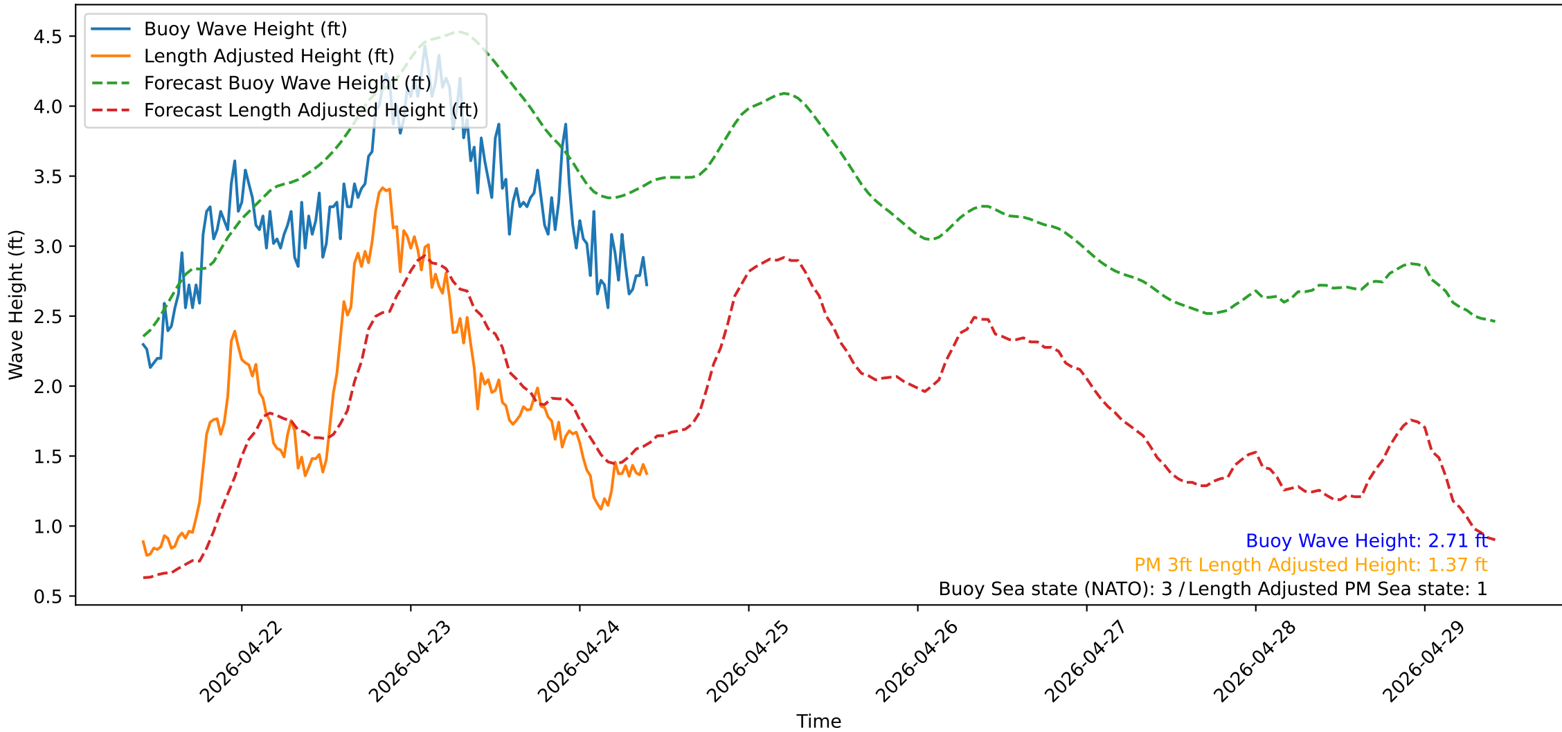
Wave Heights over Time for Oceanside Harbor at 2026-04-24 10:00:32
