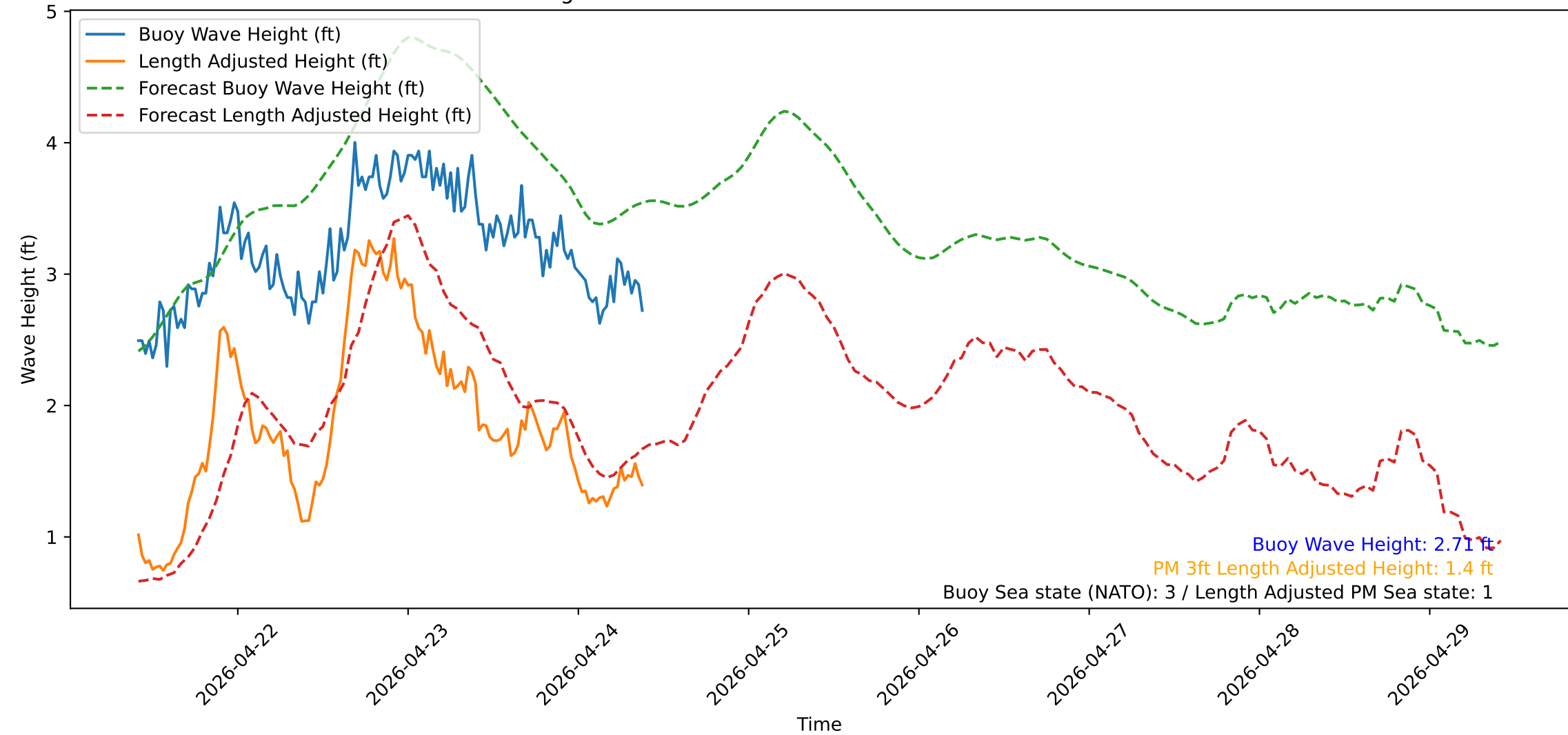
Wave Heights over Time for Green Beach at 2026-04-24 10:01:13
