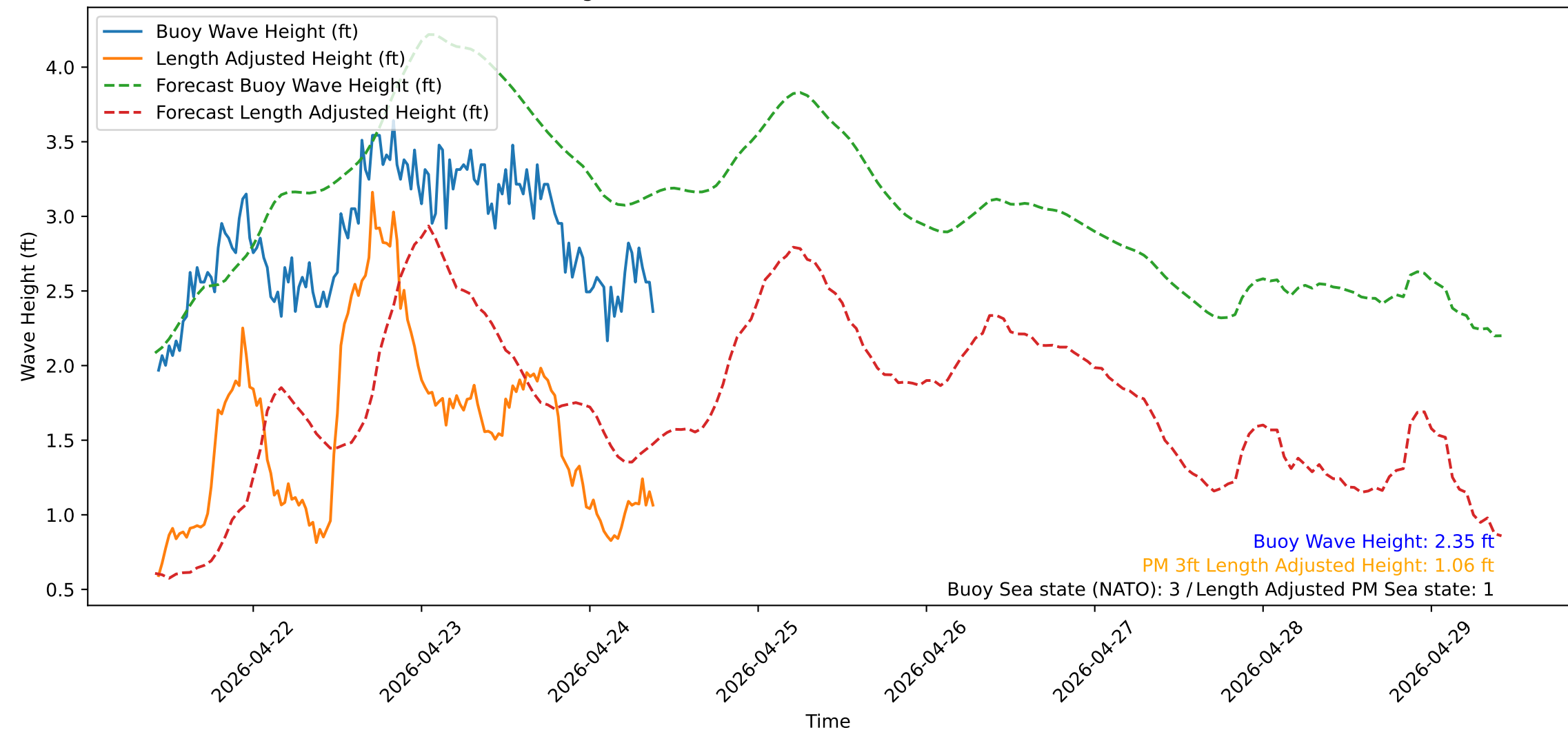
Wave Heights over Time for Red Beach at 2026-04-24 10:00:51
