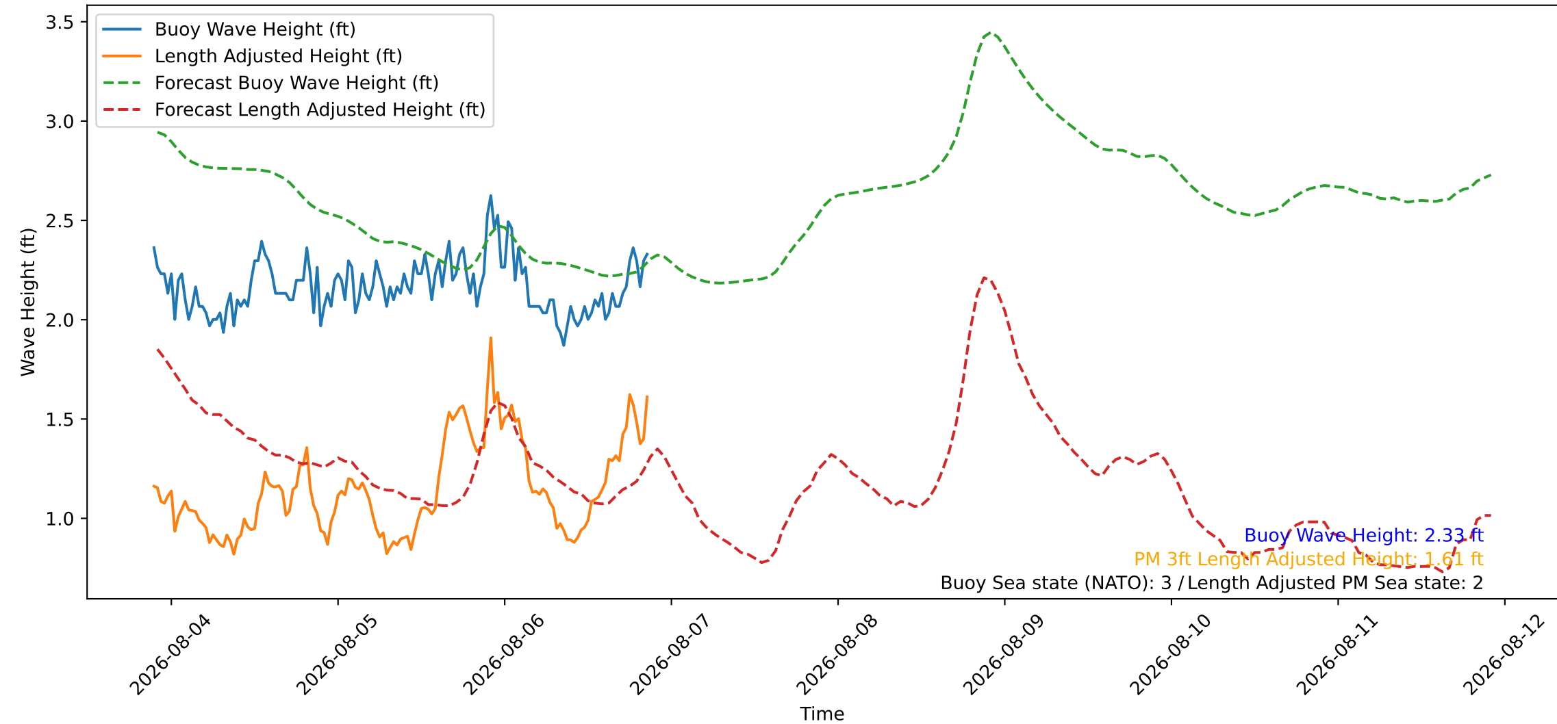
Wave Heights over Time for Green Beach at 2026-08-06 21:31:08
