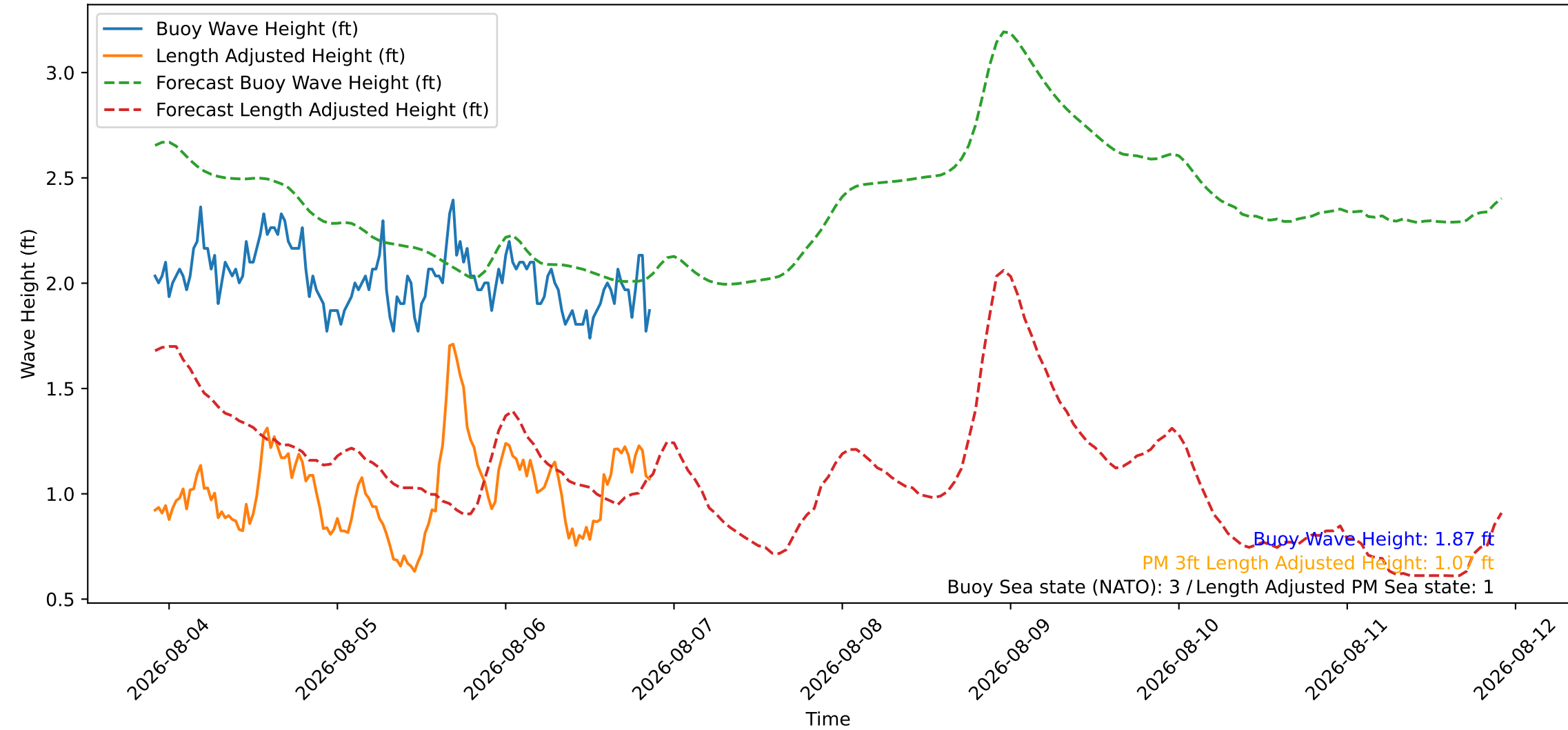
Wave Heights over Time for Red Beach at 2026-08-06 21:30:45
