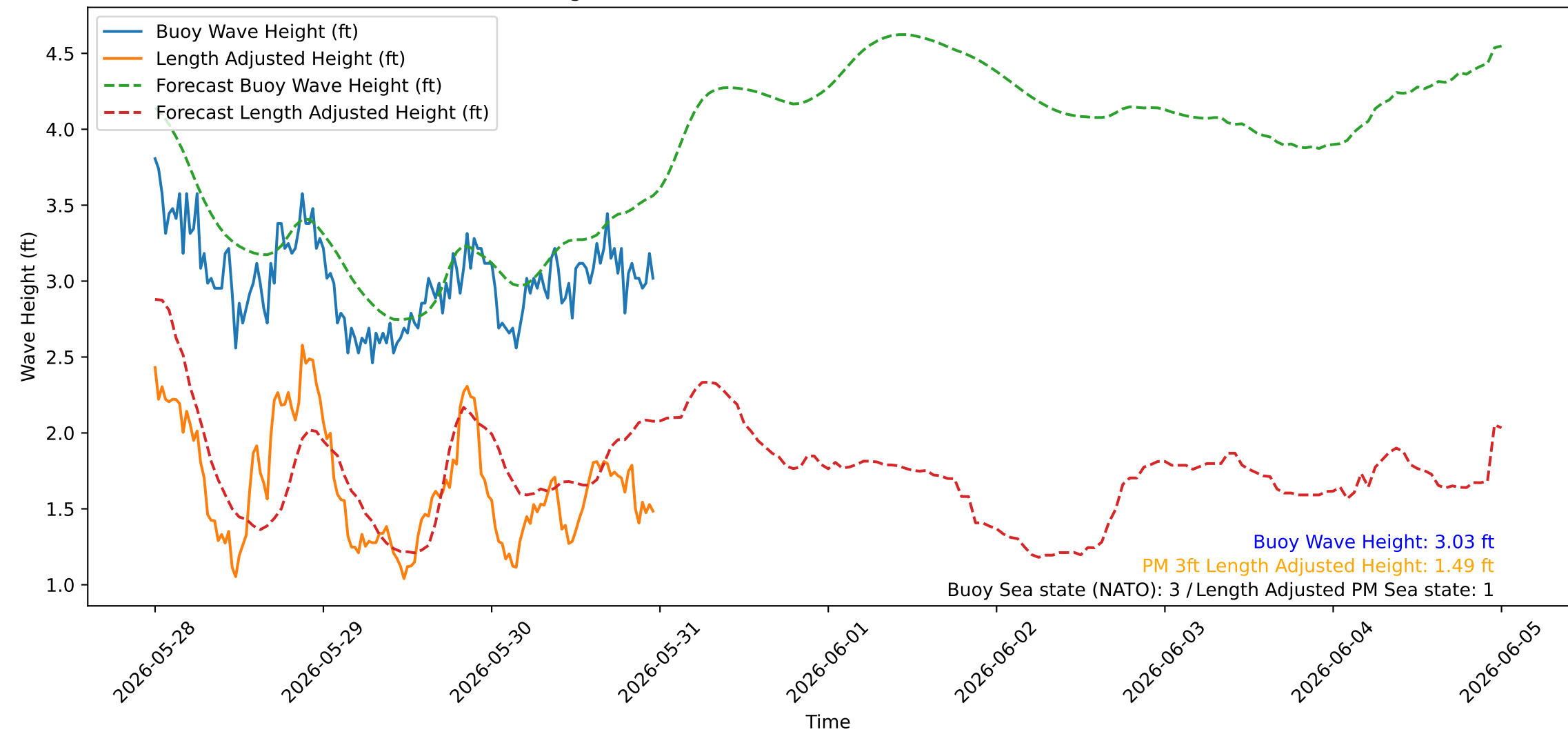
Wave Heights over Time for Green Beach at 2026-05-31 00:01:07
