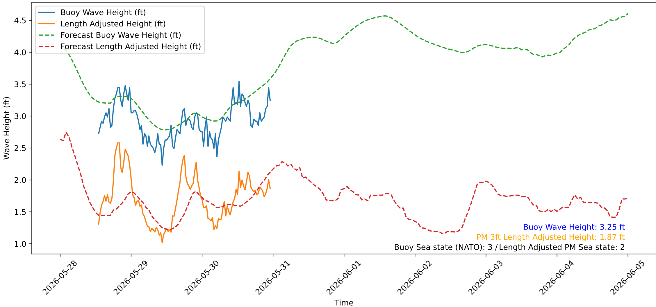
Wave Heights over Time for Oceanside Harbor at 2026-05-31 00:00:25
