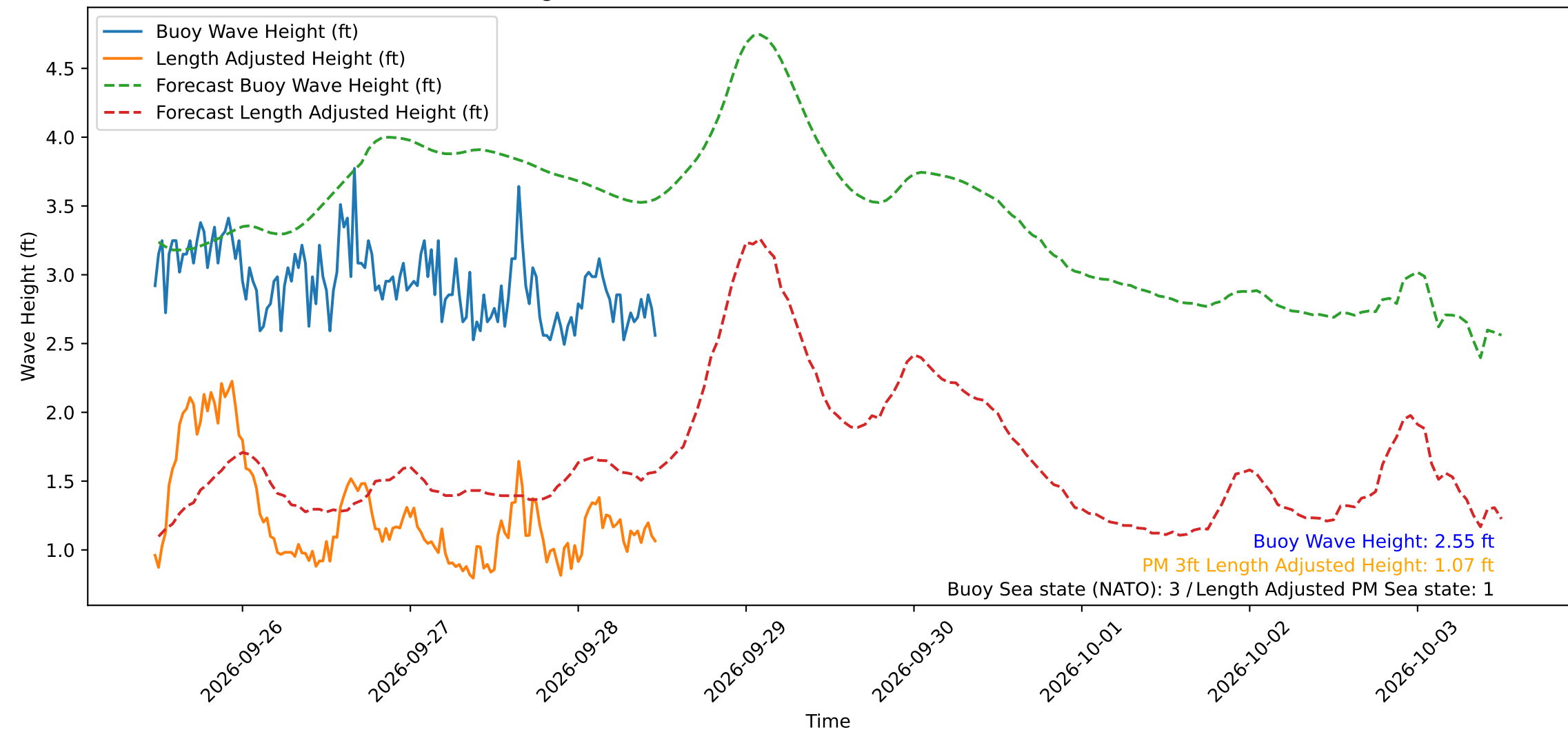
Wave Heights over Time for Oceanside Harbor at 2026-09-28 11:40:30
