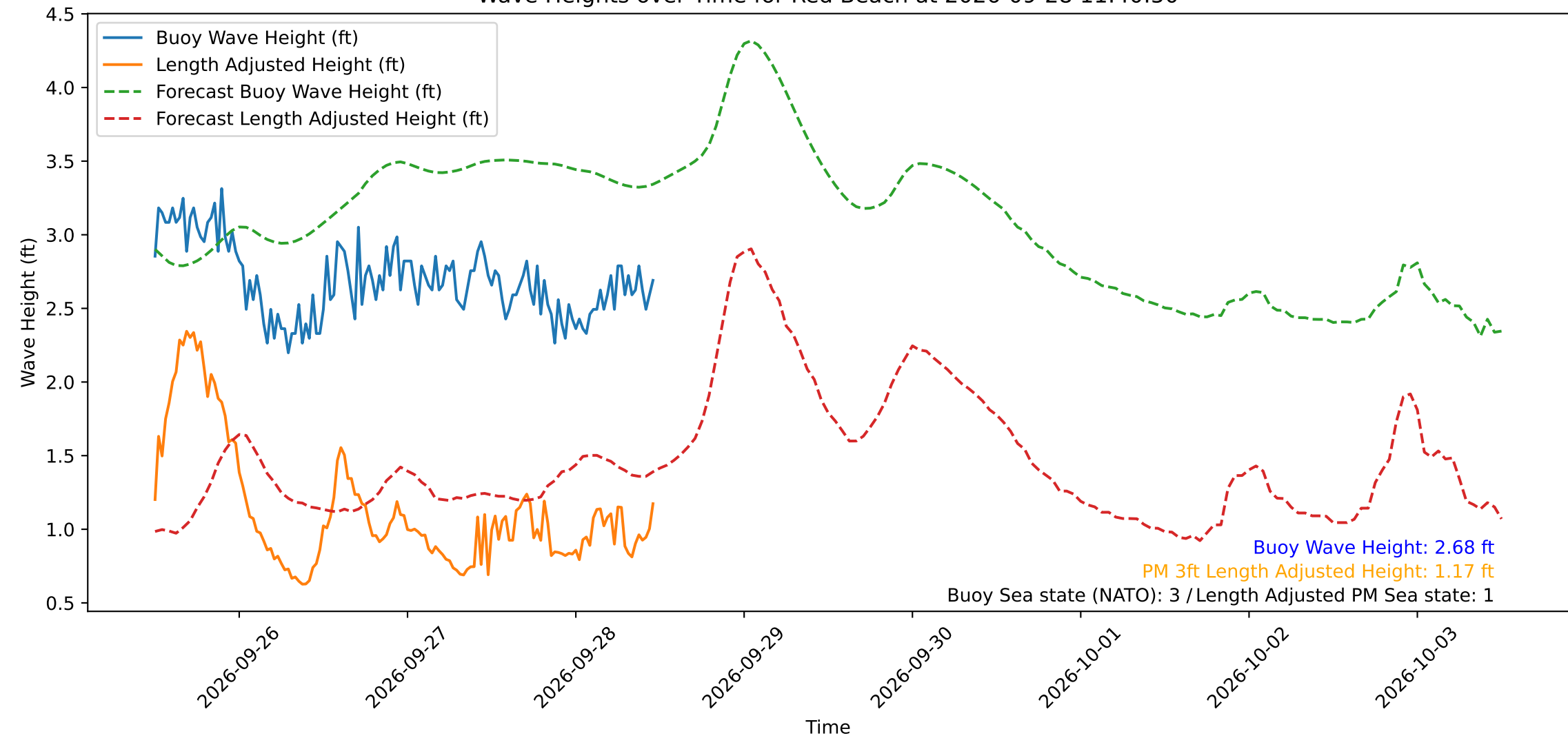
Wave Heights over Time for Red Beach at 2026-09-28 11:40:50
