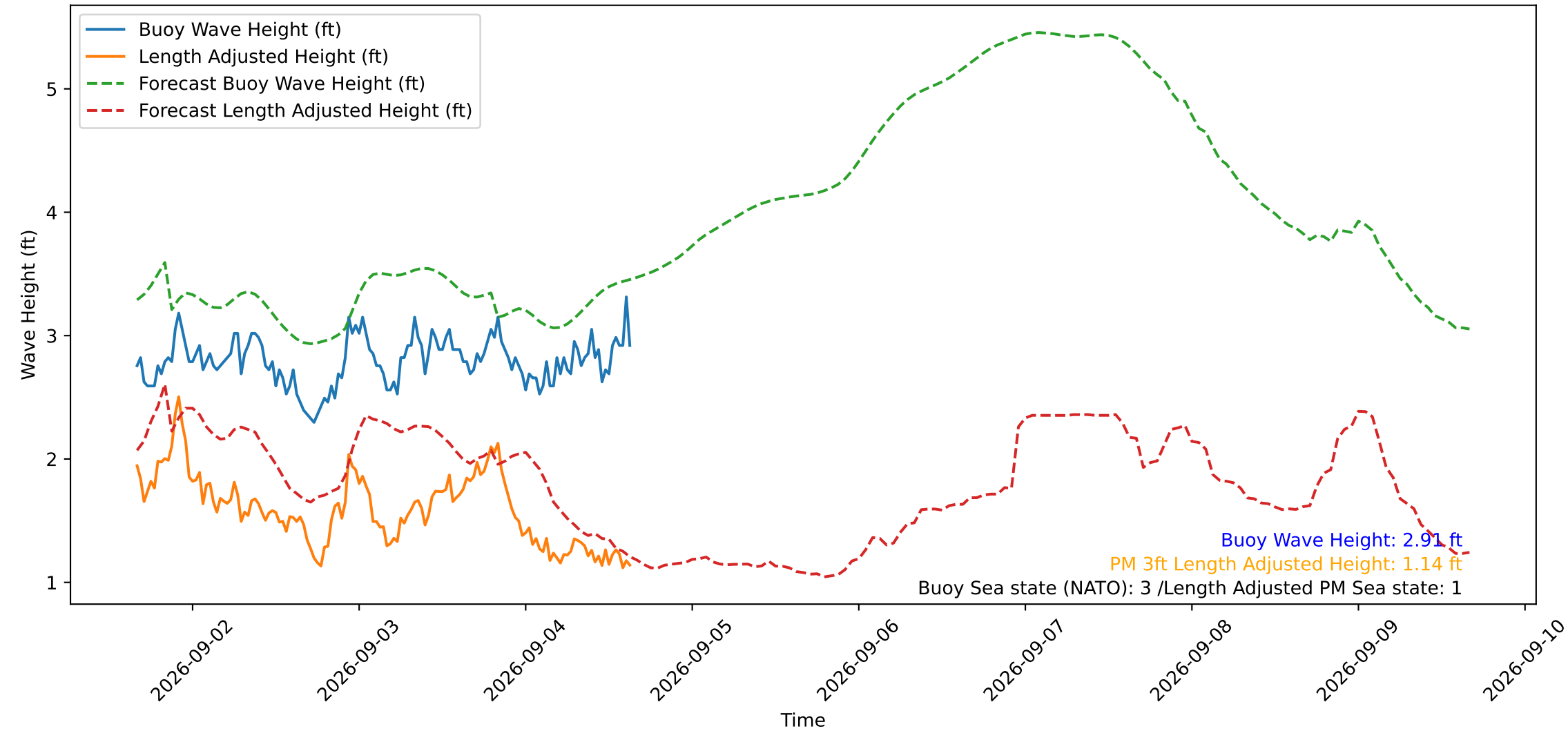
Wave Heights over Time for Red Beach at 2026-09-04 15:50:51
