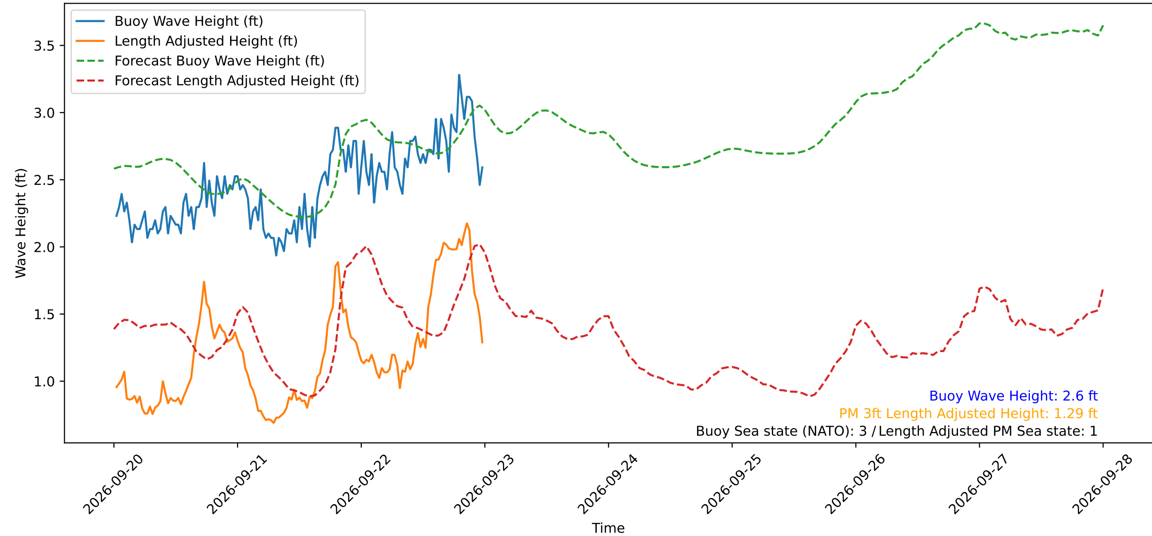
Wave Heights over Time for Red Beach at 2026-09-23 00:20:50
