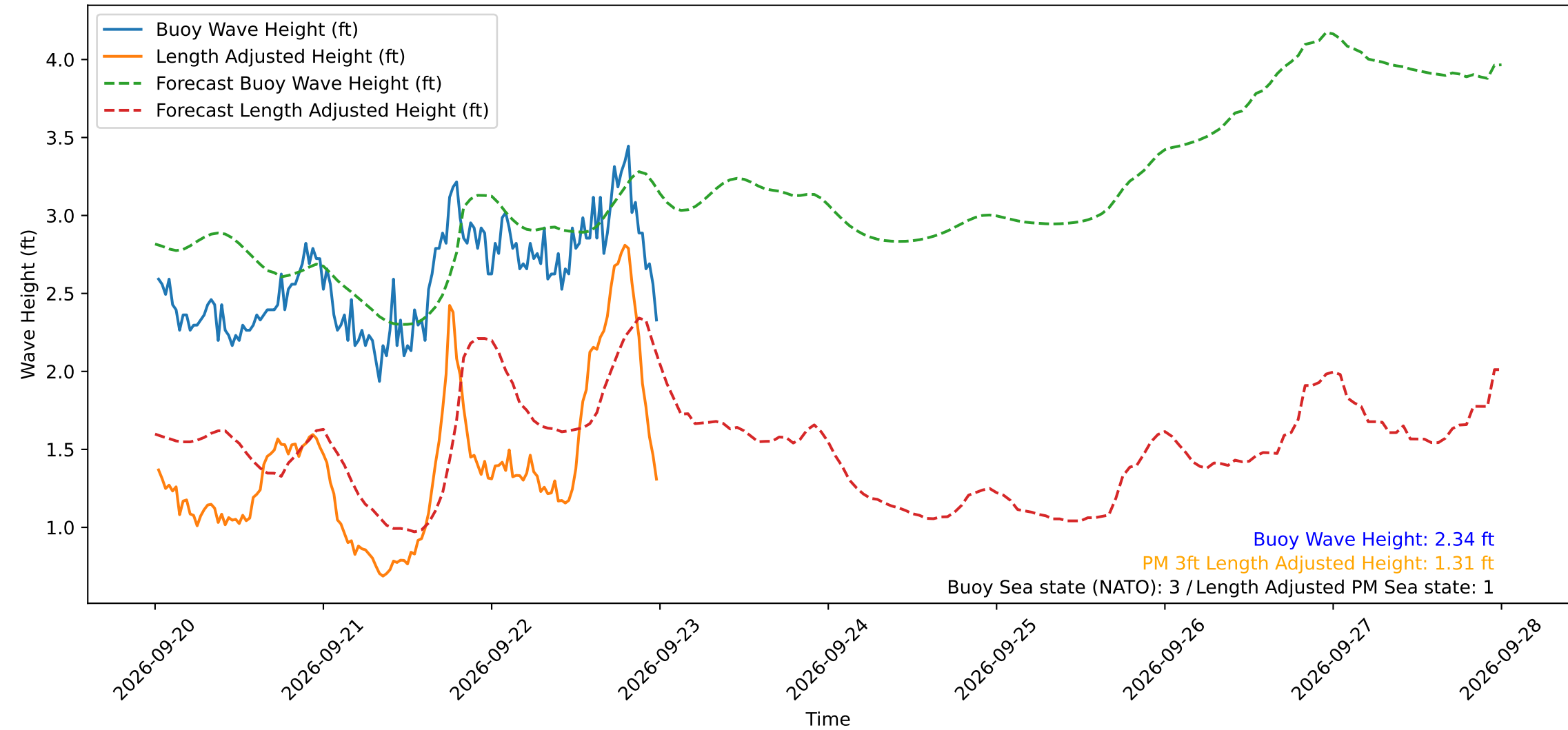
Wave Heights over Time for Green Beach at 2026-09-23 00:21:14
