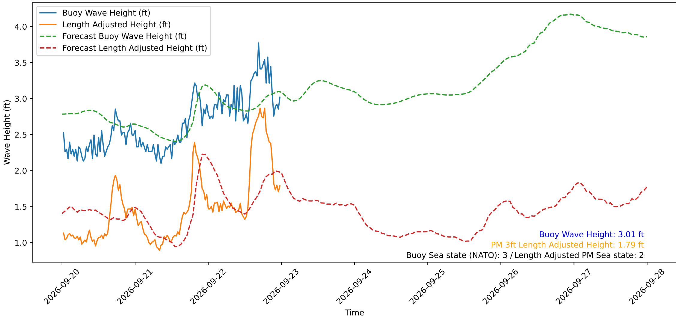
Wave Heights over Time for Oceanside Harbor at 2026-09-23 00:20:29
