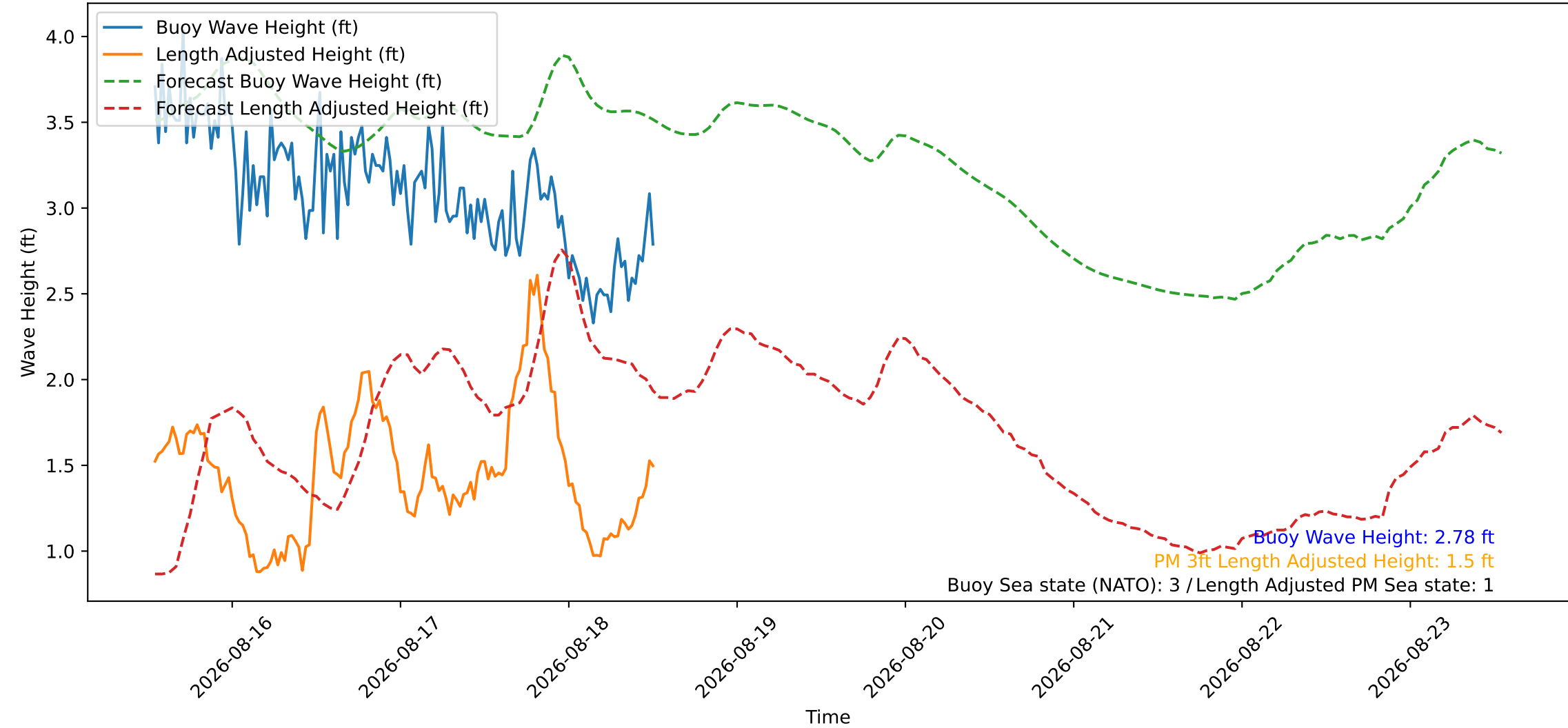
Wave Heights over Time for Red Beach at 2026-08-18 12:50:47
