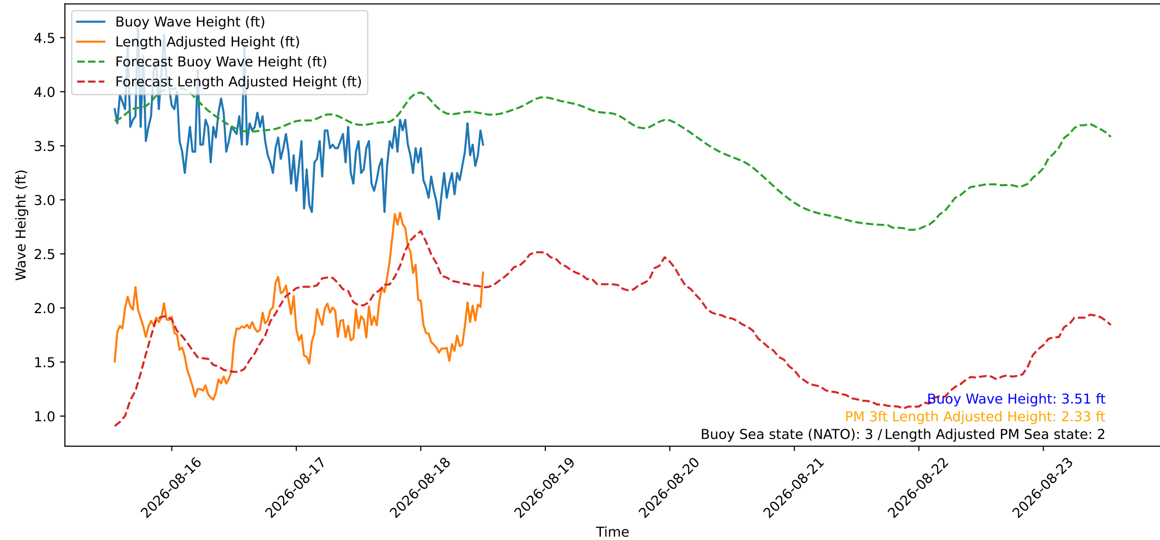
Wave Heights over Time for Oceanside Harbor at 2026-08-18 12:50:26
