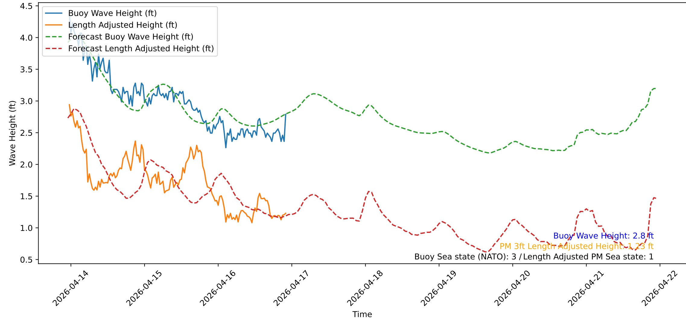
Wave Heights over Time for Red Beach at 2026-04-16 23:00:51
