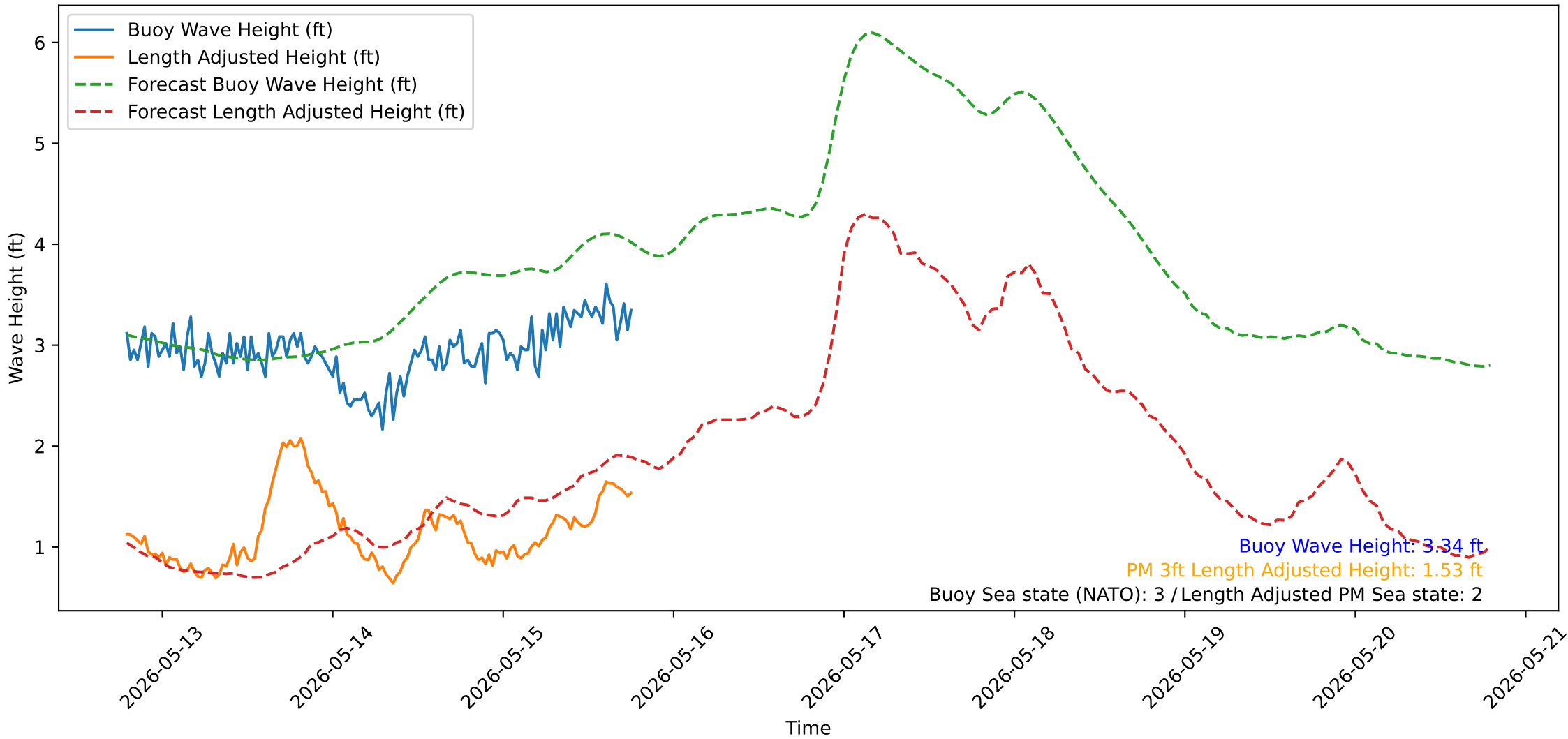
Wave Heights over Time for Oceanside Harbor at 2026-05-15 18:50:31
