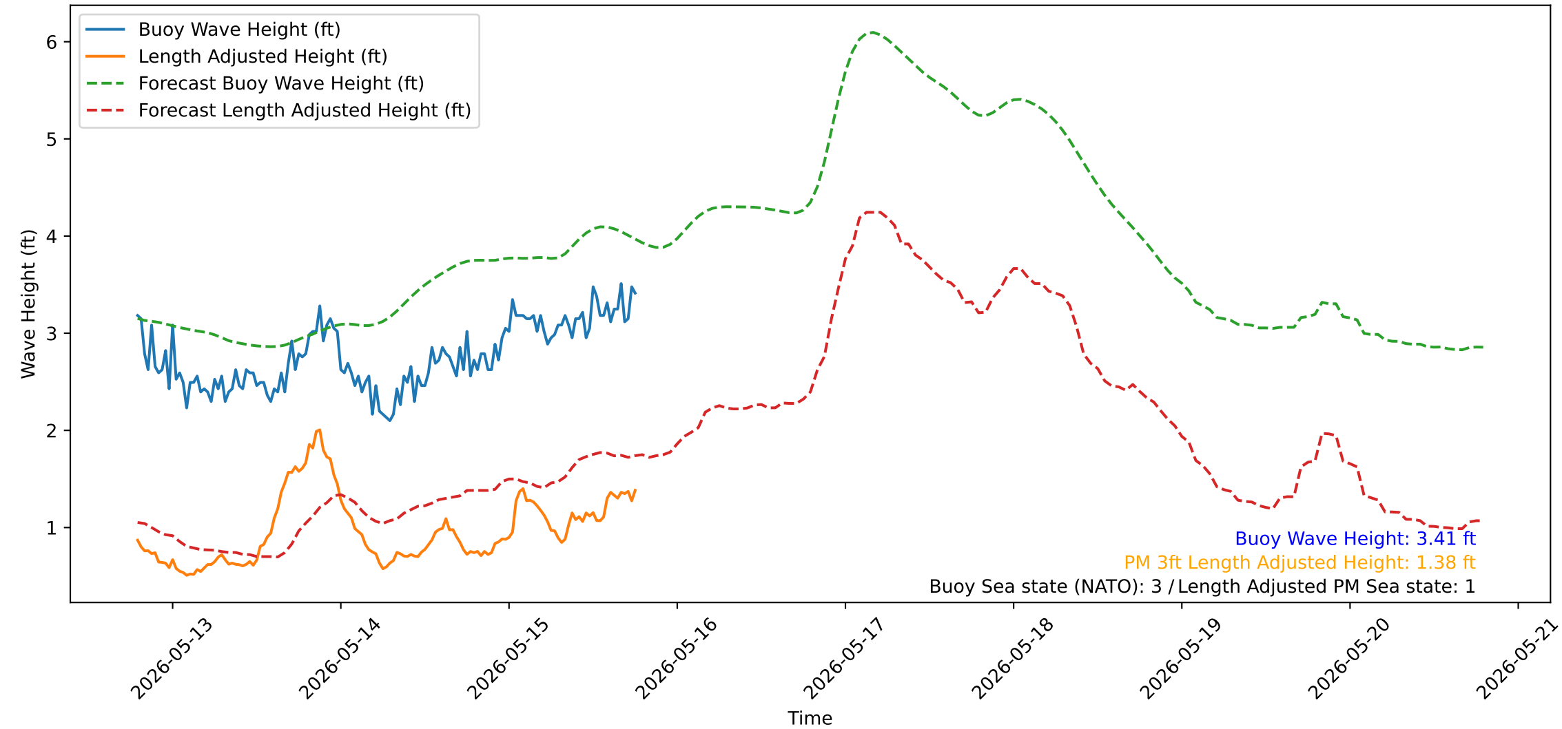
Wave Heights over Time for Green Beach at 2026-05-15 18:51:14
