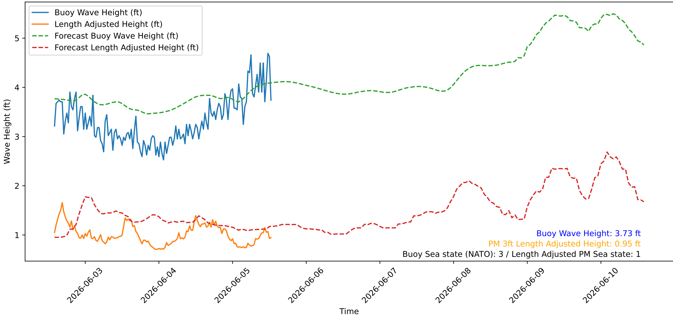
Wave Heights over Time for Red Beach at 2026-06-05 13:40:45
