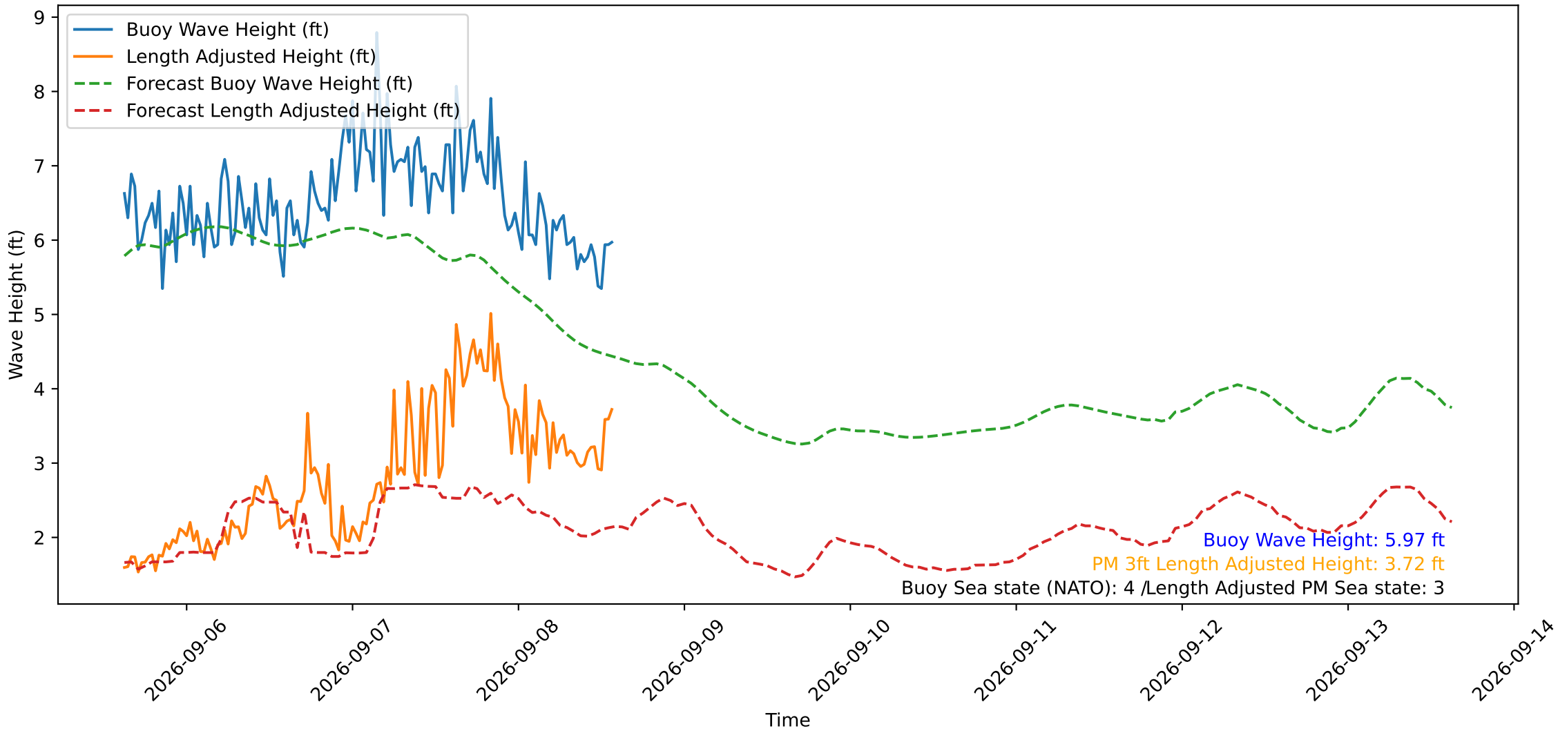
Wave Heights over Time for Green Beach at 2026-09-08 14:31:12
