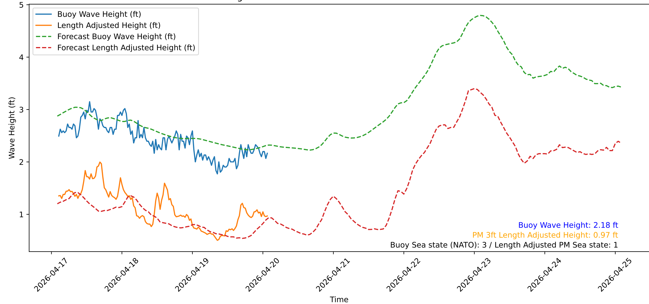
Wave Heights over Time for Red Beach at 2026-04-20 02:20:52
