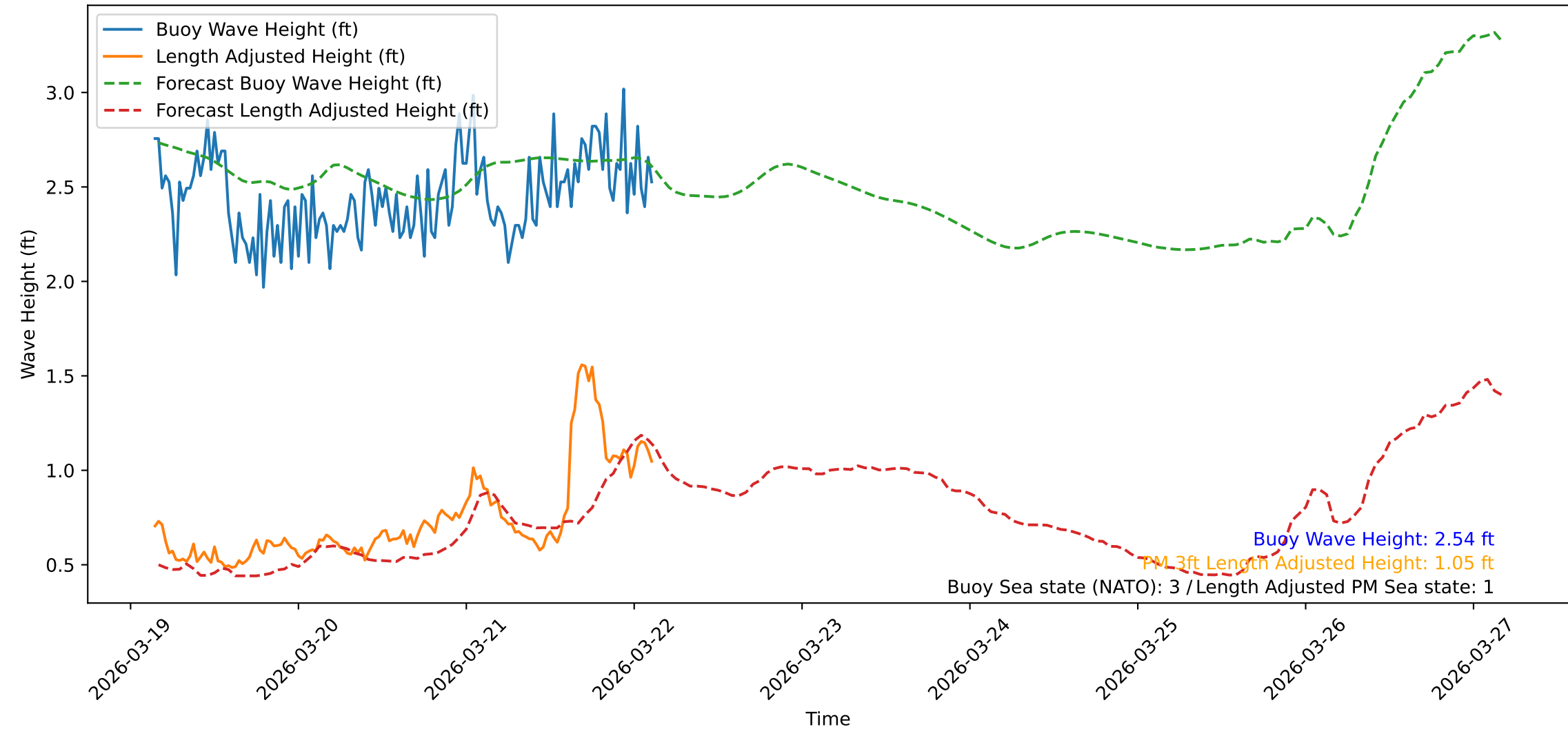
Wave Heights over Time for Oceanside Harbor at 2026-03-22 03:40:31
