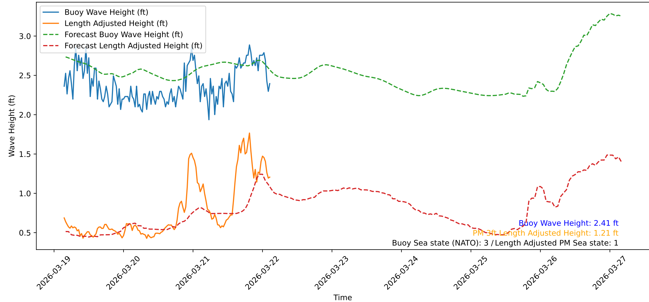
Wave Heights over Time for Green Beach at 2026-03-22 03:41:10
