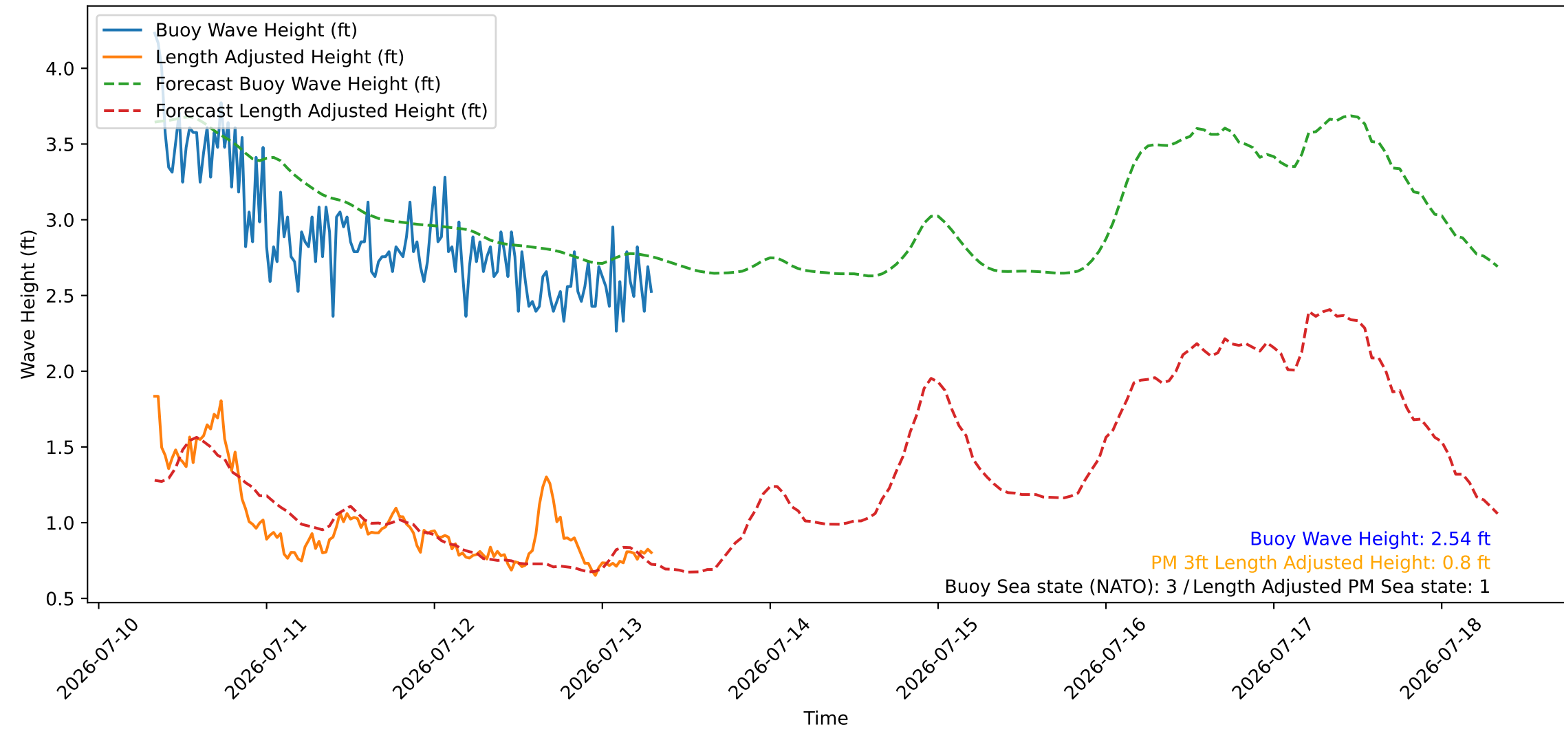
Wave Heights over Time for Oceanside Harbor at 2026-07-13 07:50:26
