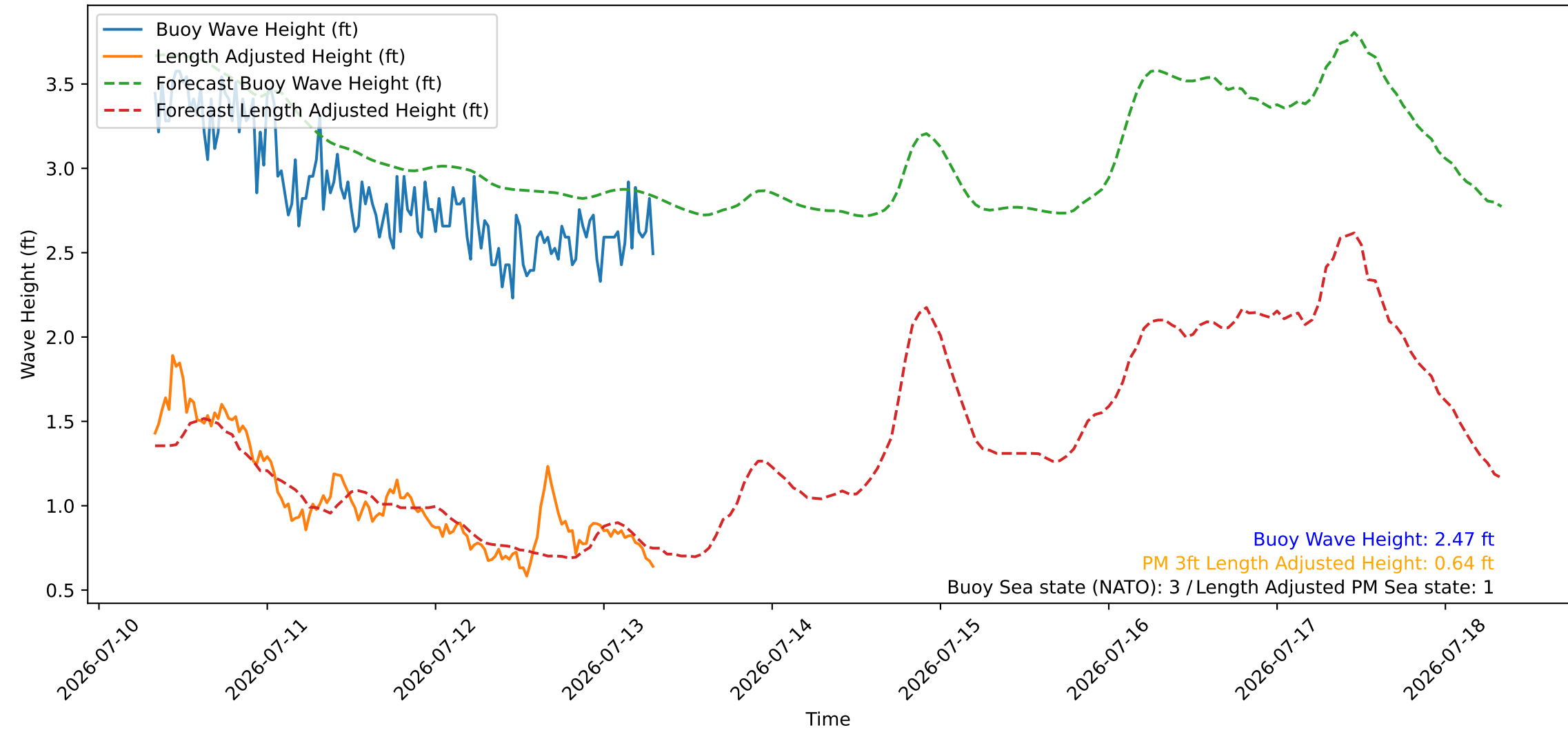
Wave Heights over Time for Green Beach at 2026-07-13 07:51:10
