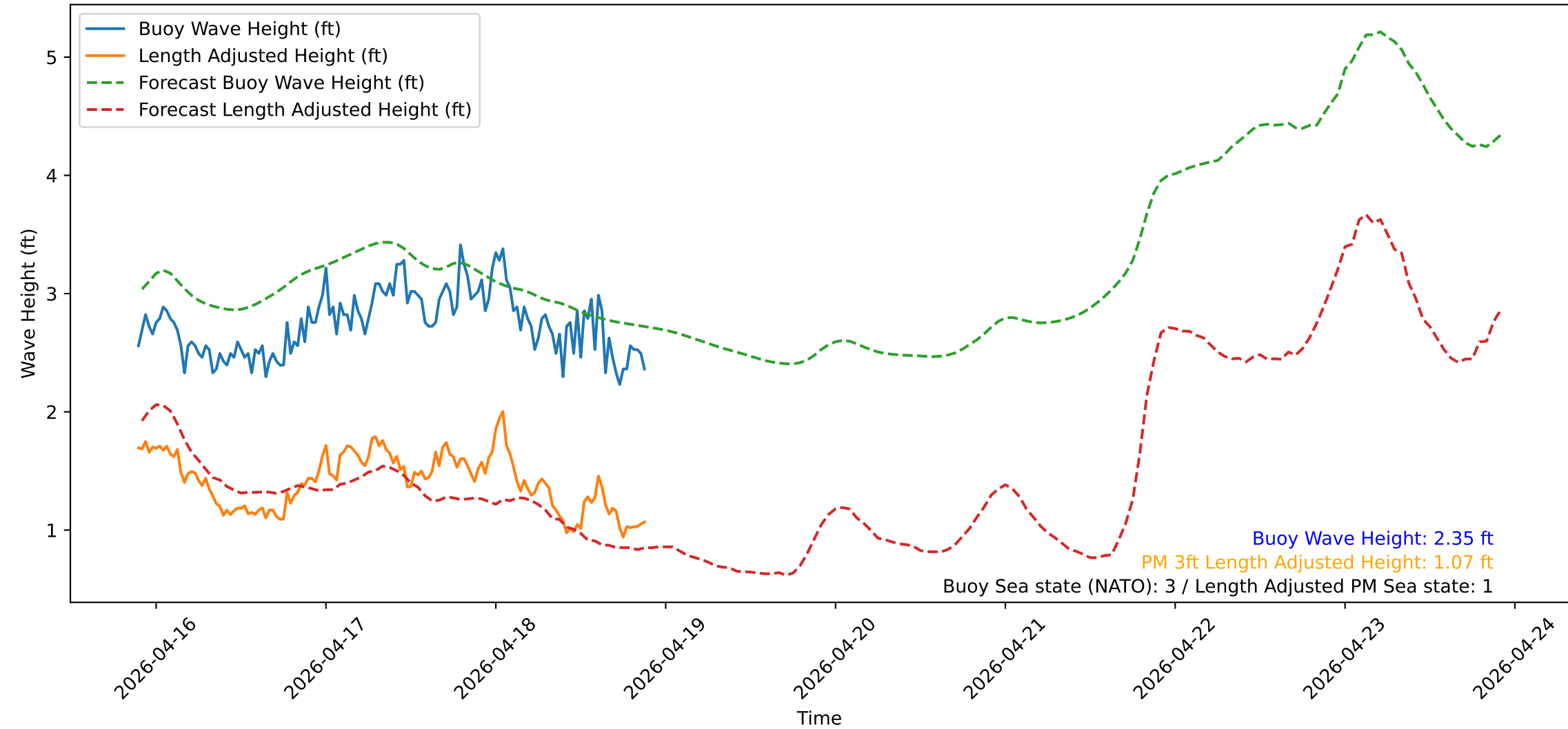
Wave Heights over Time for Oceanside Harbor at 2026-04-18 21:30:31
