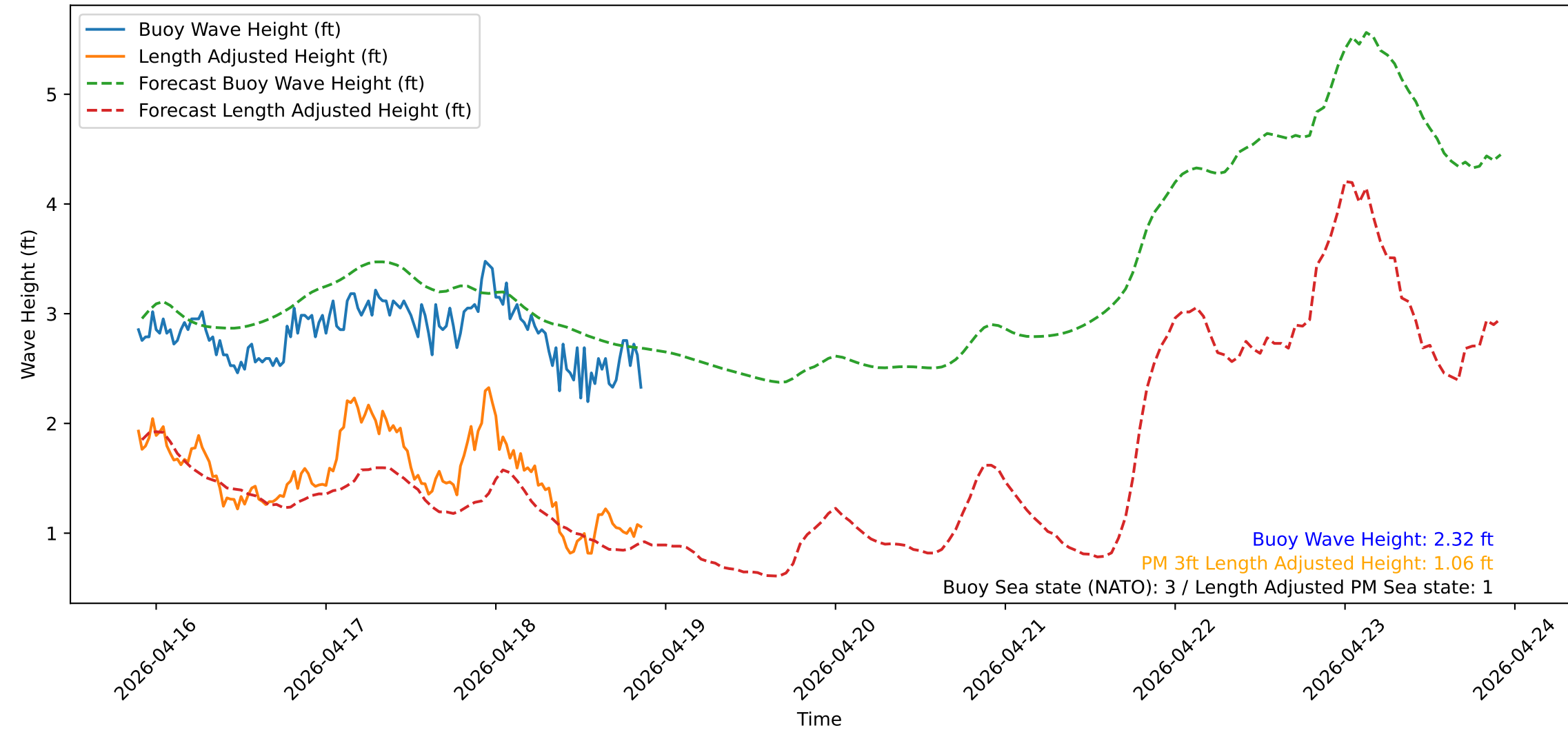
Wave Heights over Time for Green Beach at 2026-04-18 21:31:13
