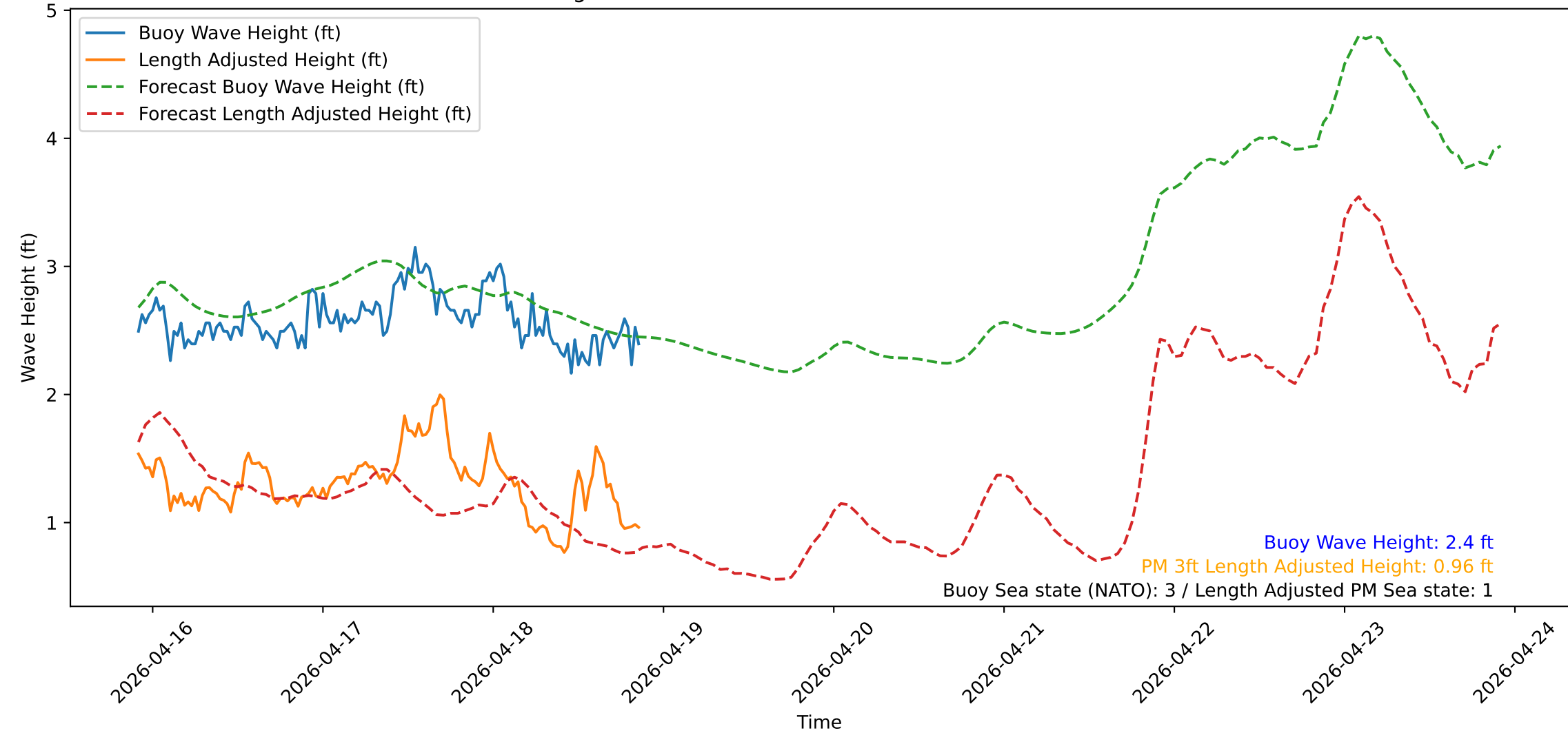
Wave Heights over Time for Red Beach at 2026-04-18 21:30:50
