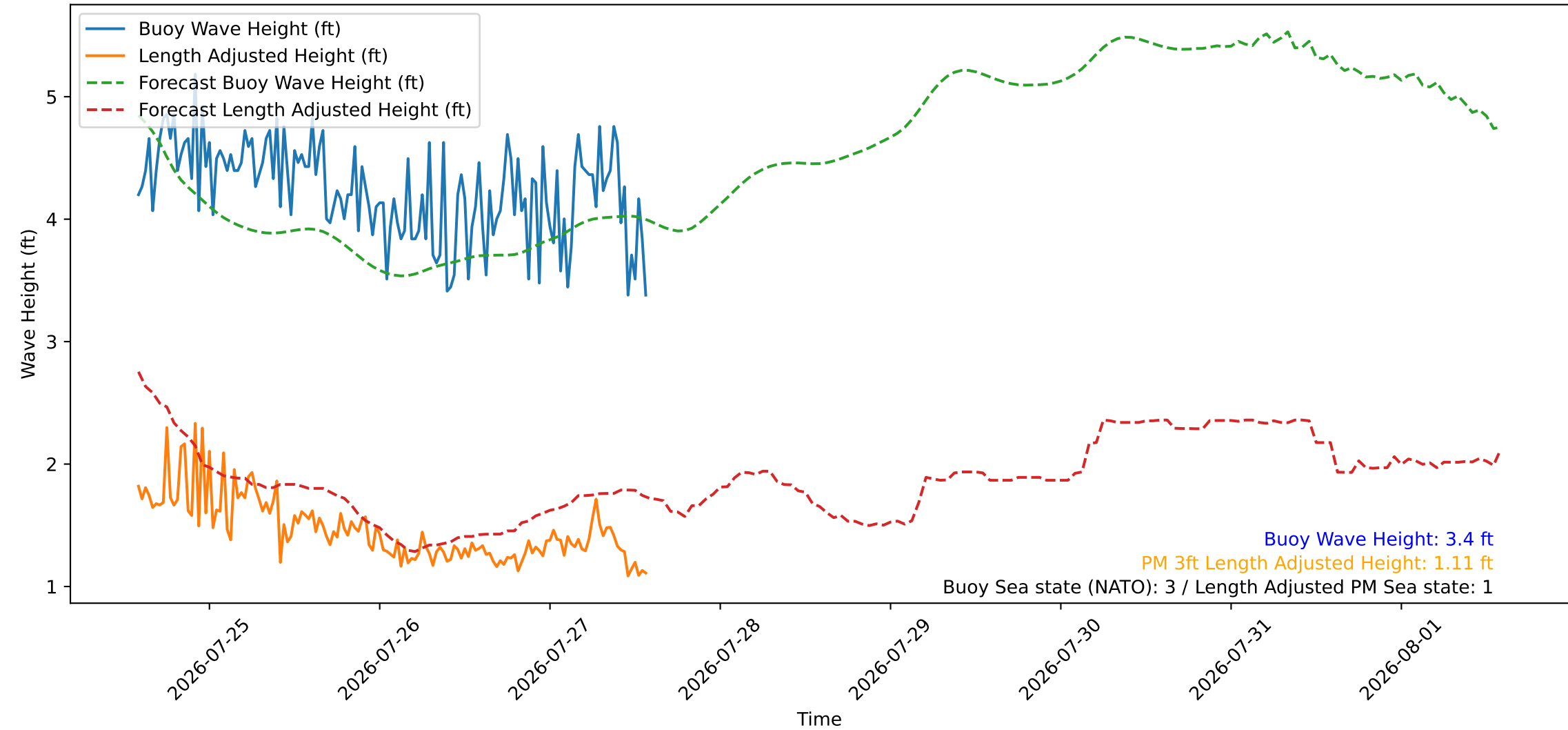
Wave Heights over Time for Green Beach at 2026-07-27 14:11:08
