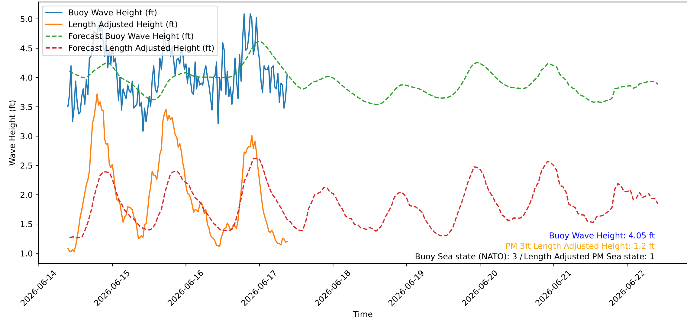
Wave Heights over Time for Green Beach at 2026-06-17 09:41:09
