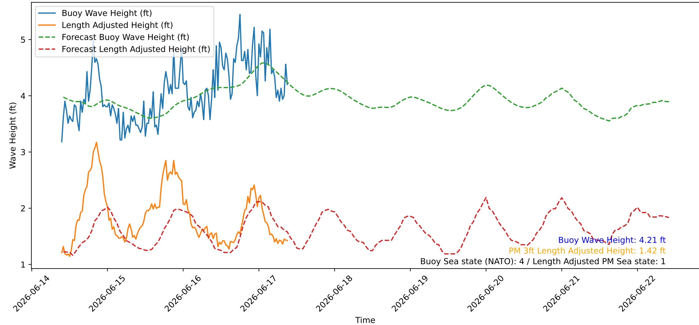
Wave Heights over Time for Oceanside Harbor at 2026-06-17 09:40:26
