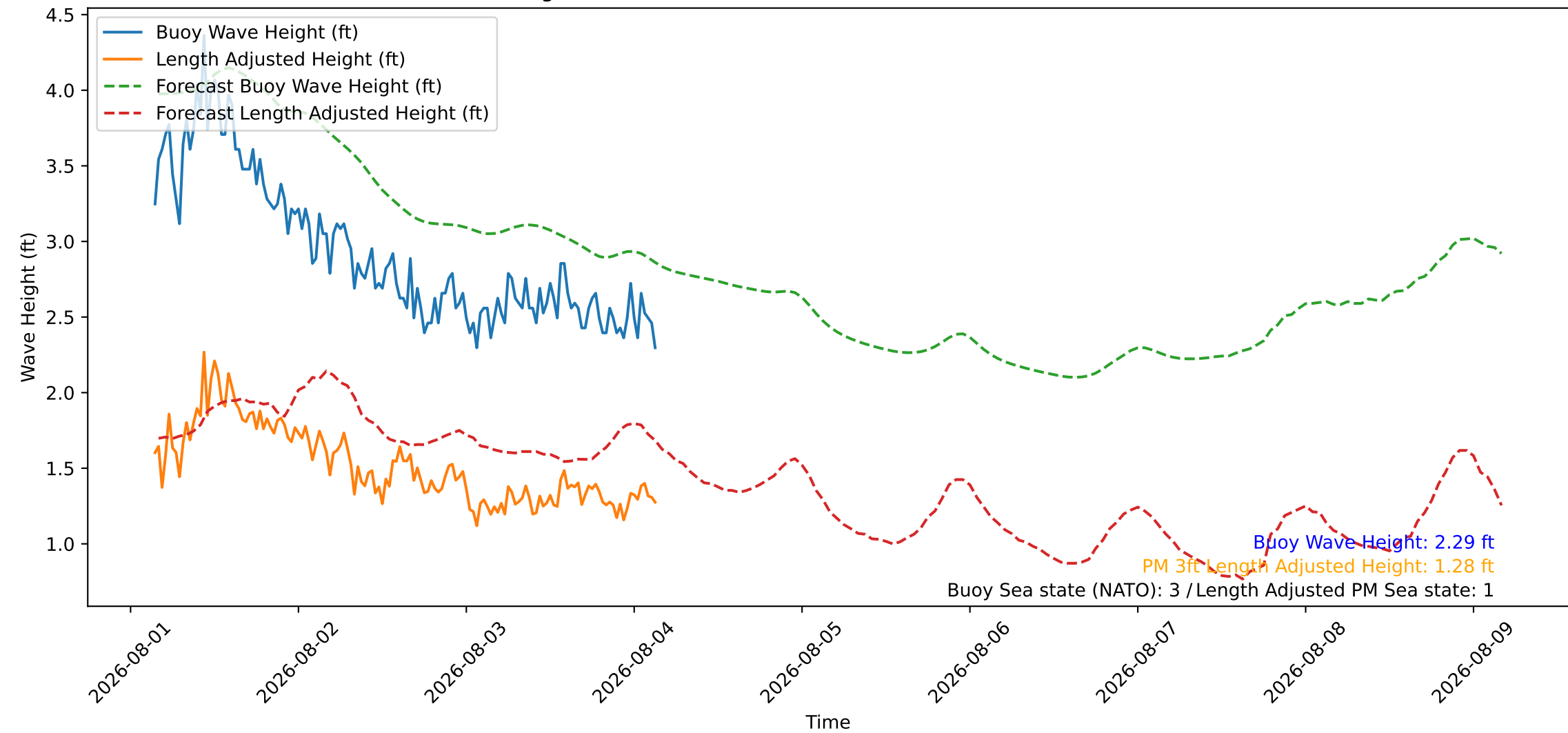
Wave Heights over Time for Oceanside Harbor at 2026-08-04 03:40:26
