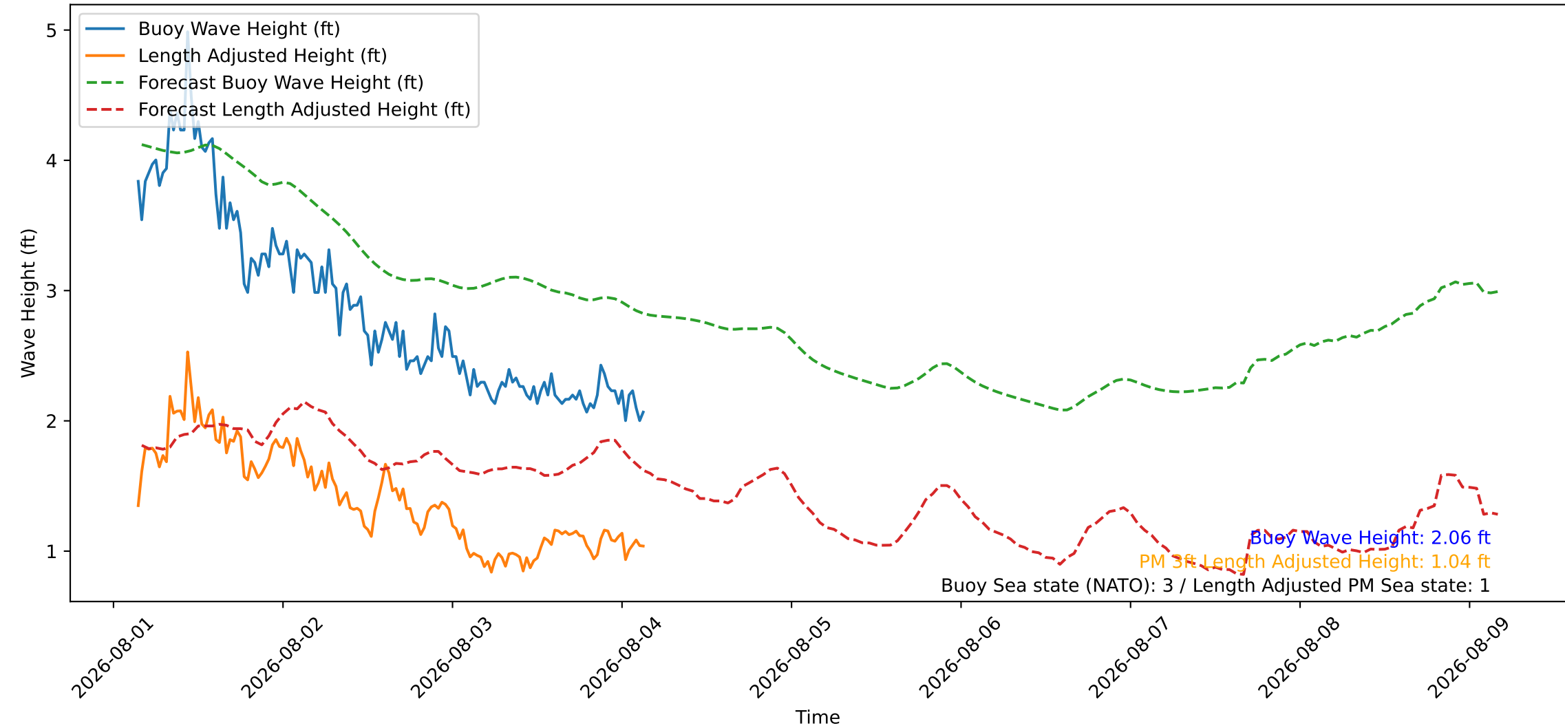
Wave Heights over Time for Green Beach at 2026-08-04 03:41:08
