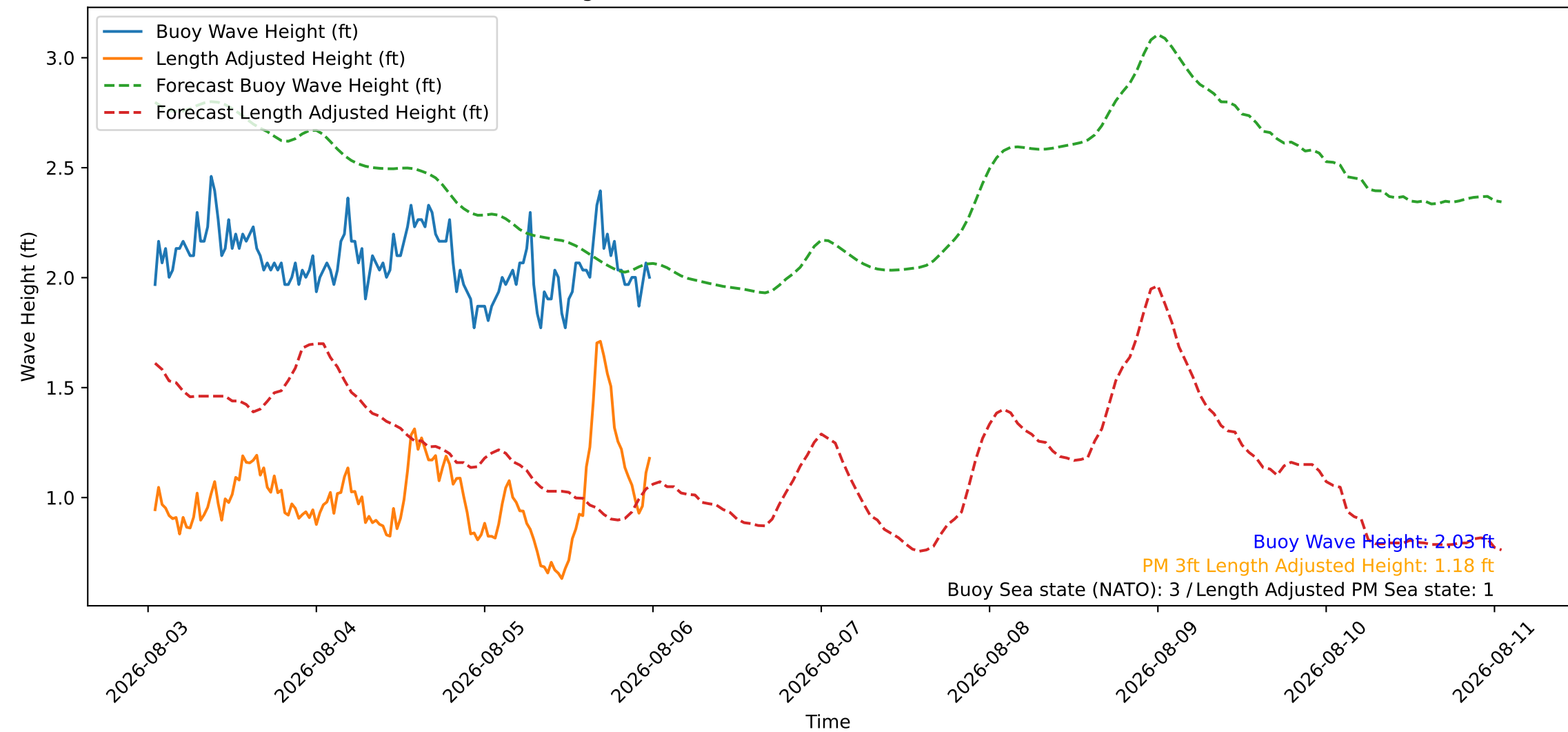
Wave Heights over Time for Red Beach at 2026-08-06 00:40:46
