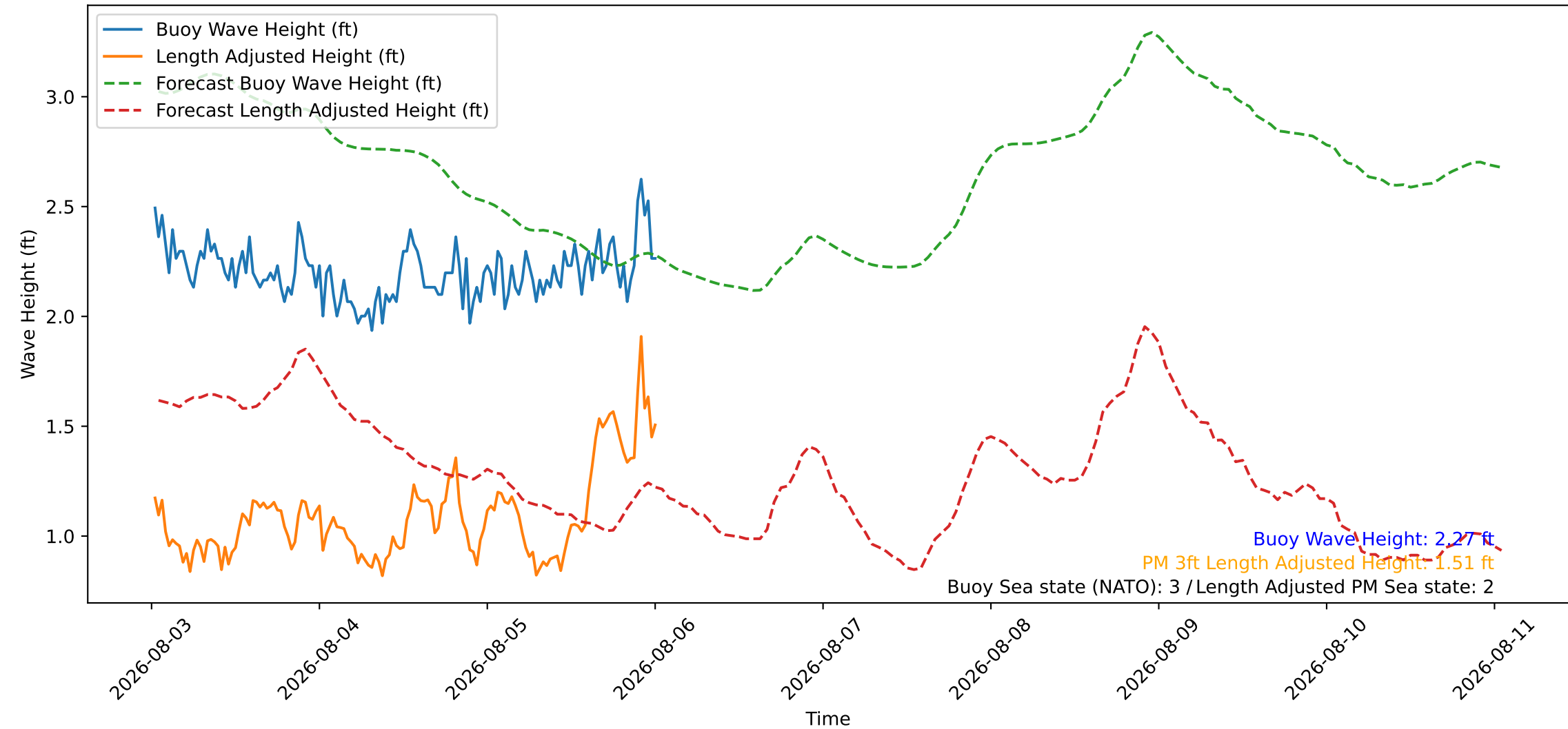
Wave Heights over Time for Green Beach at 2026-08-06 00:41:08
