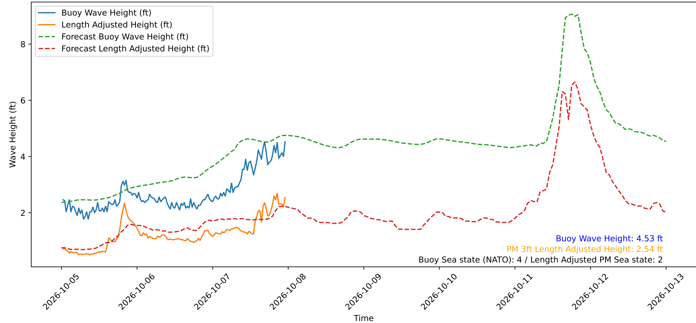
Wave Heights over Time for Green Beach at 2026-10-08 00:01:12
