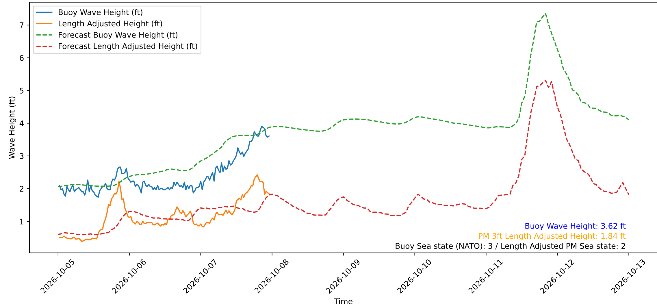
Wave Heights over Time for Red Beach at 2026-10-08 00:00:49
