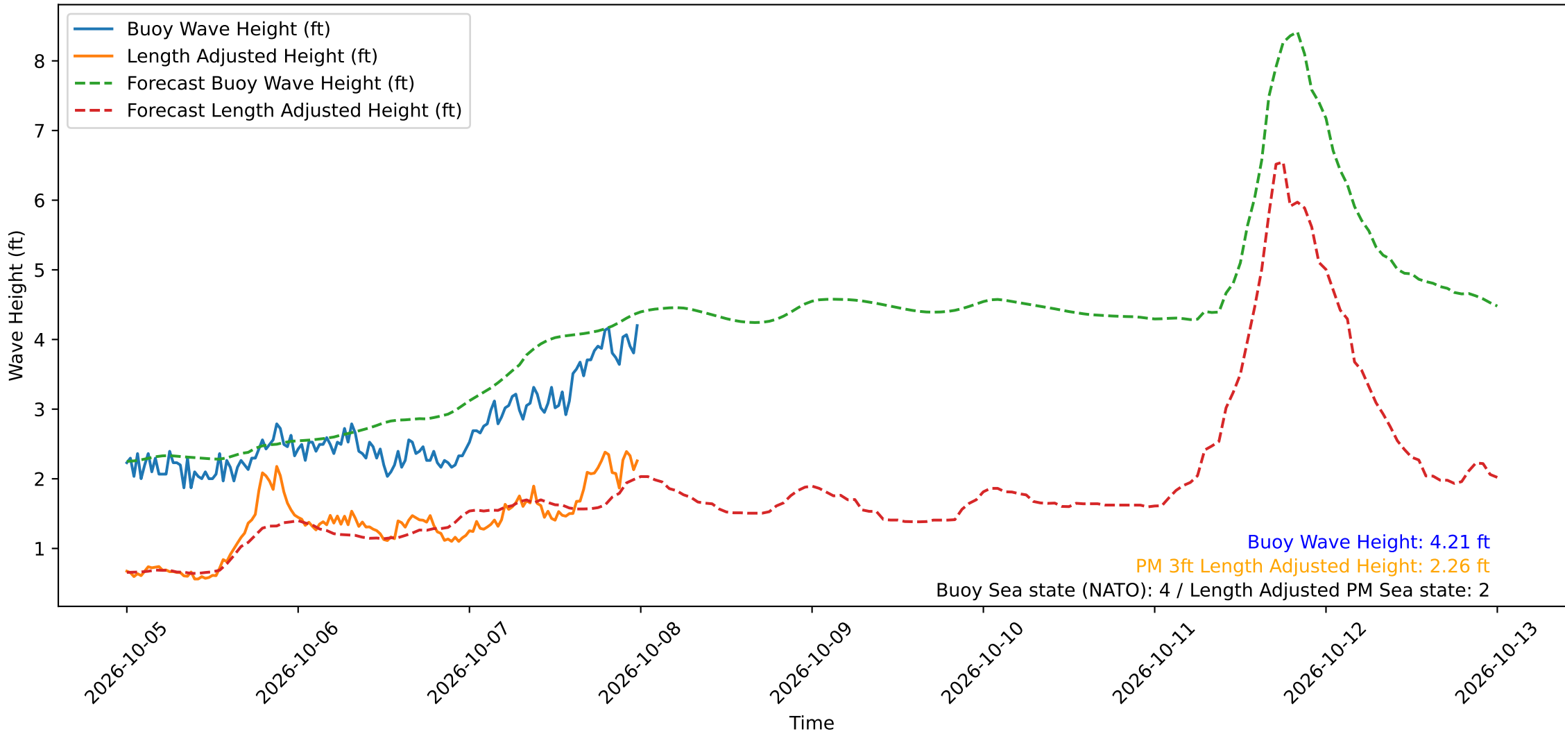
Wave Heights over Time for Oceanside Harbor at 2026-10-08 00:00:30
