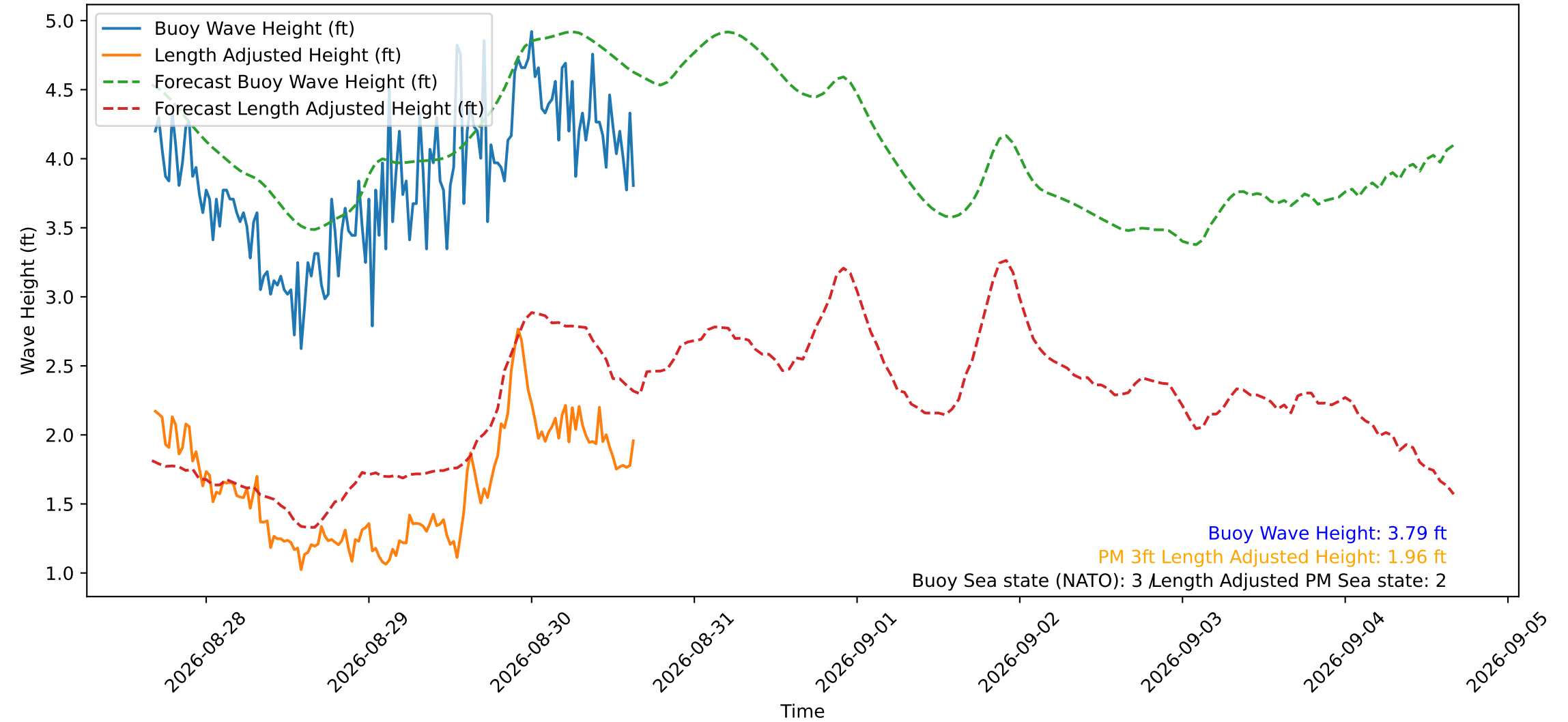
Wave Heights over Time for Green Beach at 2026-08-30 16:01:12
