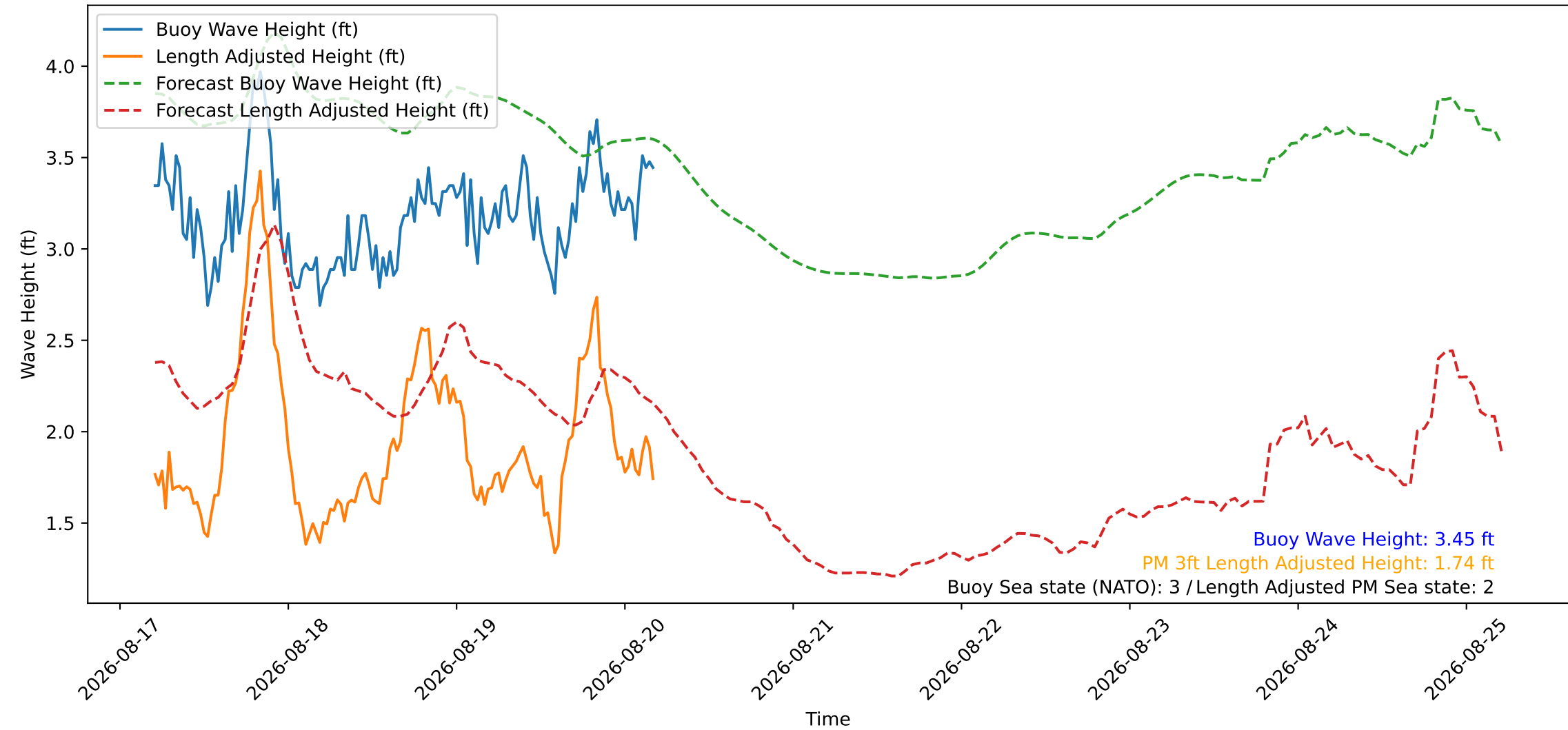
Wave Heights over Time for Green Beach at 2026-08-20 04:51:11
