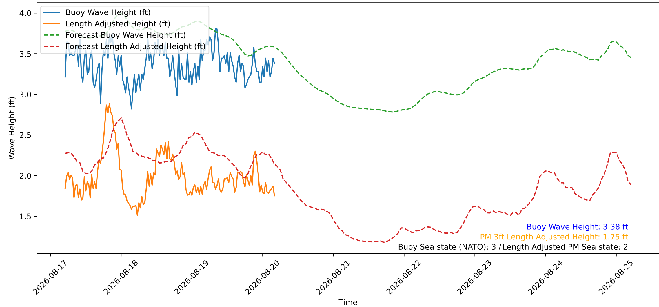
Wave Heights over Time for Oceanside Harbor at 2026-08-20 04:50:26
