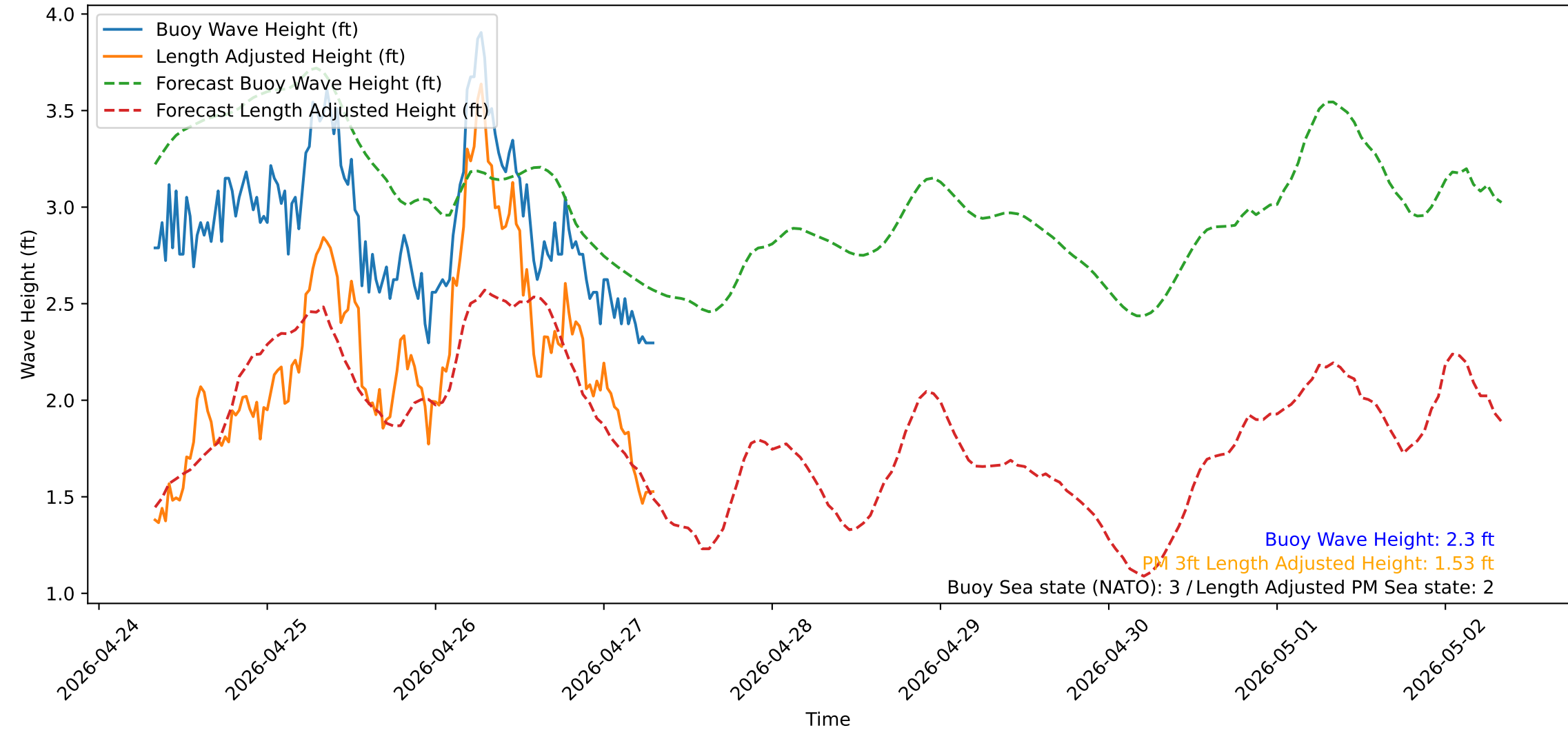
Wave Heights over Time for Oceanside Harbor at 2026-04-27 07:50:31
