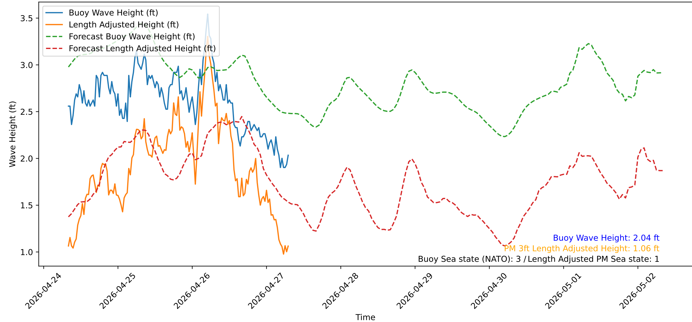
Wave Heights over Time for Red Beach at 2026-04-27 07:50:51
