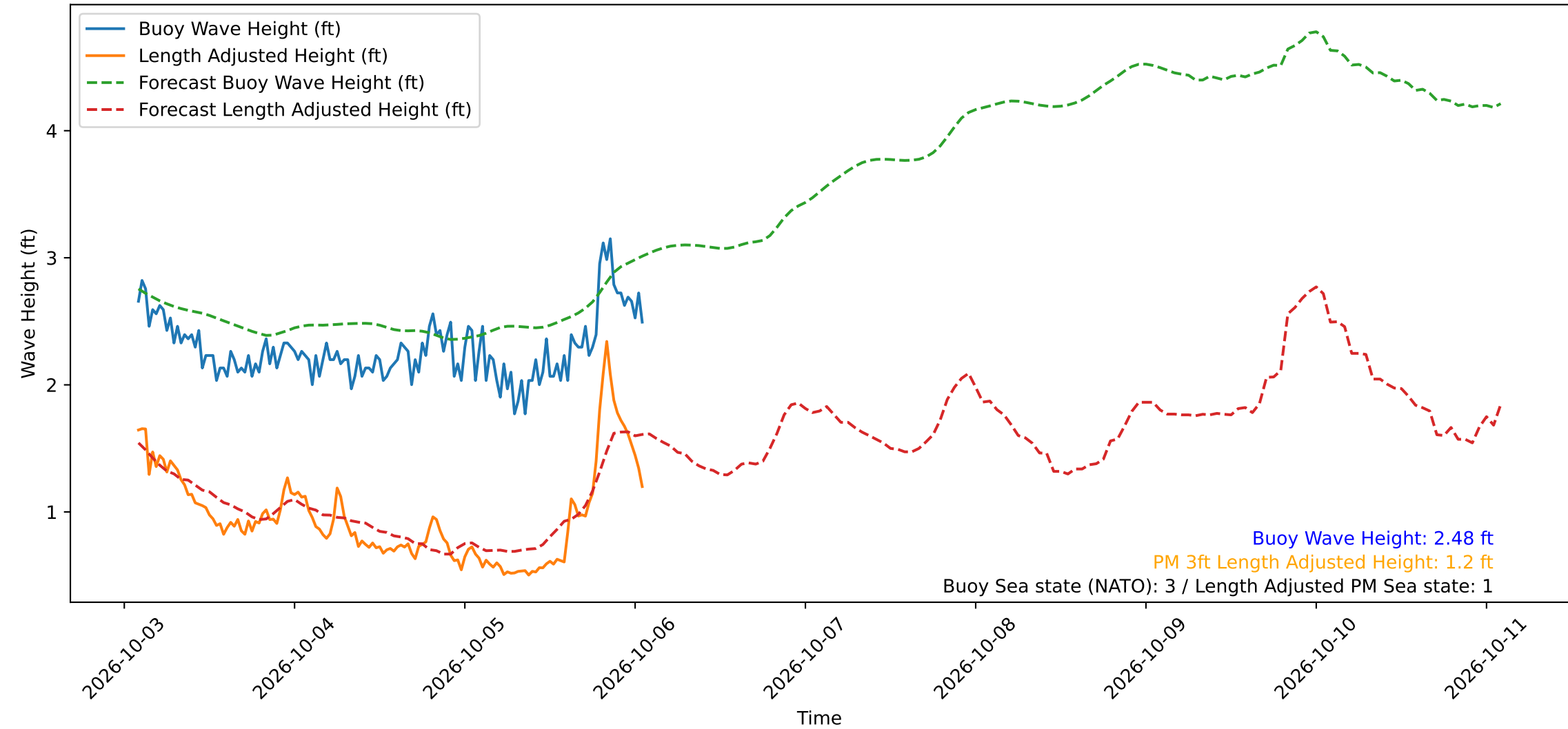
Wave Heights over Time for Green Beach at 2026-10-06 01:41:11
