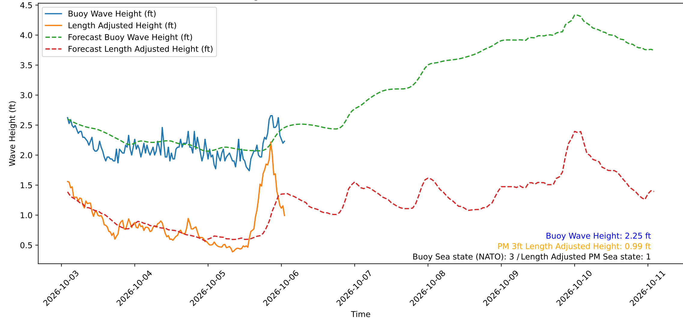
Wave Heights over Time for Red Beach at 2026-10-06 01:40:49
