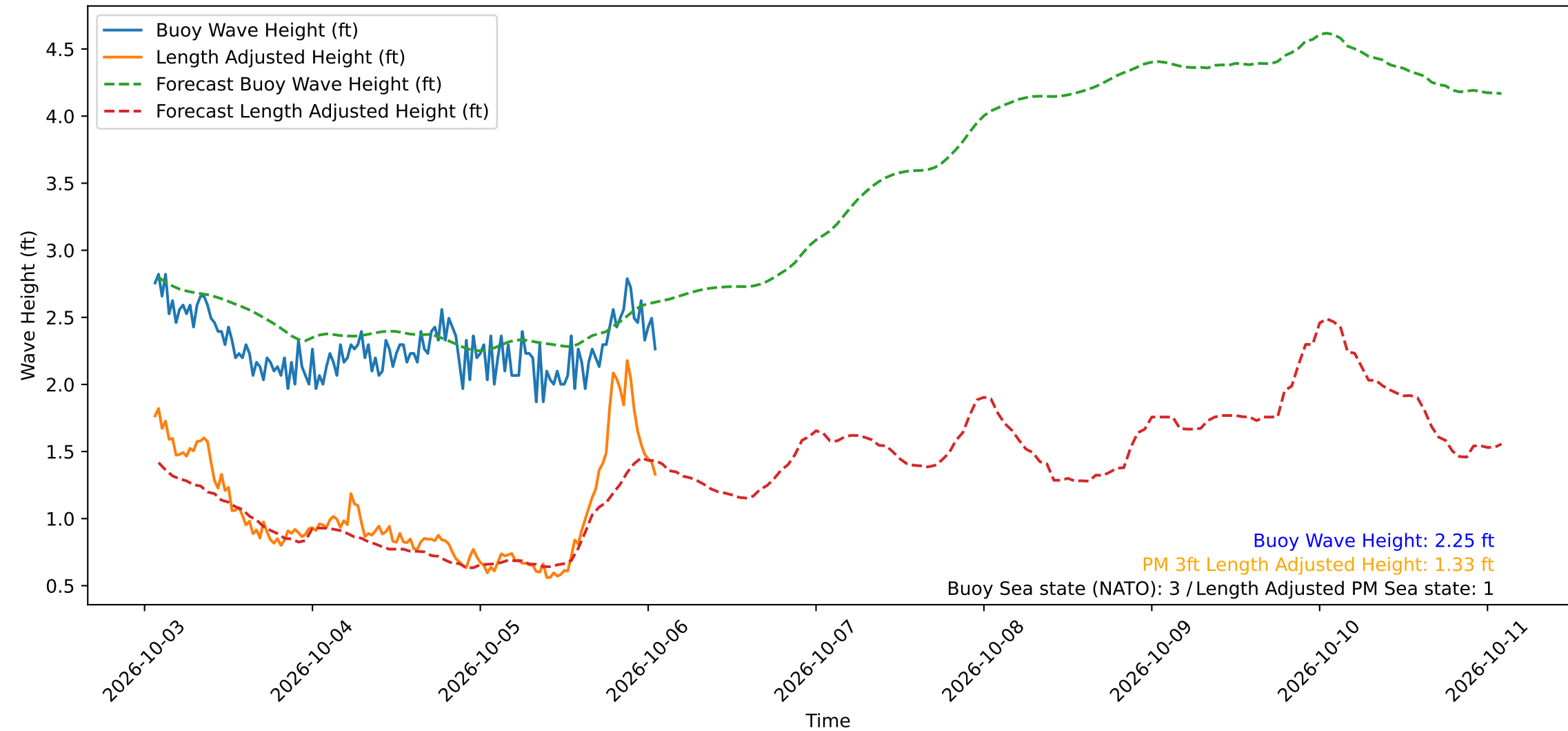
Wave Heights over Time for Oceanside Harbor at 2026-10-06 01:40:29
