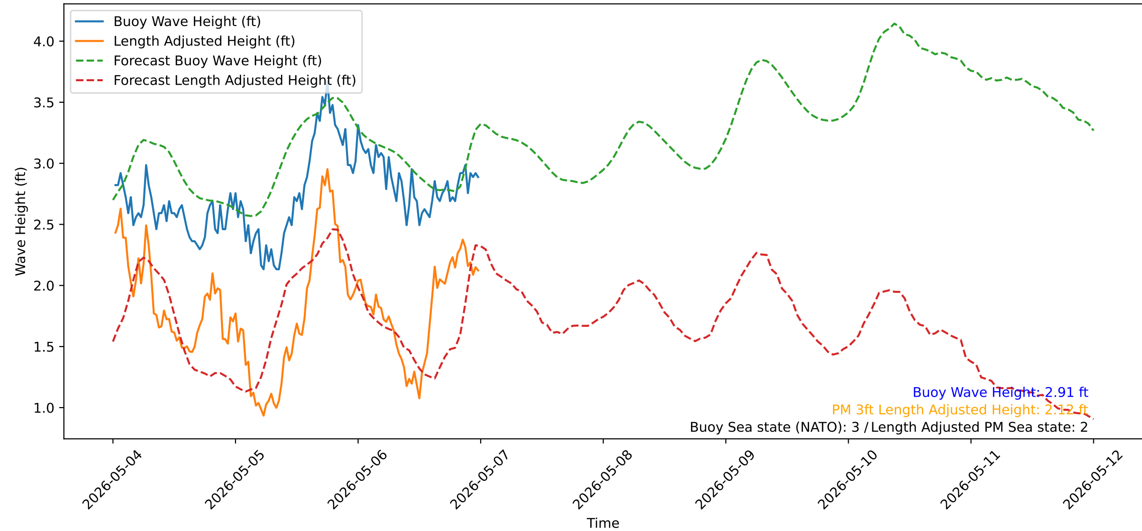
Wave Heights over Time for Green Beach at 2026-05-07 00:21:14
