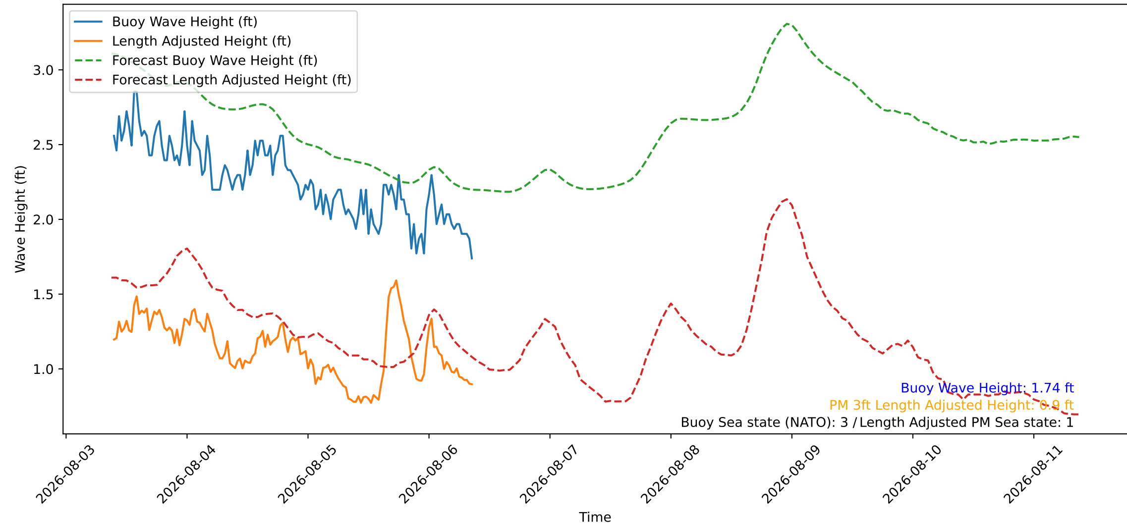
Wave Heights over Time for Oceanside Harbor at 2026-08-06 09:20:25
