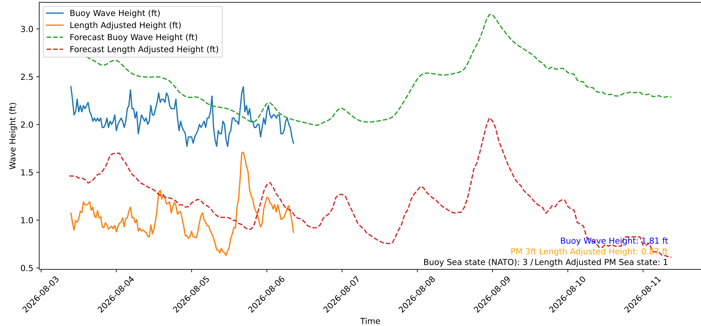
Wave Heights over Time for Red Beach at 2026-08-06 09:20:46
