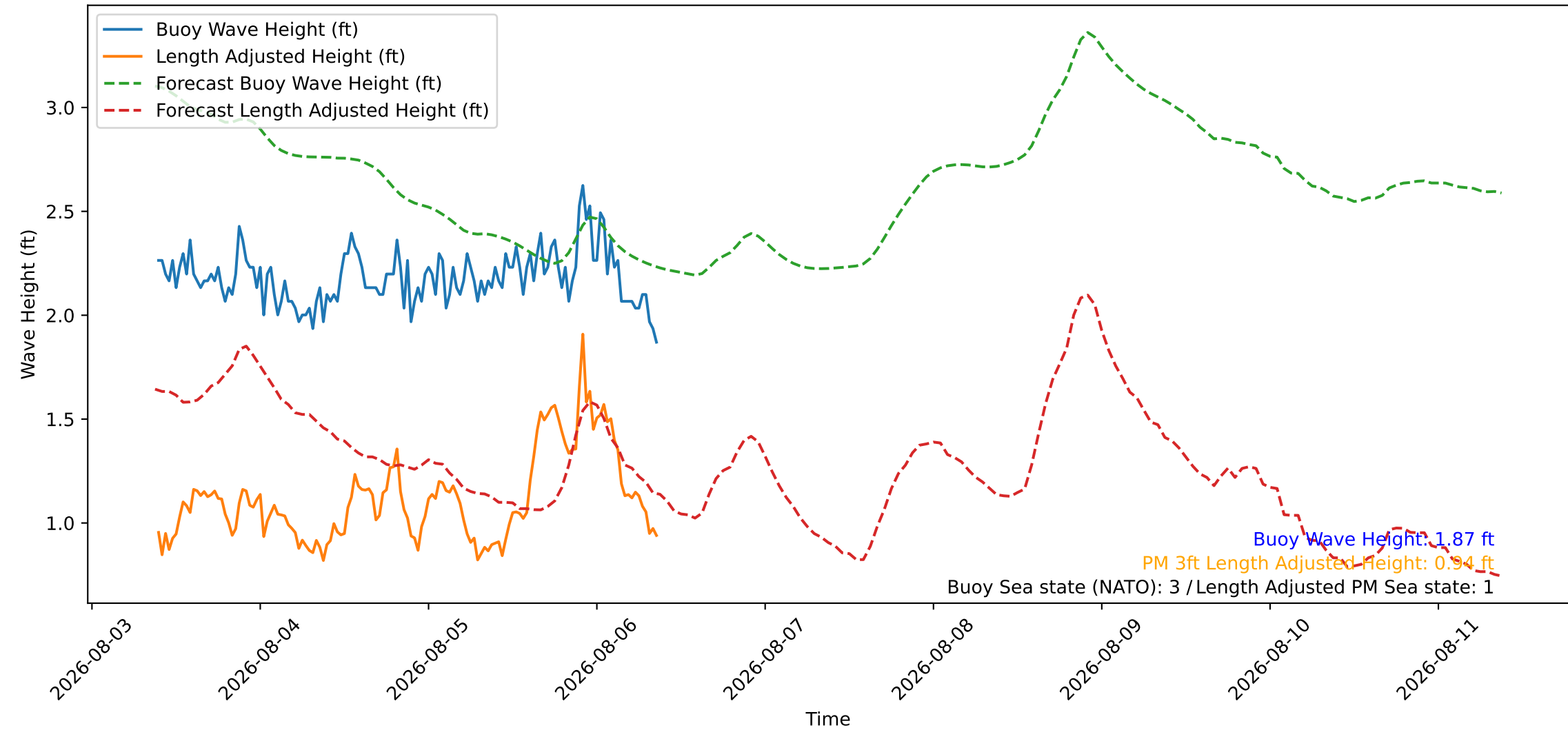
Wave Heights over Time for Green Beach at 2026-08-06 09:21:09
