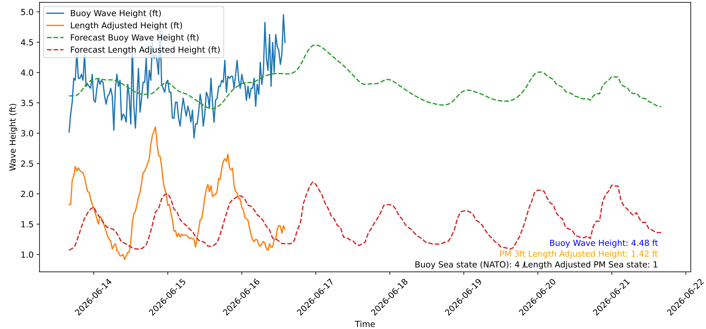
Wave Heights over Time for Red Beach at 2026-06-16 15:30:45
