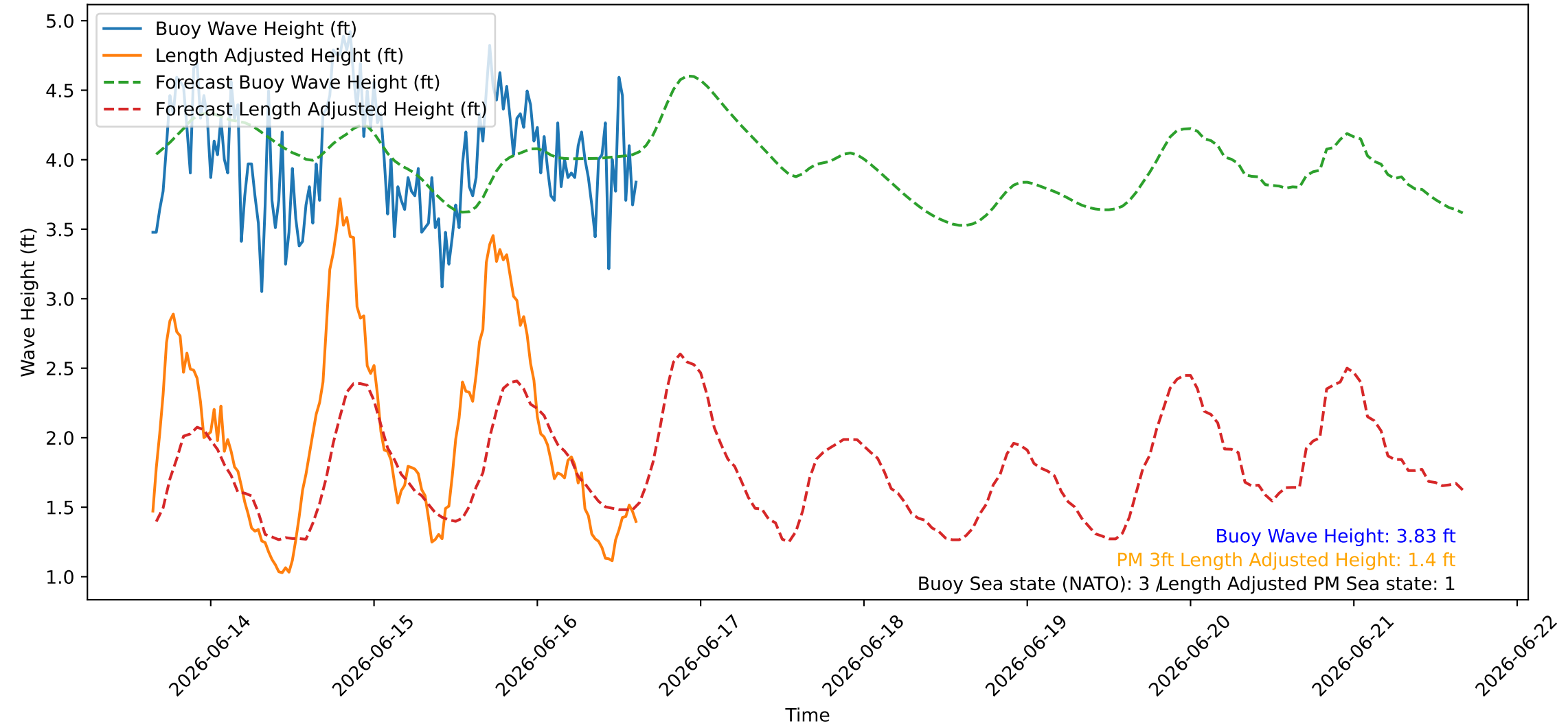
Wave Heights over Time for Green Beach at 2026-06-16 15:31:07
