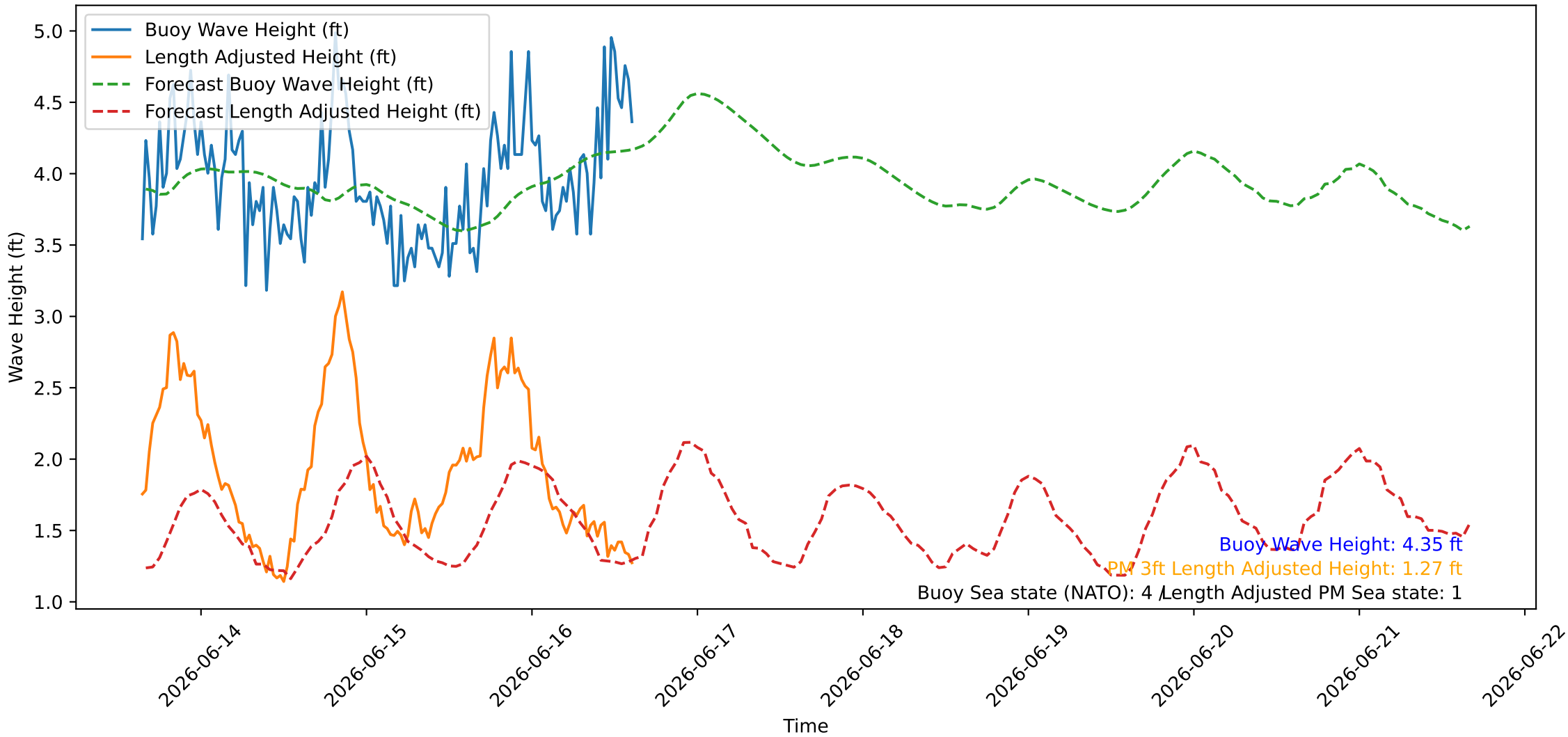
Wave Heights over Time for Oceanside Harbor at 2026-06-16 15:30:26
