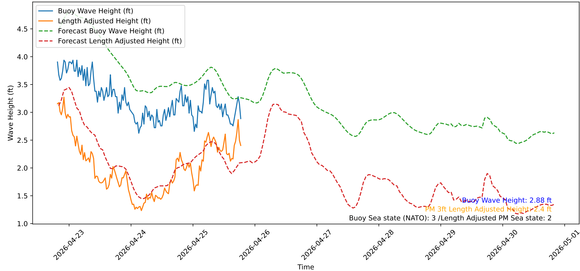
Wave Heights over Time for Green Beach at 2026-04-25 19:31:12
