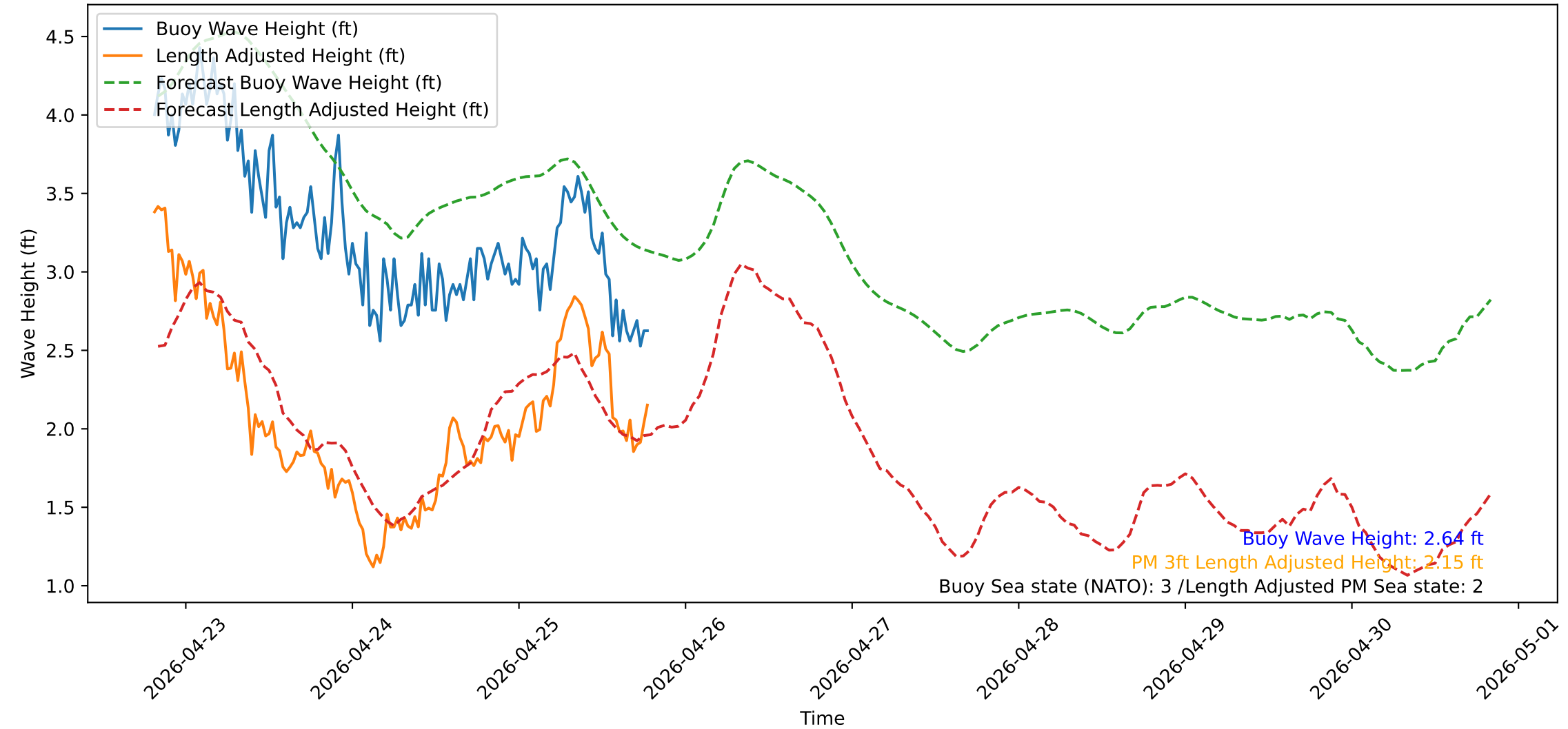
Wave Heights over Time for Oceanside Harbor at 2026-04-25 19:30:31
