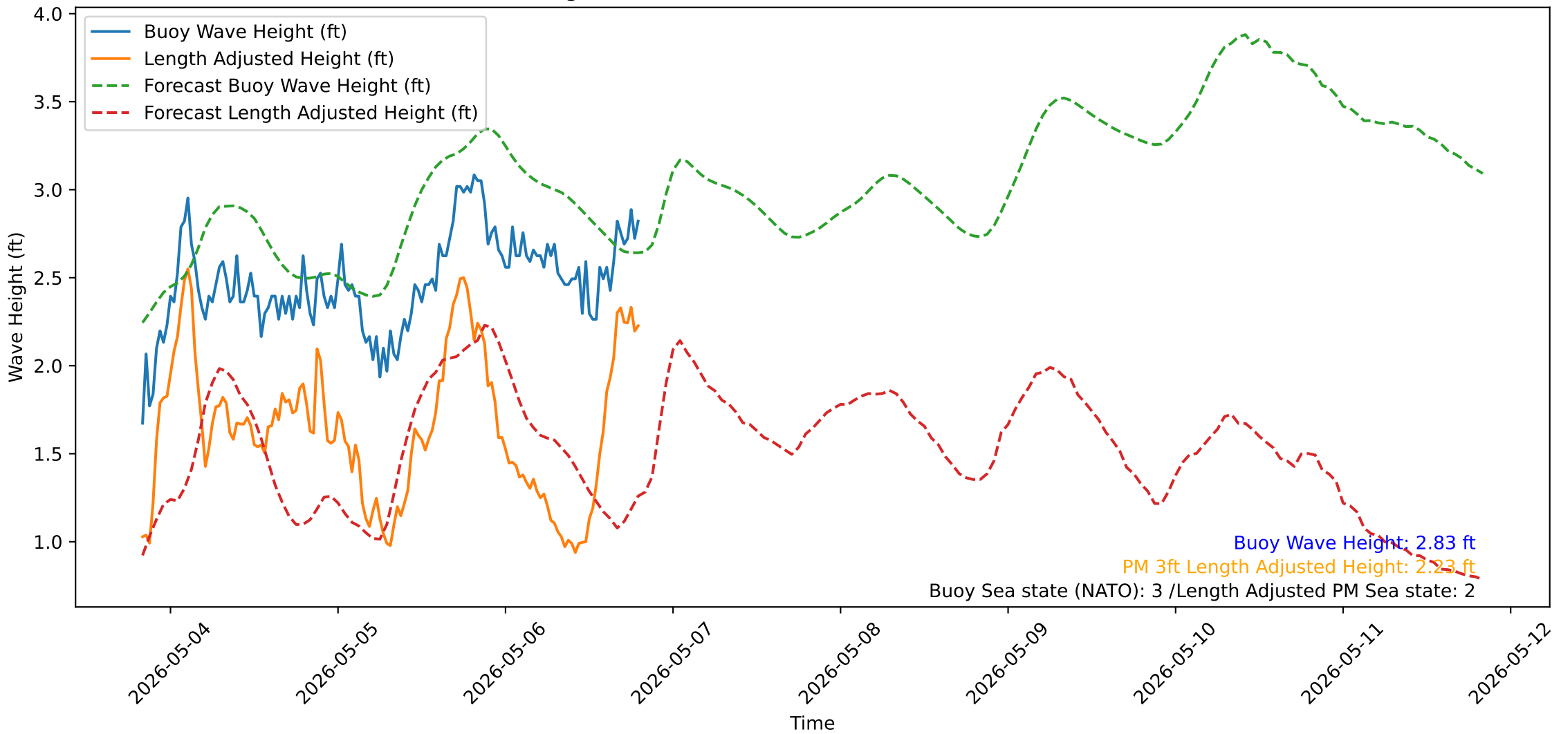
Wave Heights over Time for Red Beach at 2026-05-06 19:40:51
