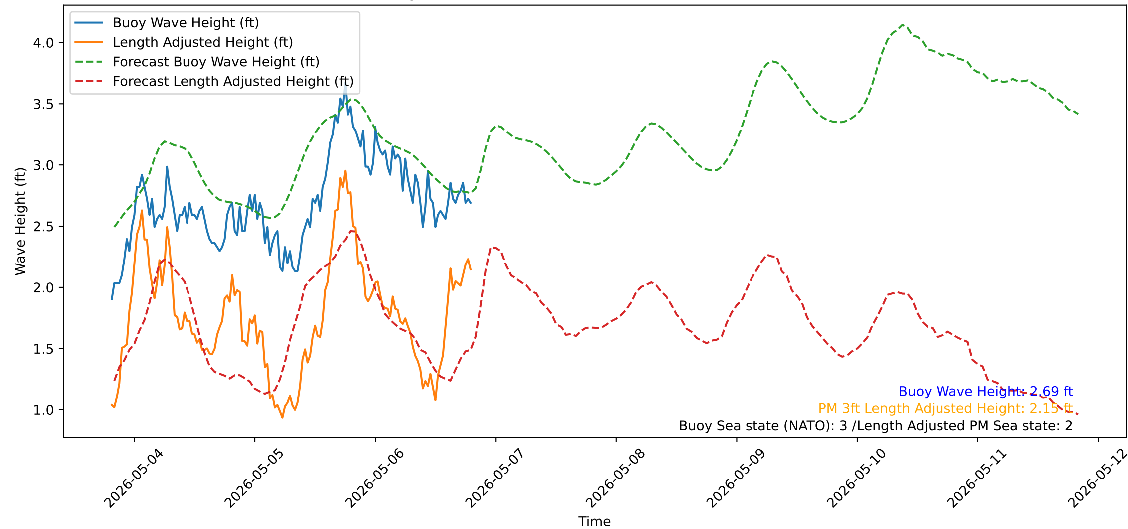
Wave Heights over Time for Green Beach at 2026-05-06 19:41:14
