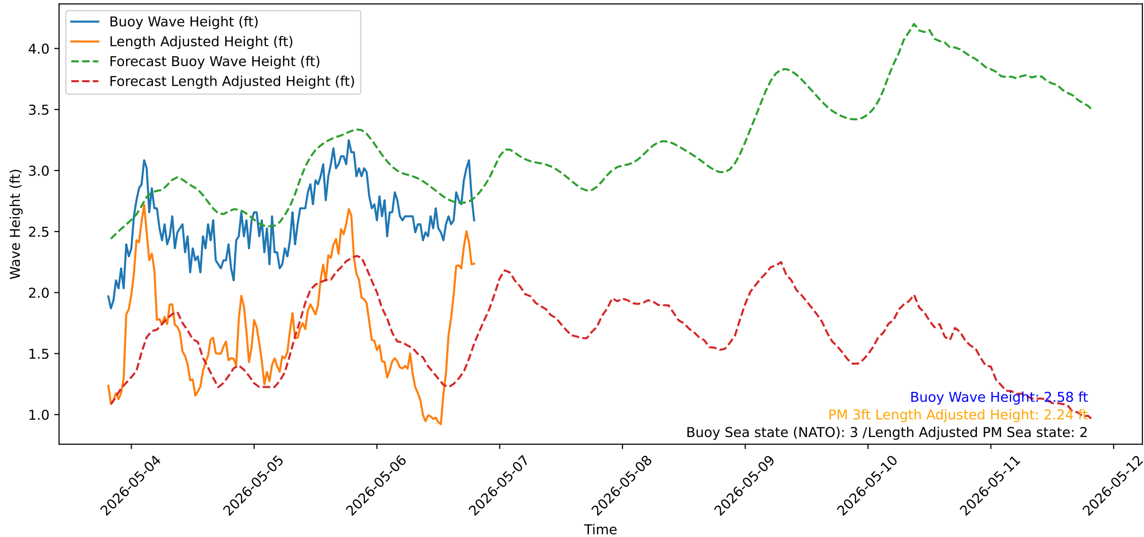
Wave Heights over Time for Oceanside Harbor at 2026-05-06 19:40:32
