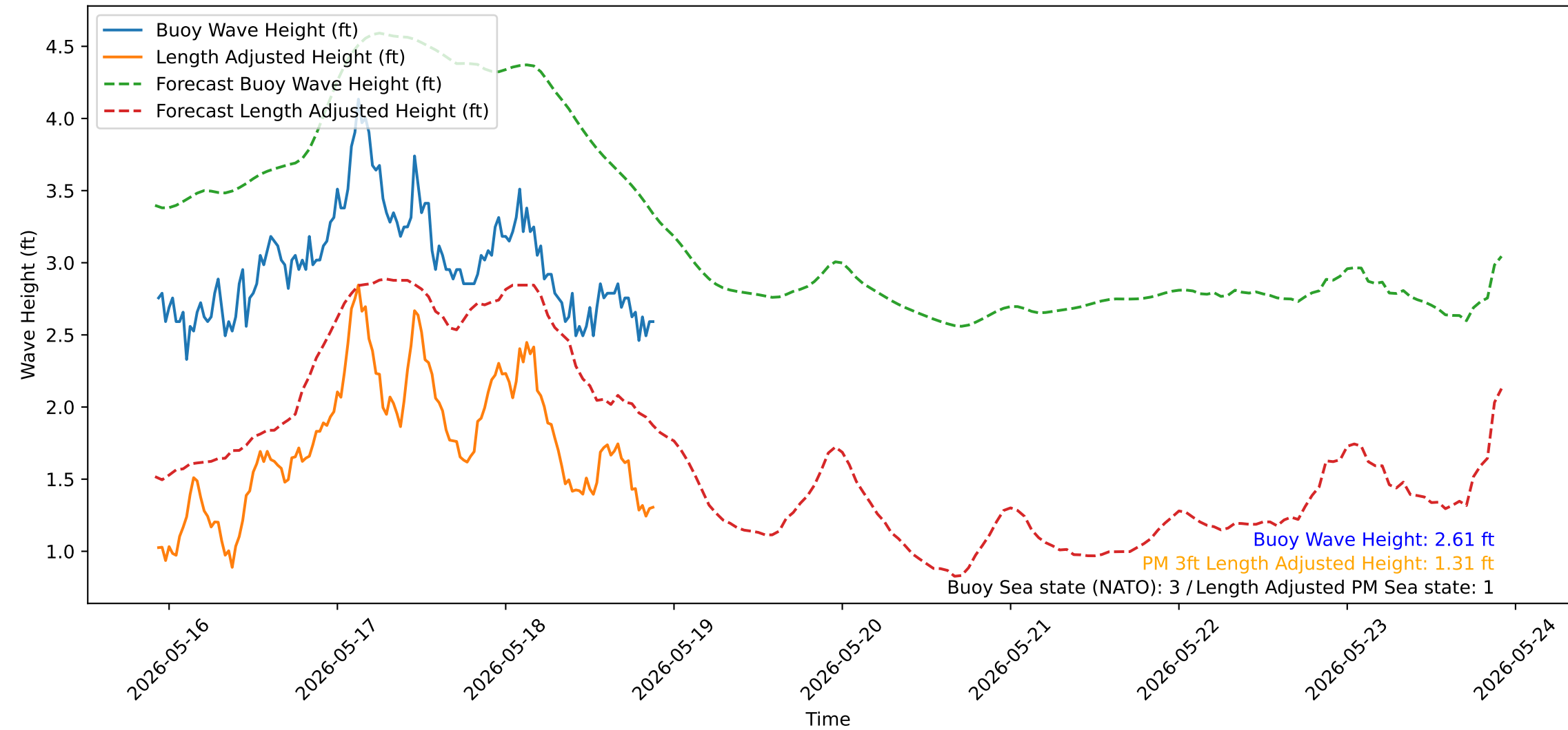
Wave Heights over Time for Red Beach at 2026-05-18 22:00:51
