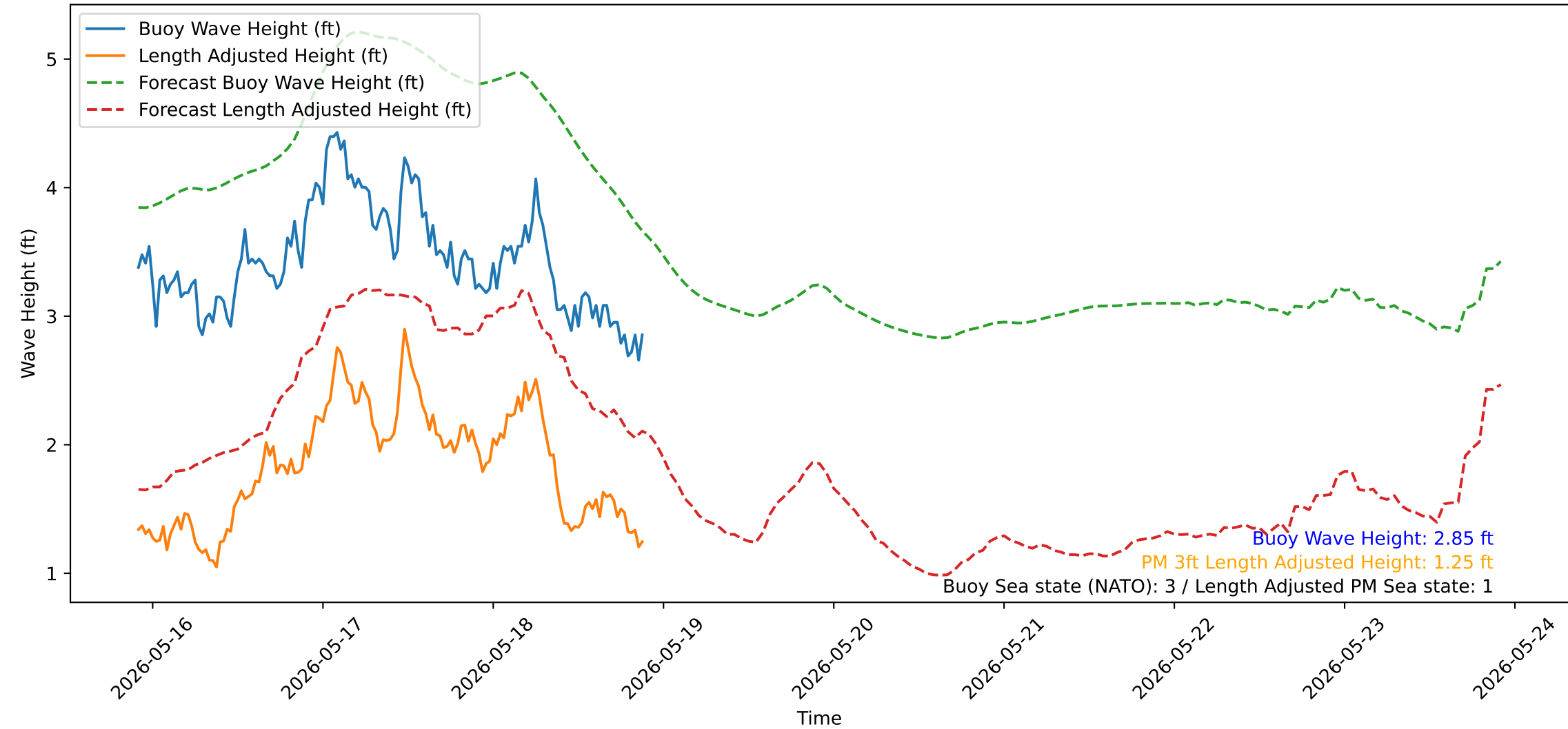
Wave Heights over Time for Green Beach at 2026-05-18 22:01:14
