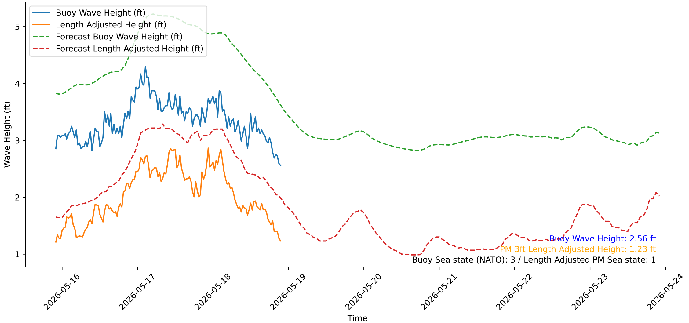
Wave Heights over Time for Oceanside Harbor at 2026-05-18 22:00:31
