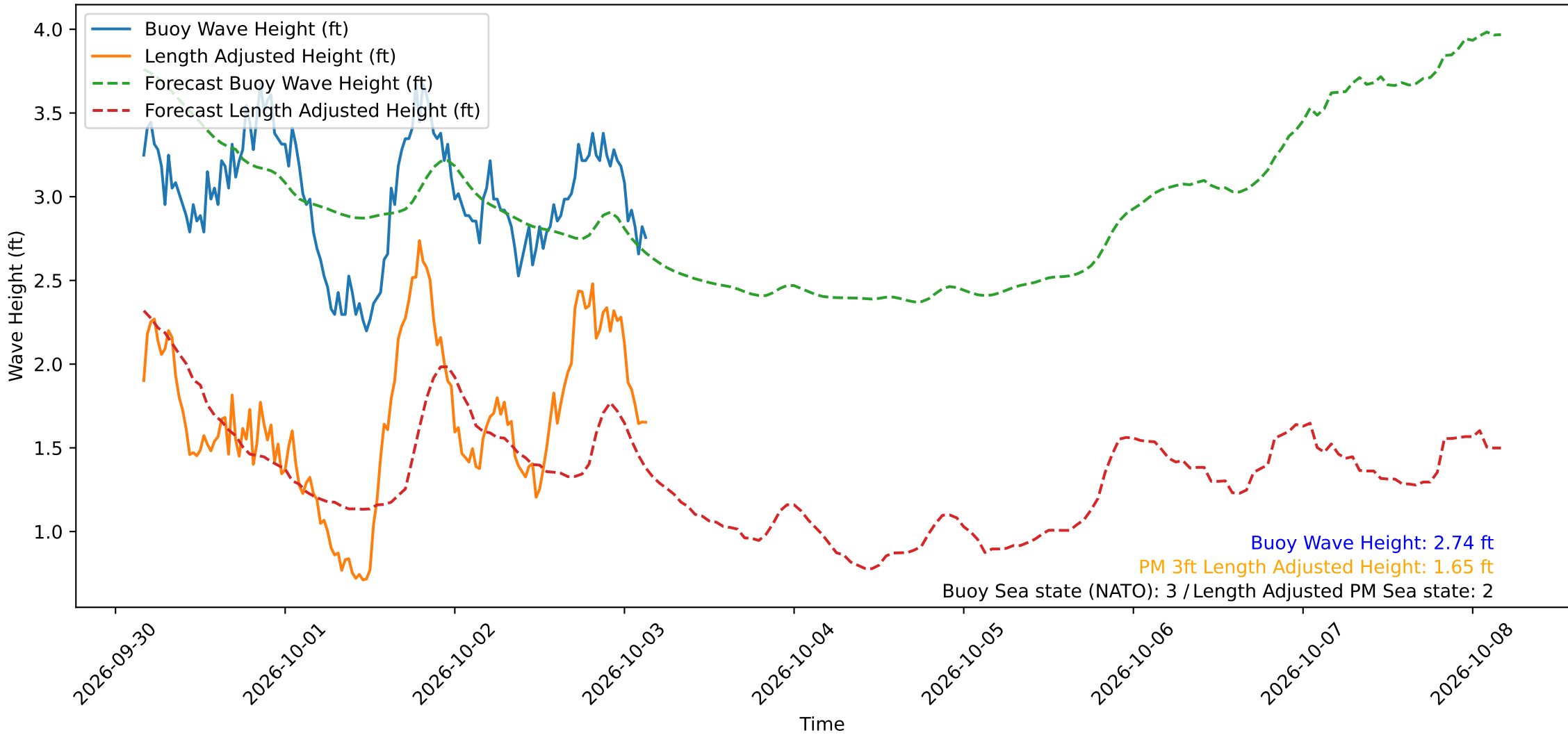
Wave Heights over Time for Green Beach at 2026-10-03 03:51:14
