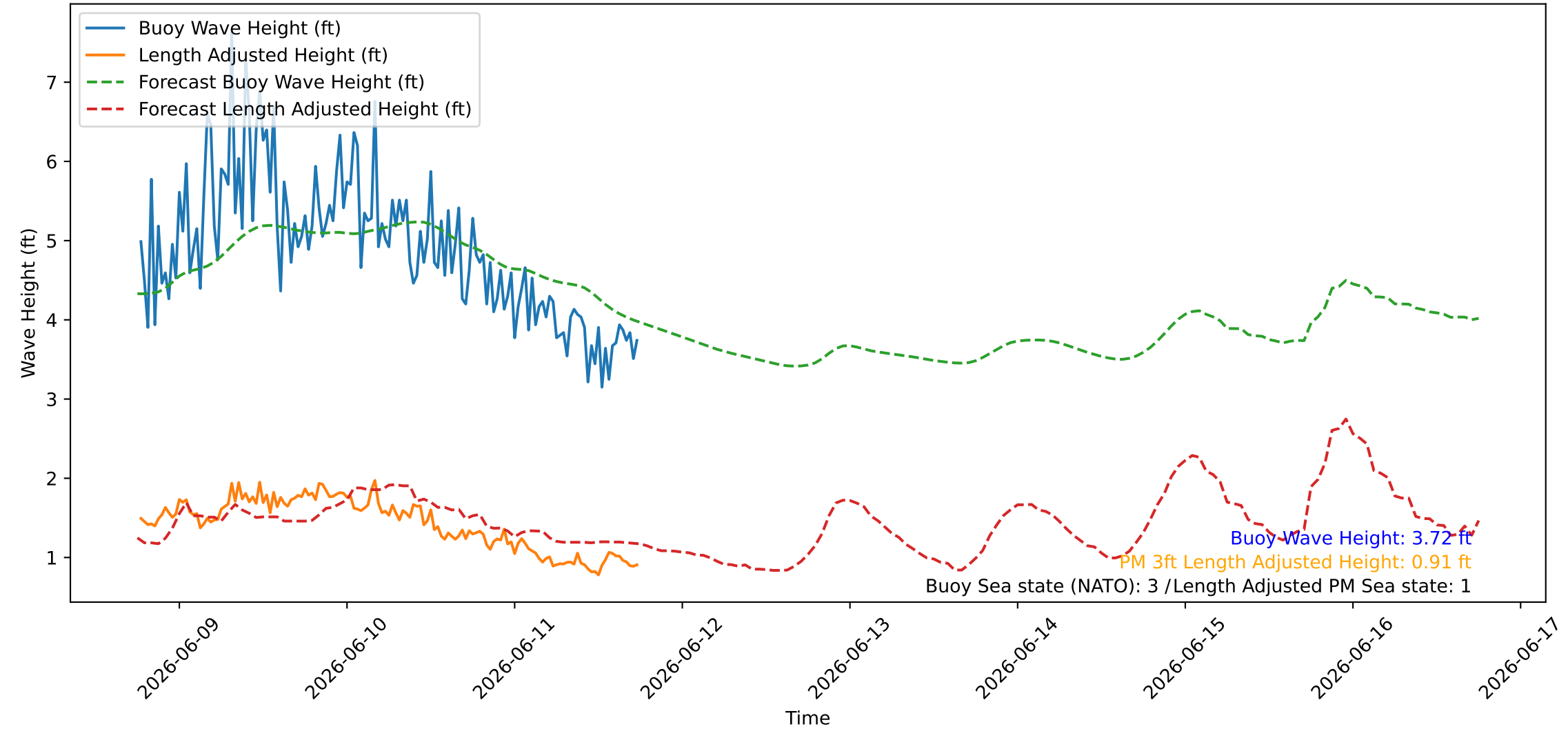
Wave Heights over Time for Red Beach at 2026-06-11 18:10:47
