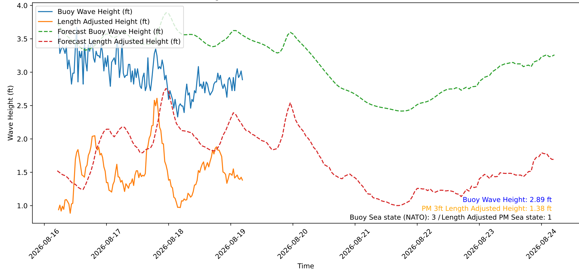
Wave Heights over Time for Red Beach at 2026-08-19 05:20:47
