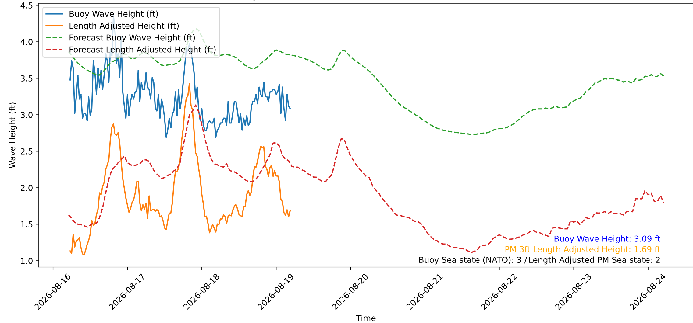
Wave Heights over Time for Green Beach at 2026-08-19 05:21:11
