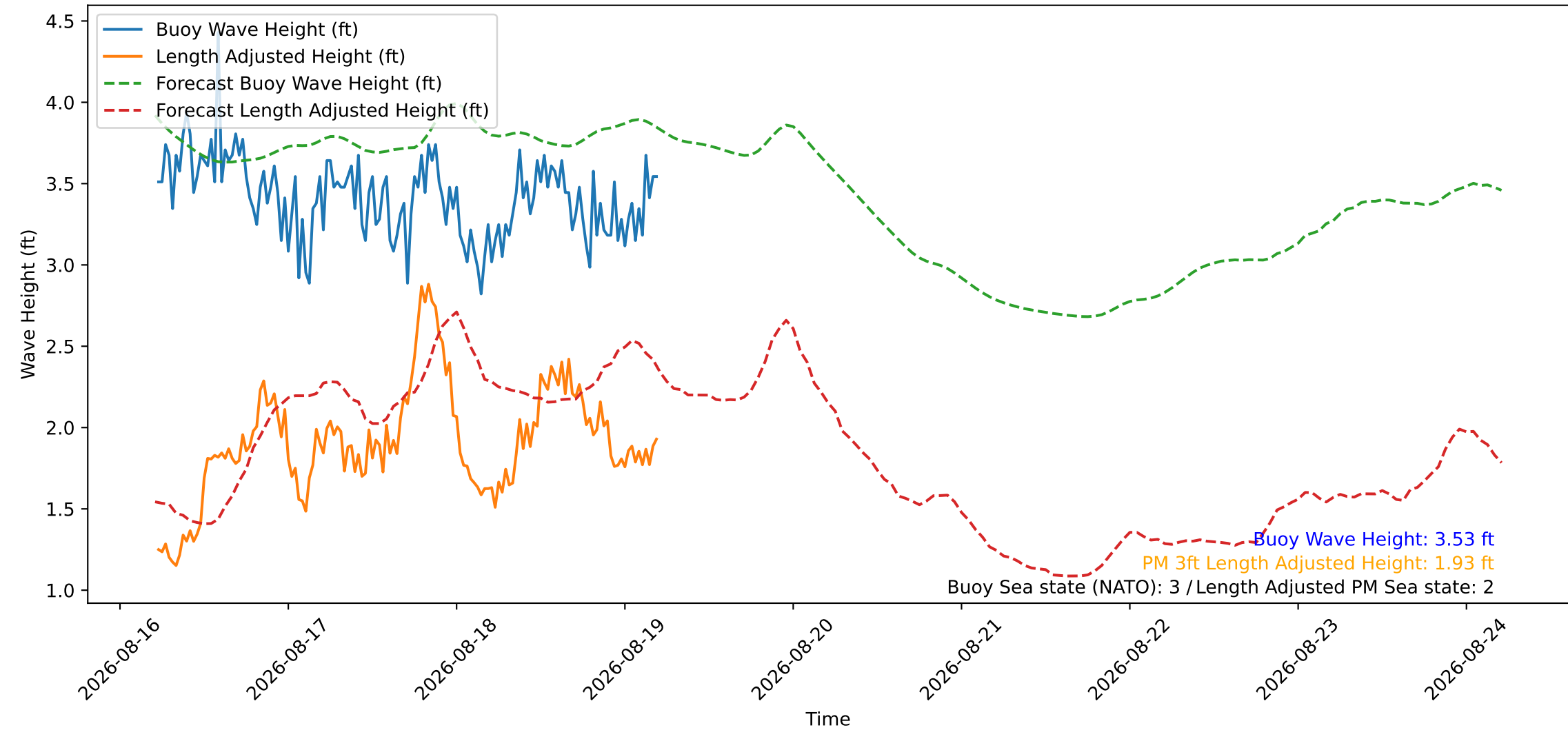
Wave Heights over Time for Oceanside Harbor at 2026-08-19 05:20:26
