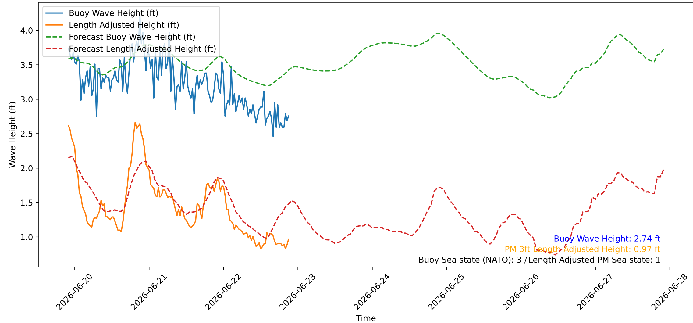
Wave Heights over Time for Green Beach at 2026-06-22 22:01:09
