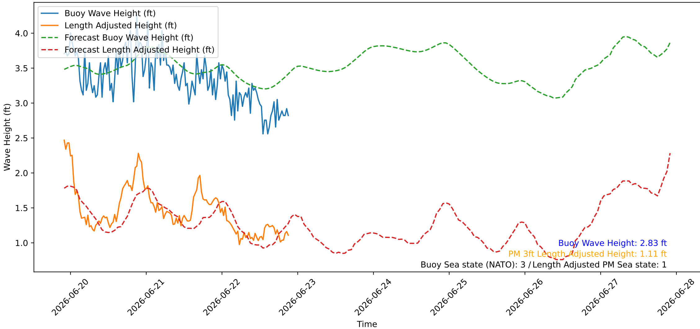
Wave Heights over Time for Oceanside Harbor at 2026-06-22 22:00:26
