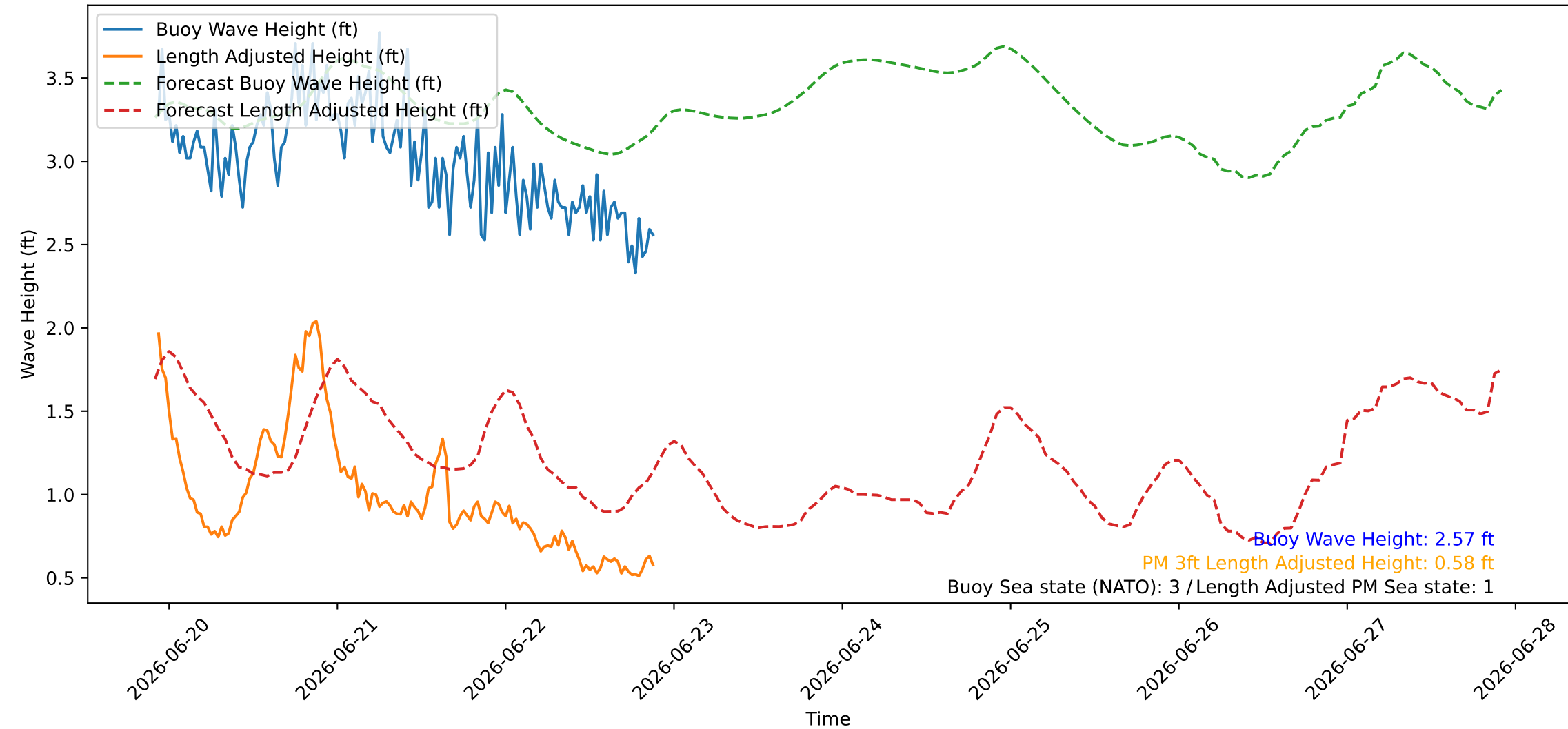
Wave Heights over Time for Red Beach at 2026-06-22 22:00:46
