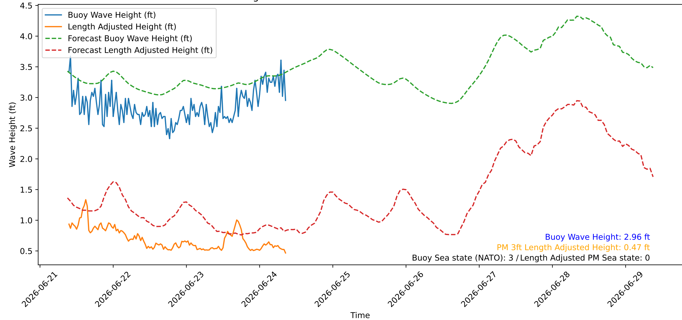
Wave Heights over Time for Red Beach at 2026-06-24 09:20:47
