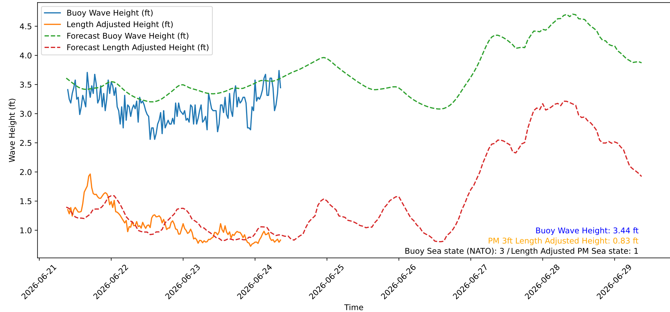
Wave Heights over Time for Oceanside Harbor at 2026-06-24 09:20:26
