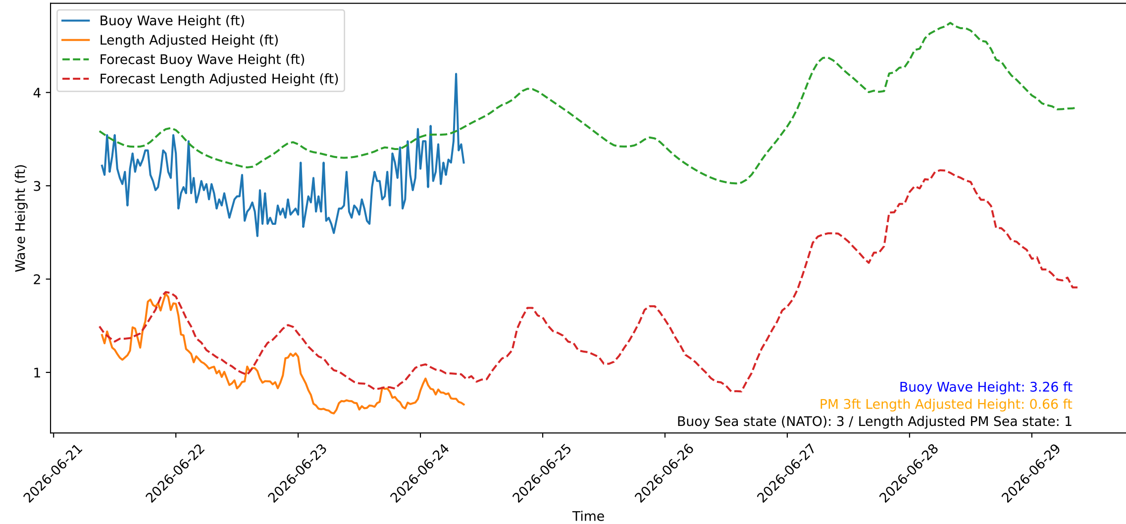
Wave Heights over Time for Green Beach at 2026-06-24 09:21:09
