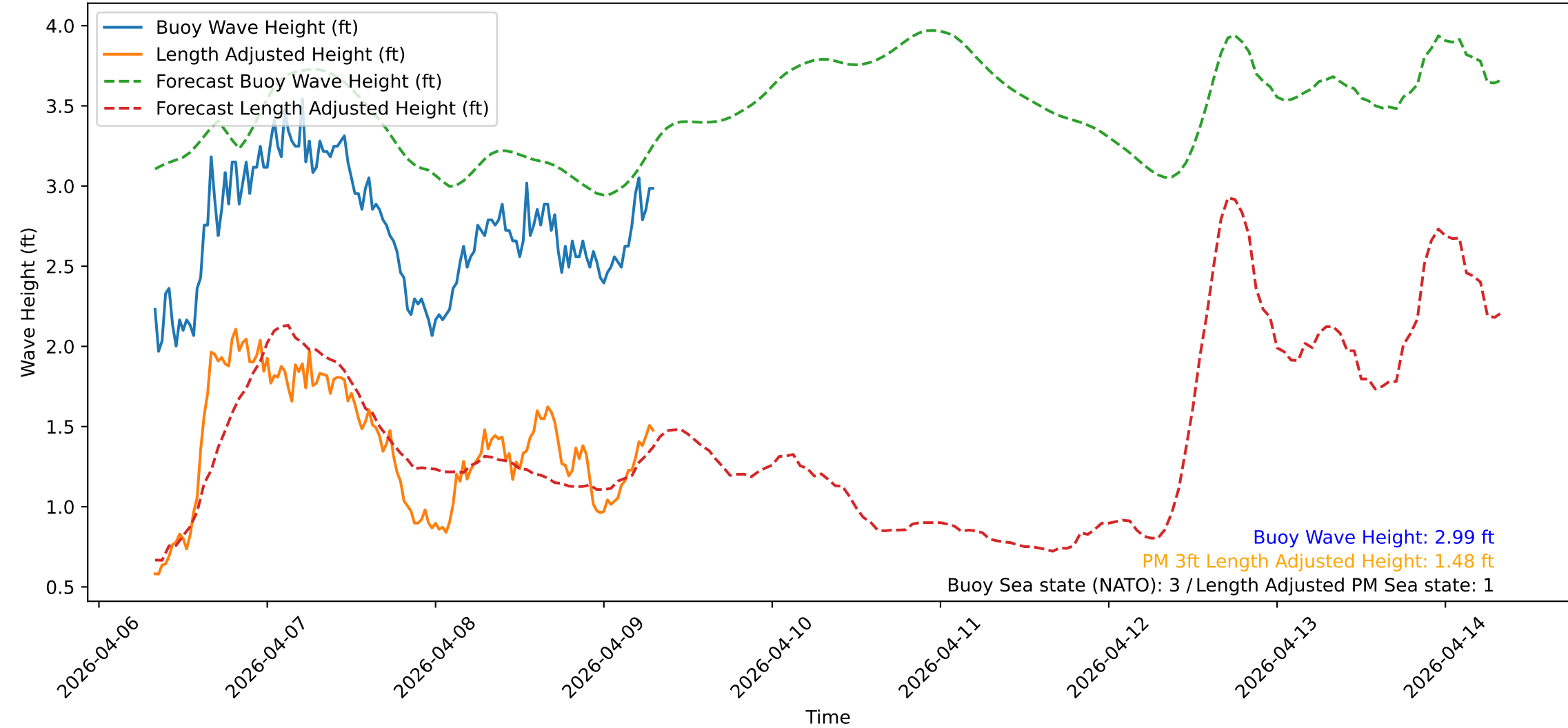
Wave Heights over Time for Red Beach at 2026-04-09 07:50:48
