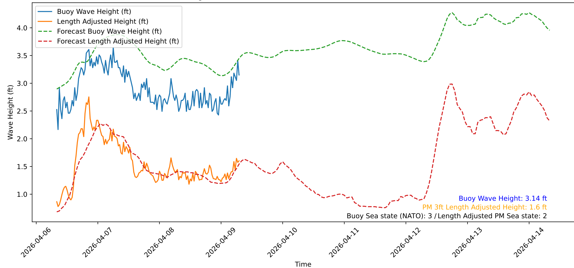
Wave Heights over Time for Oceanside Harbor at 2026-04-09 07:50:32
