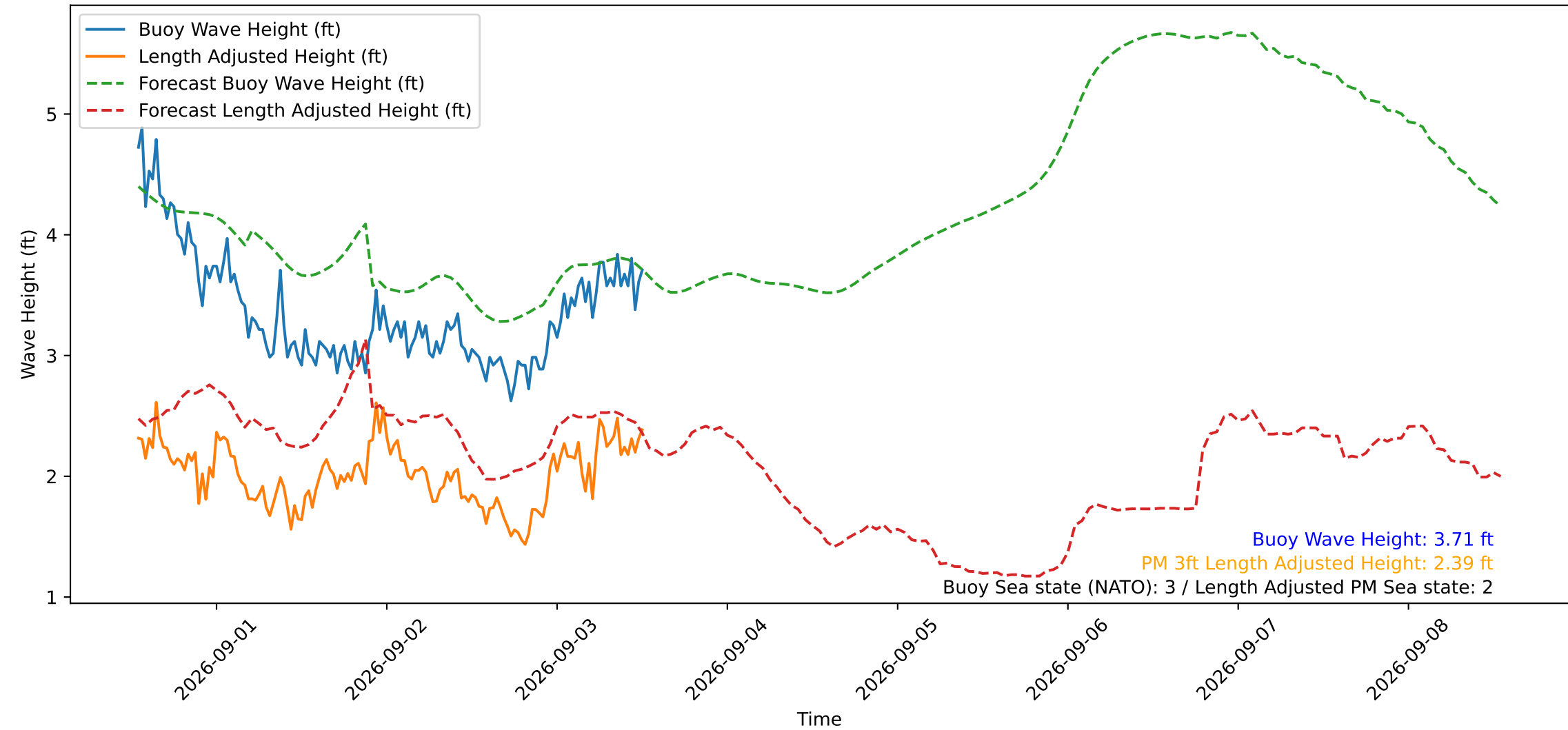
Wave Heights over Time for Oceanside Harbor at 2026-09-03 12:50:30
