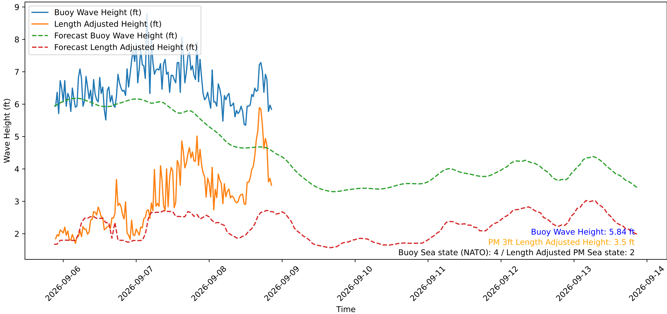
Wave Heights over Time for Green Beach at 2026-09-08 21:11:11
