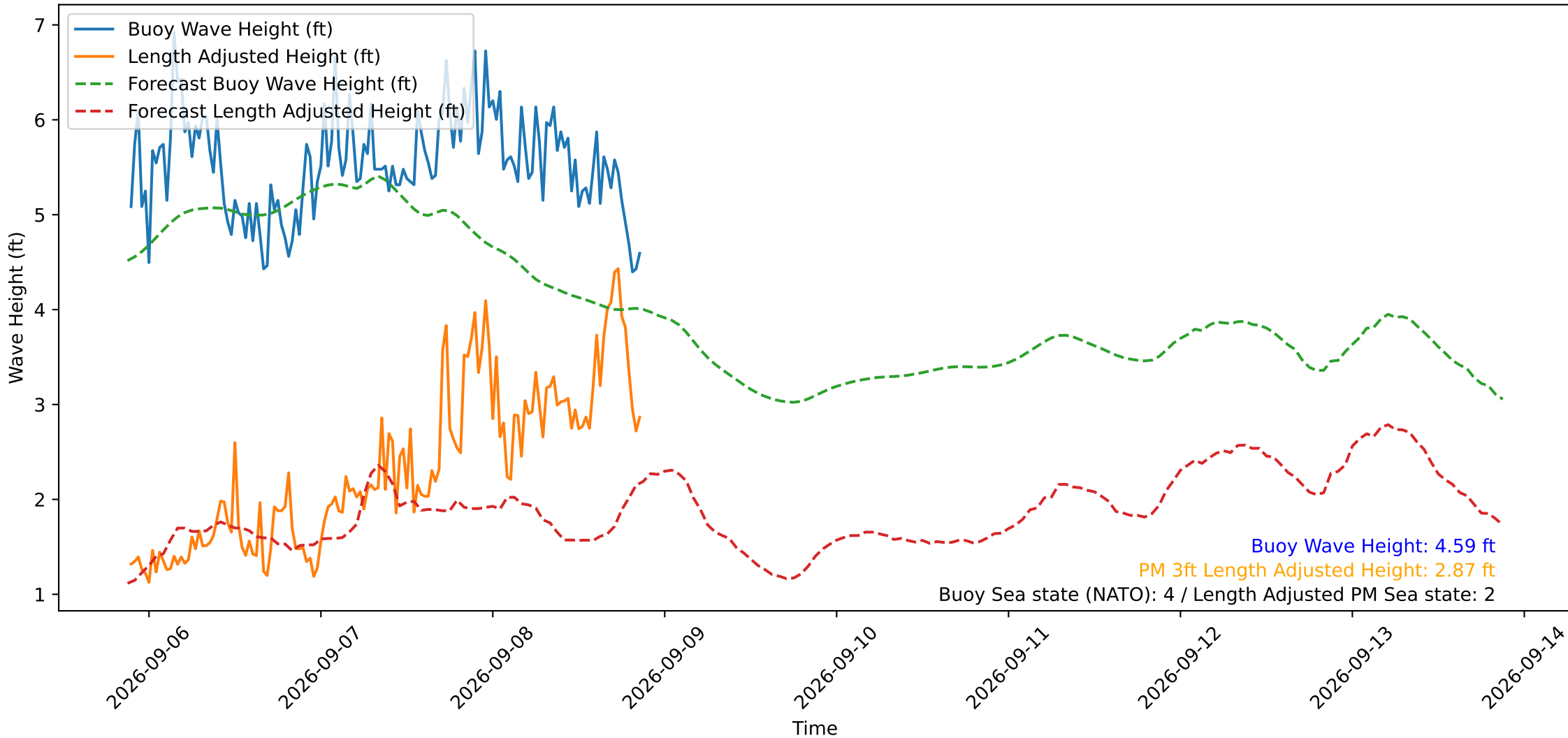
Wave Heights over Time for Red Beach at 2026-09-08 21:10:49
