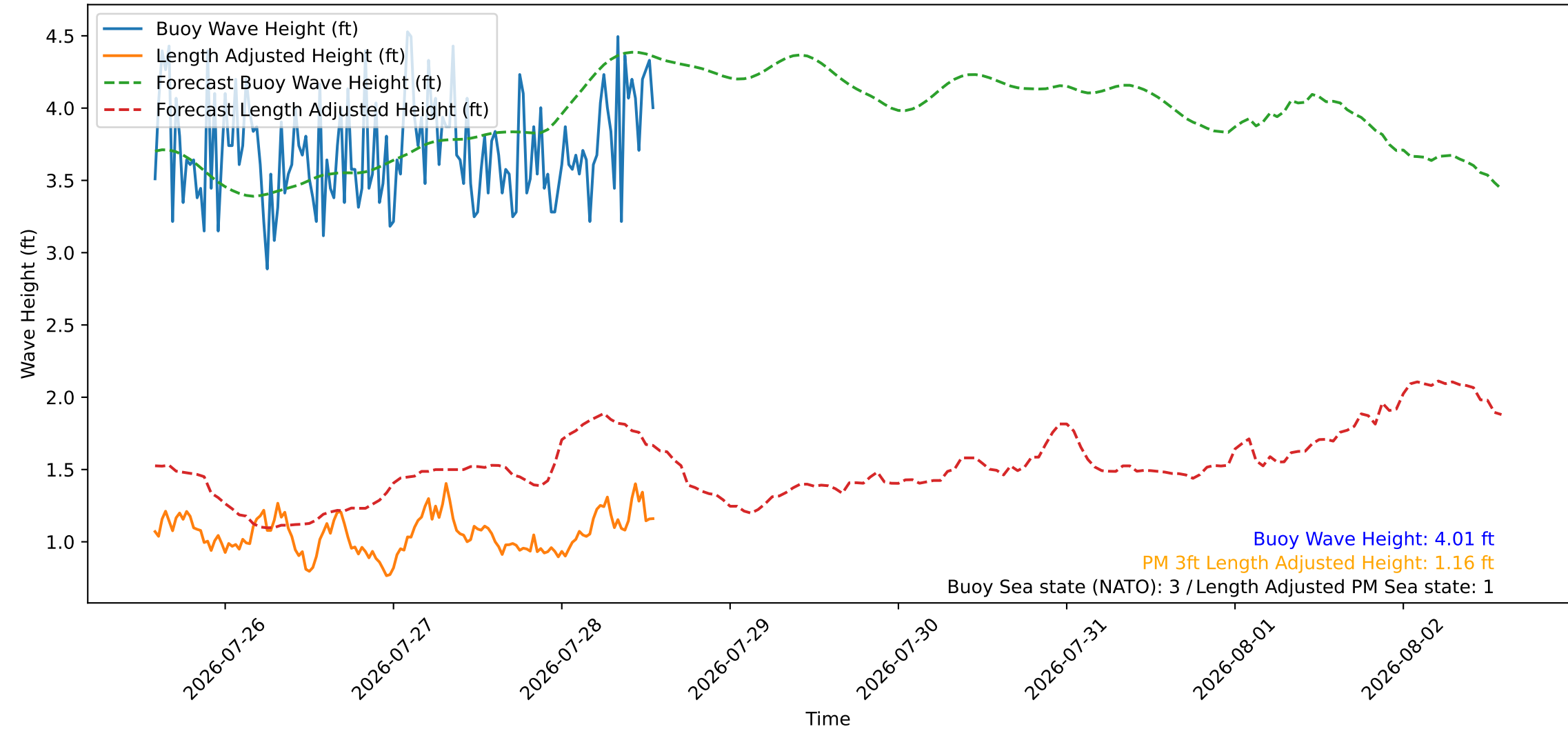
Wave Heights over Time for Red Beach at 2026-07-28 13:40:46
