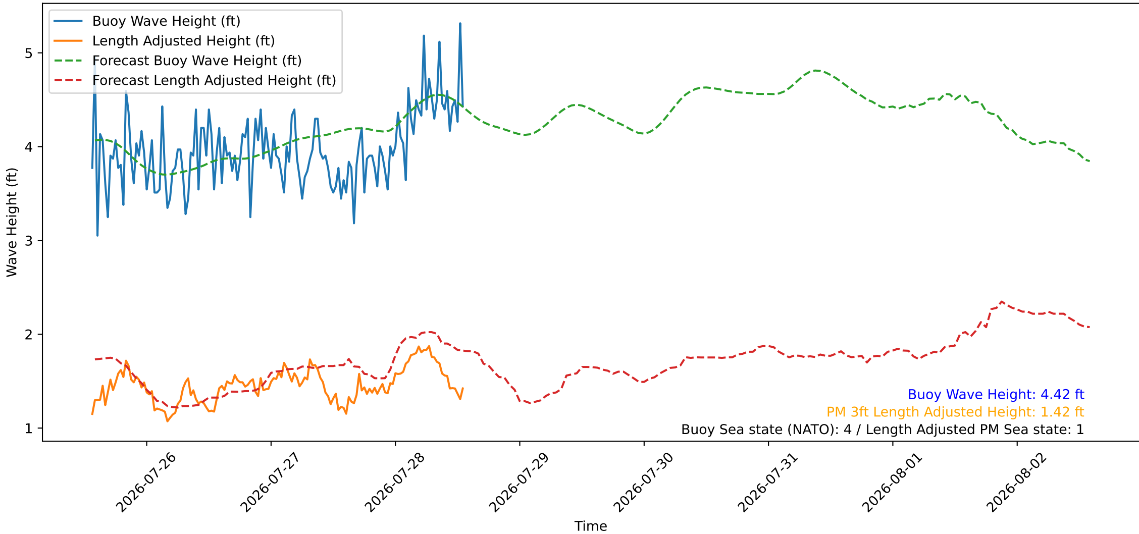
Wave Heights over Time for Oceanside Harbor at 2026-07-28 13:40:26
