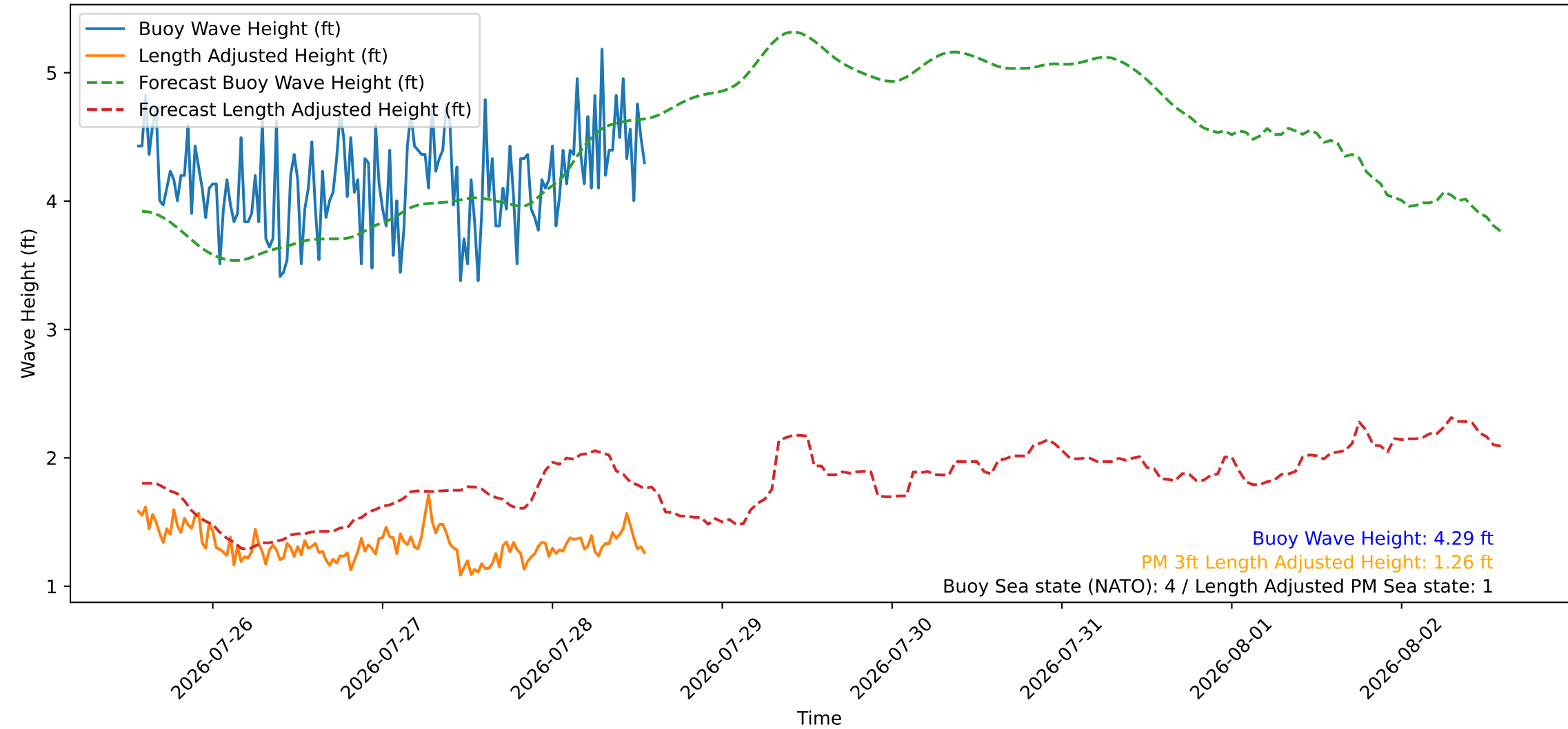
Wave Heights over Time for Green Beach at 2026-07-28 13:41:08
