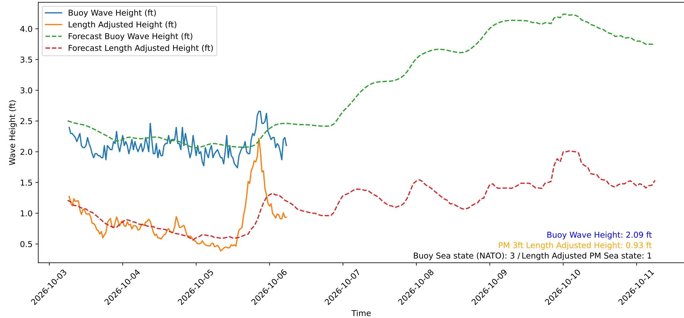
Wave Heights over Time for Red Beach at 2026-10-06 06:20:51
