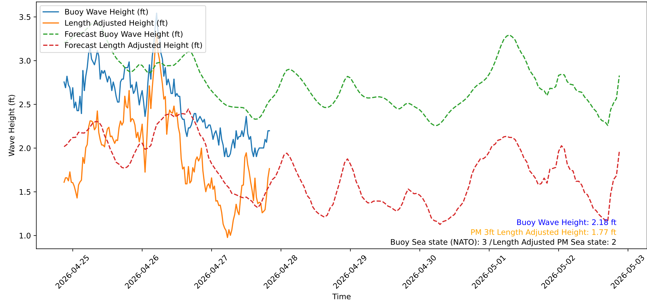
Wave Heights over Time for Red Beach at 2026-04-27 20:40:49
