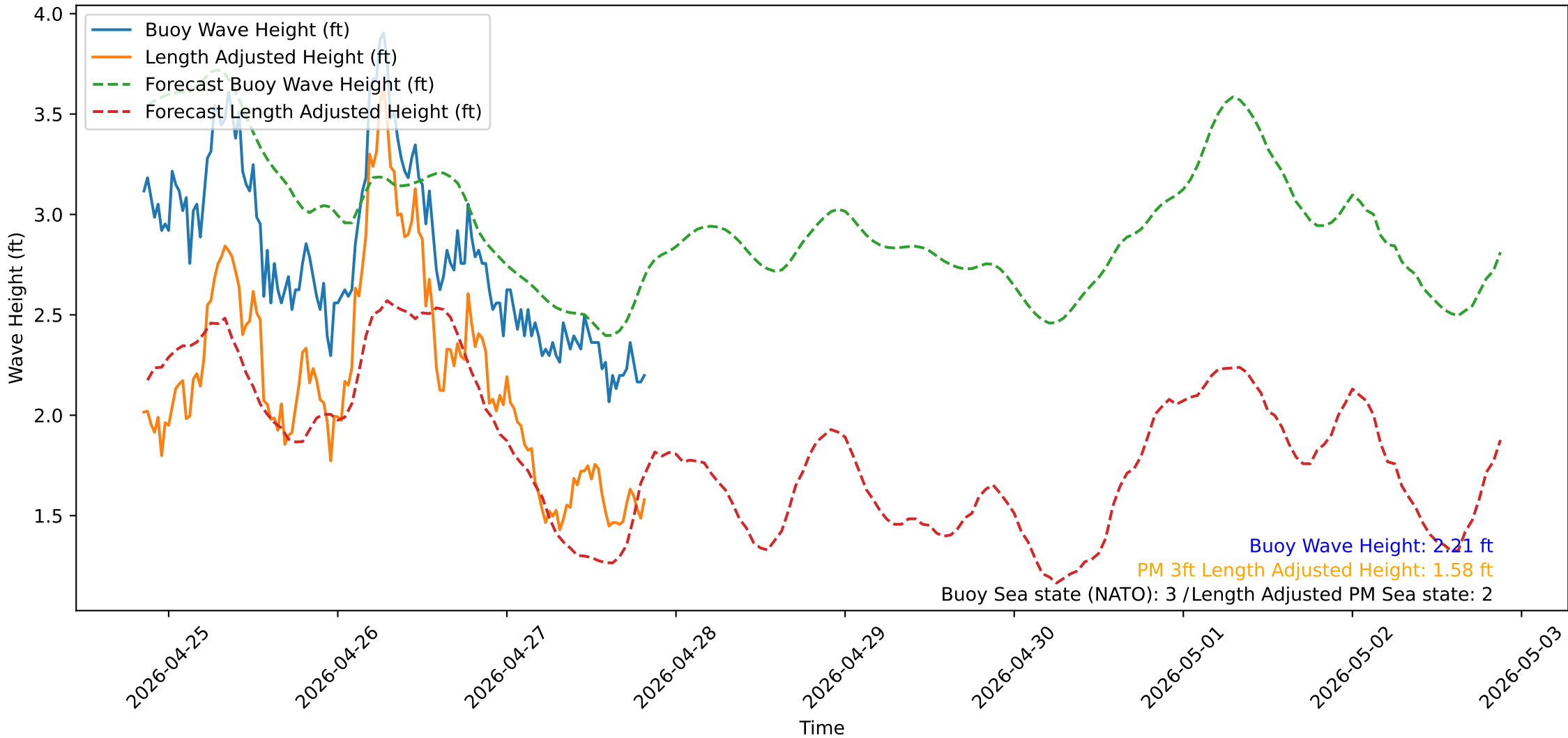
Wave Heights over Time for Oceanside Harbor at 2026-04-27 20:40:30
