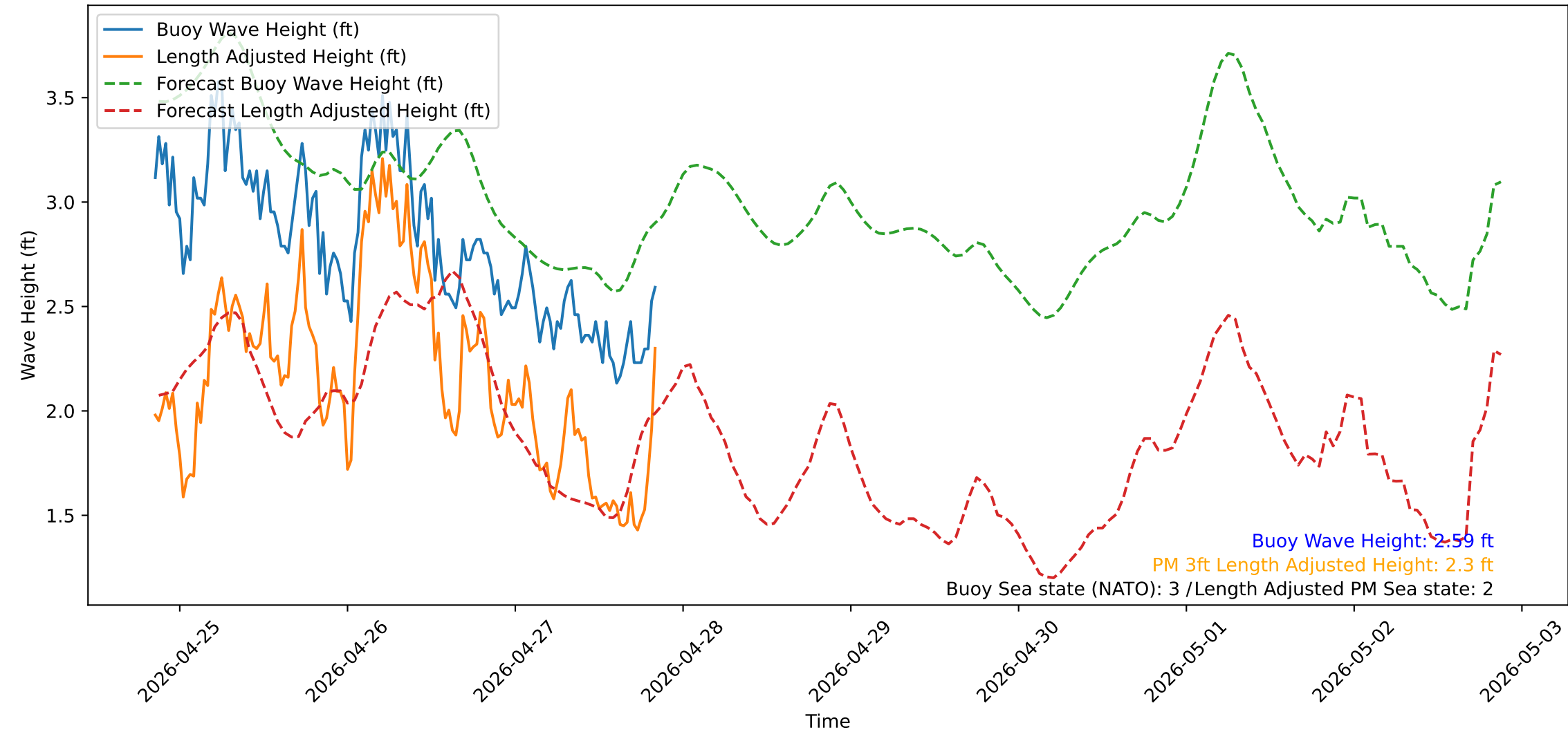
Wave Heights over Time for Green Beach at 2026-04-27 20:41:12
