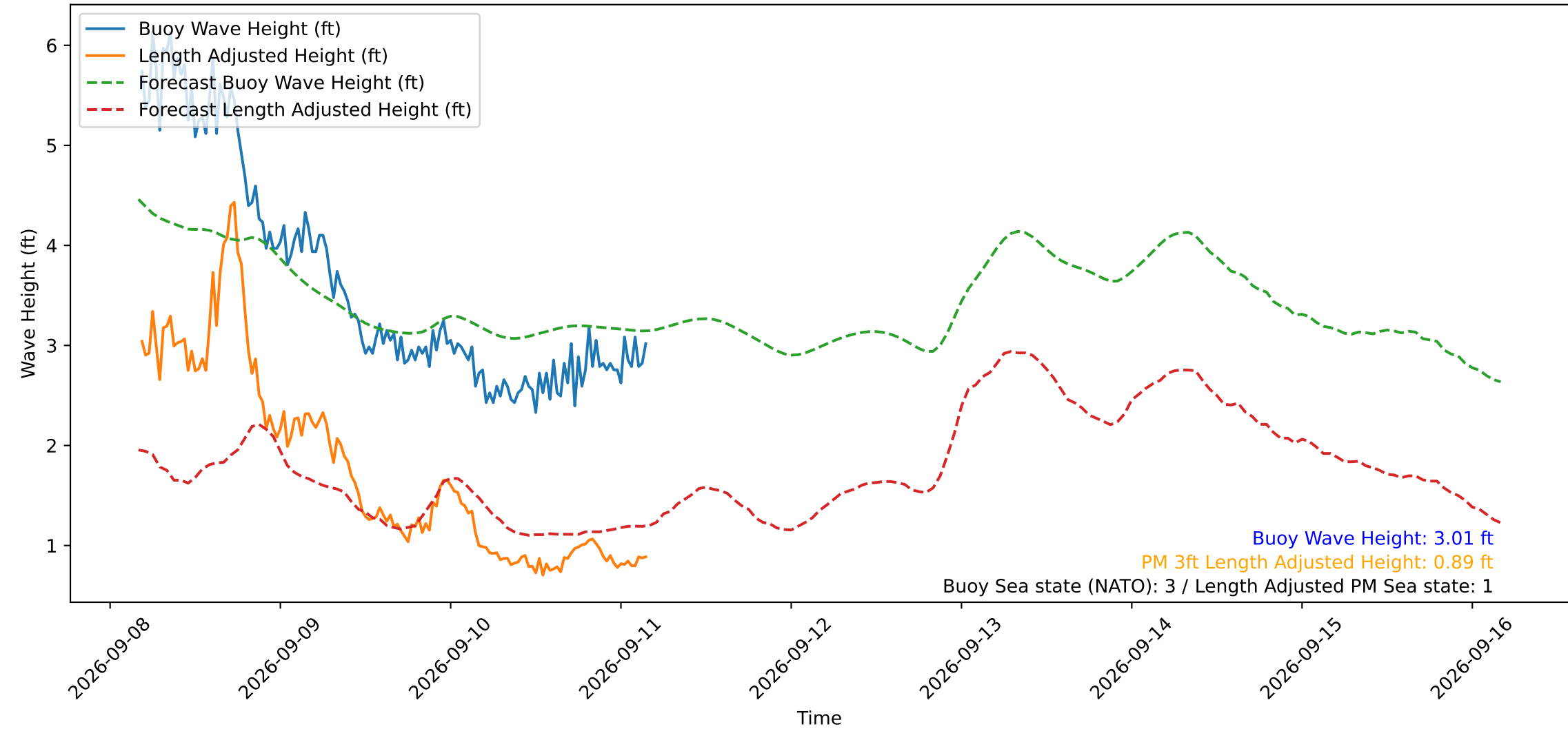
Wave Heights over Time for Red Beach at 2026-09-11 04:20:51
