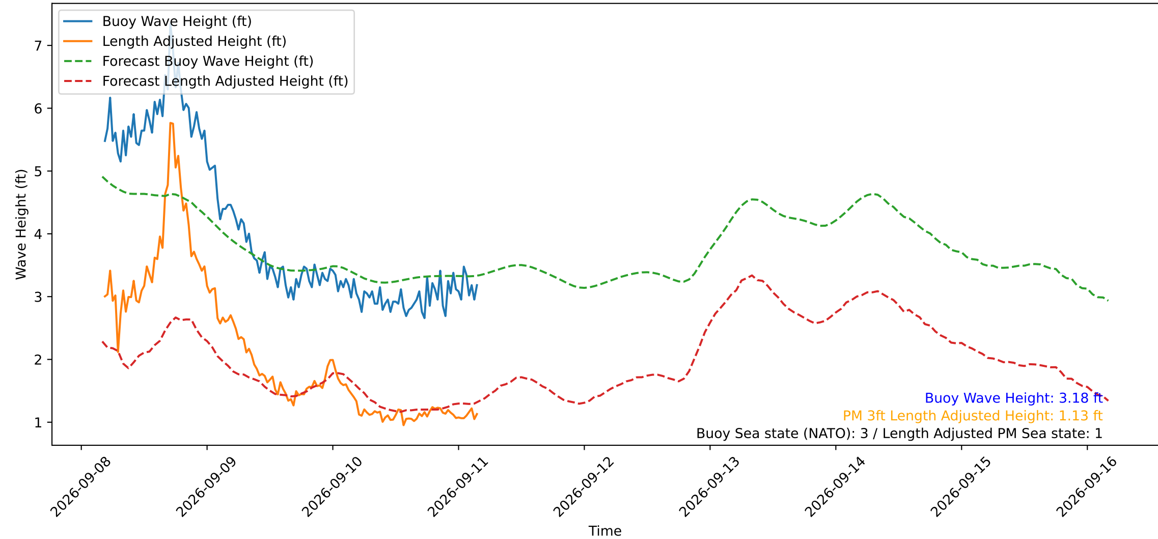
Wave Heights over Time for Oceanside Harbor at 2026-09-11 04:20:29
