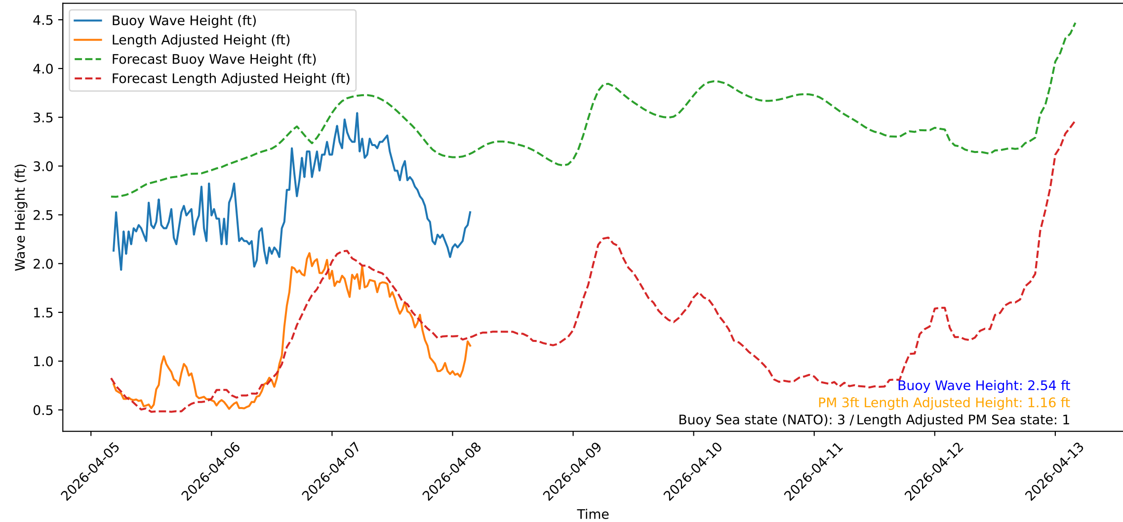
Wave Heights over Time for Red Beach at 2026-04-08 04:20:47
